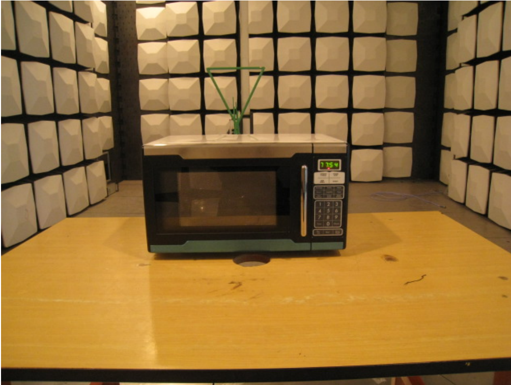
Photo 8 Radiated Disturbance Test (above 1GHz) (MEW622-A)
