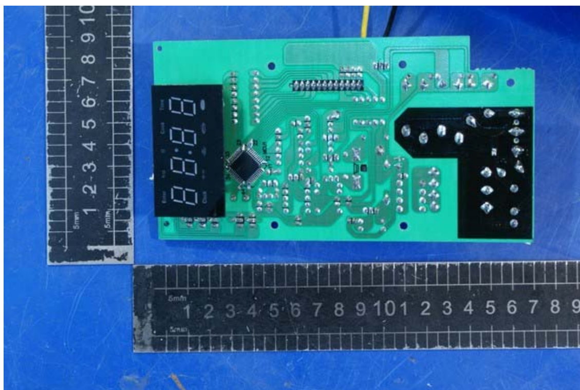
Photo 6 Internal photo of EUT (MEW621-A)
