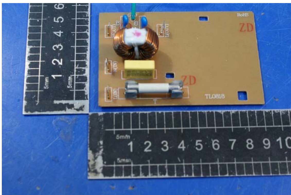
Photo 15 Internal photo of EUT (MEW622-A)
