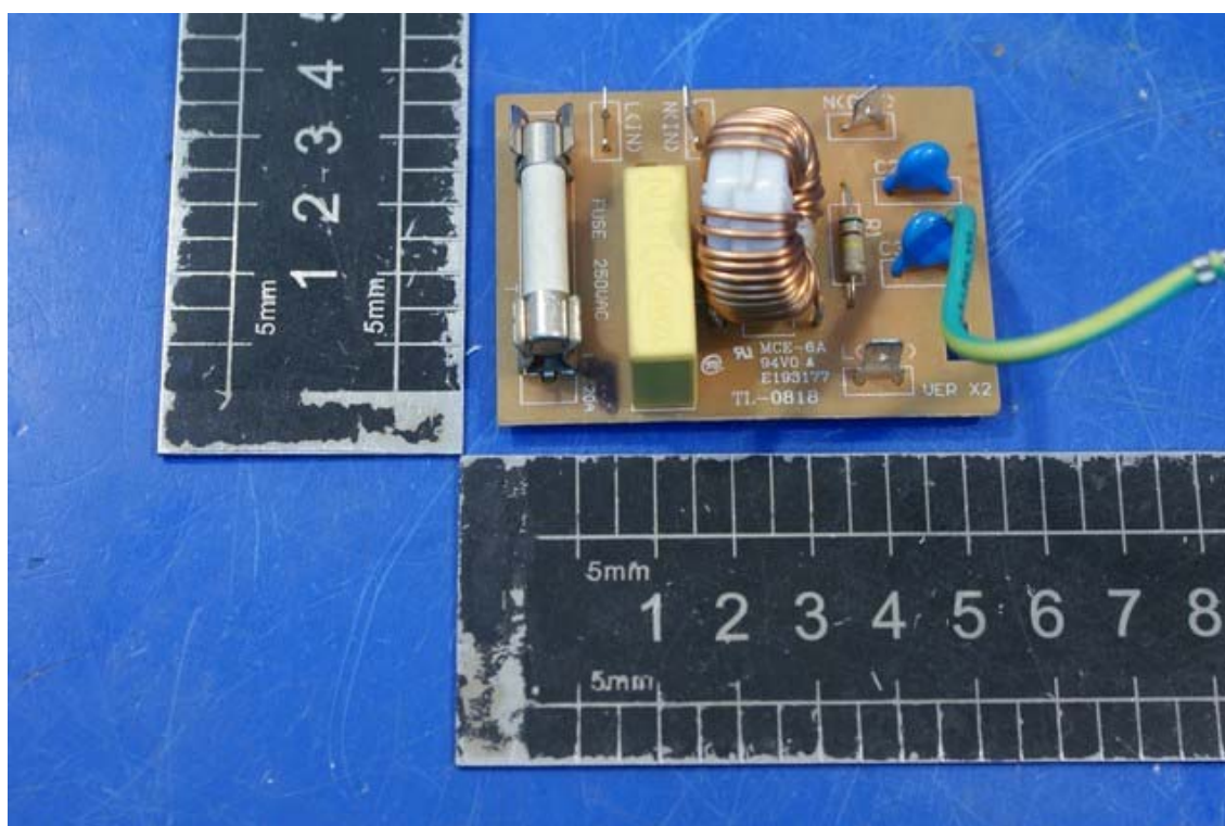
Photo 7 Internal photo of EUT (MEW621-A)
