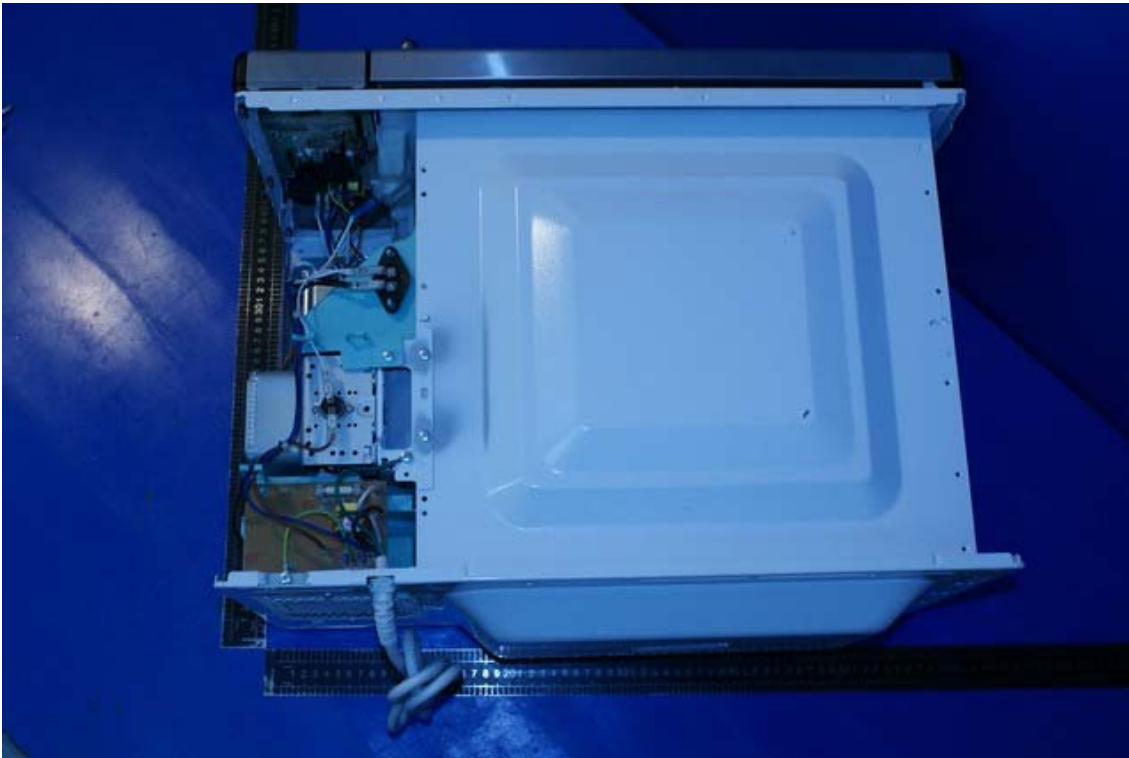
Photo 9 Internal photo of EUT (MEW622-A)
