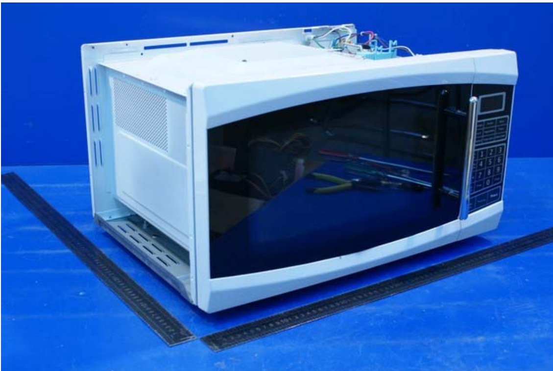
Photo 2 Internal photo of EUT (MEW621-A)
