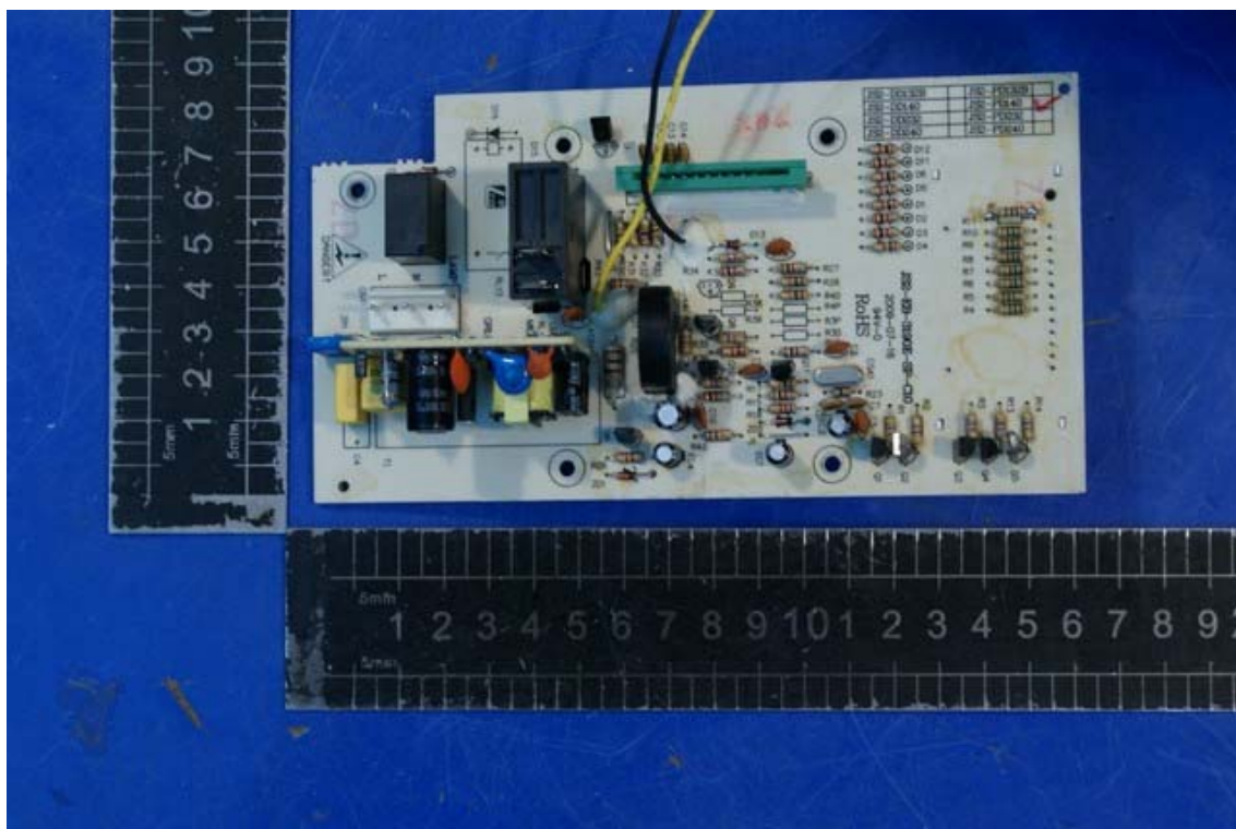
Photo 13 Internal photo of EUT (MEW622-A)
