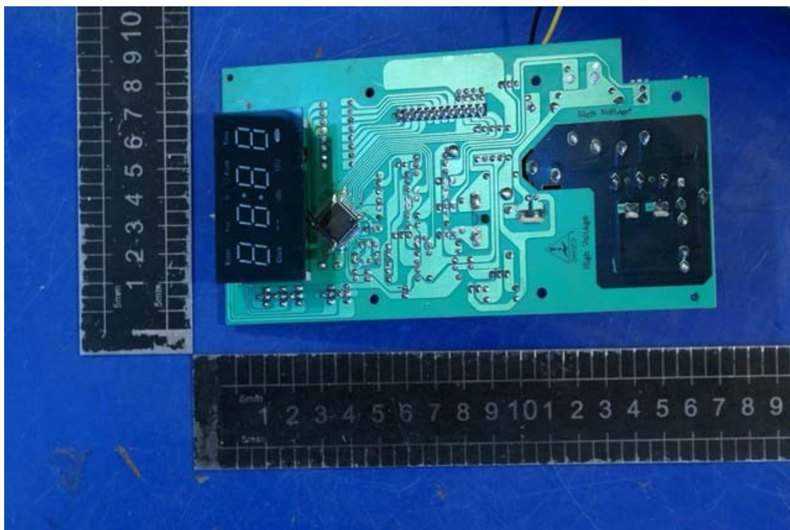
Photo 14 Internal photo of EUT (MEW622-A)
