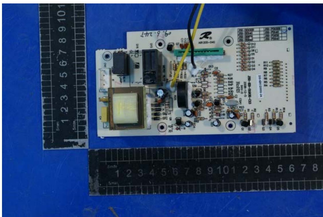
Photo 5 Internal photo of EUT (MEW621-A)
