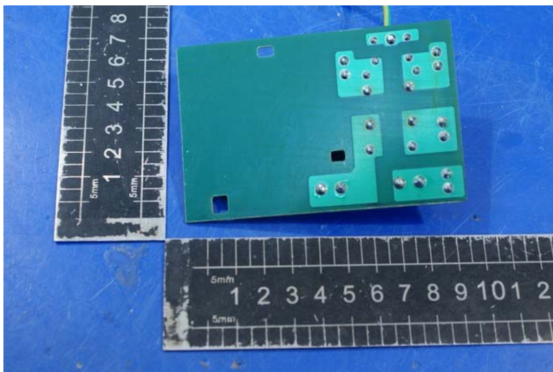
Photo 16 Internal photo of EUT (MEW622-A)
