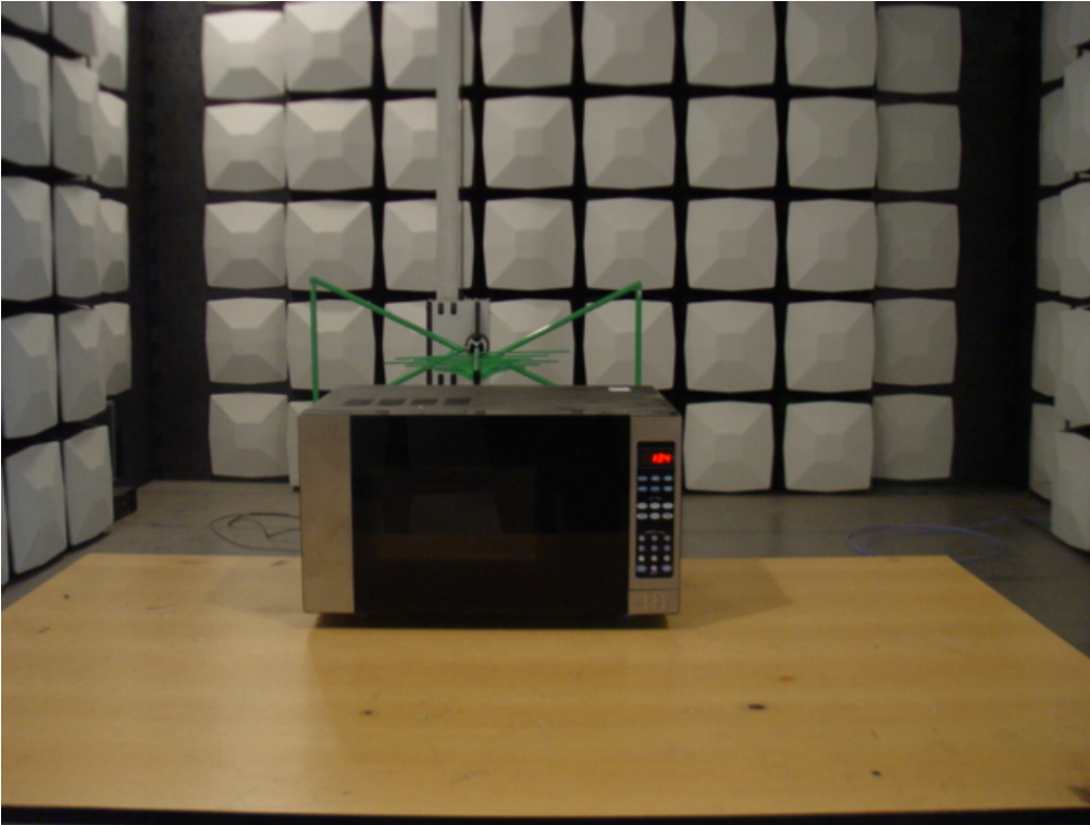
Photo 6 Radiated Disturbance Test (above 1GHz) (MEW60A-A)
