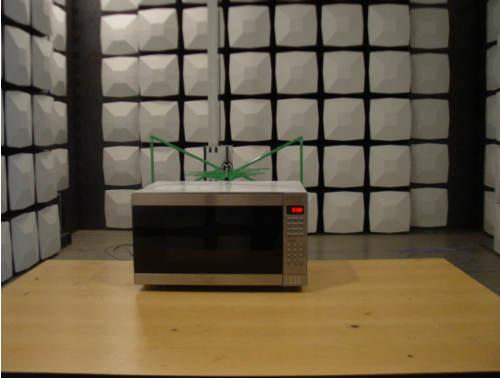
Photo 8 Radiated Disturbance Test (above 1GHz) (MEW60A-B)
