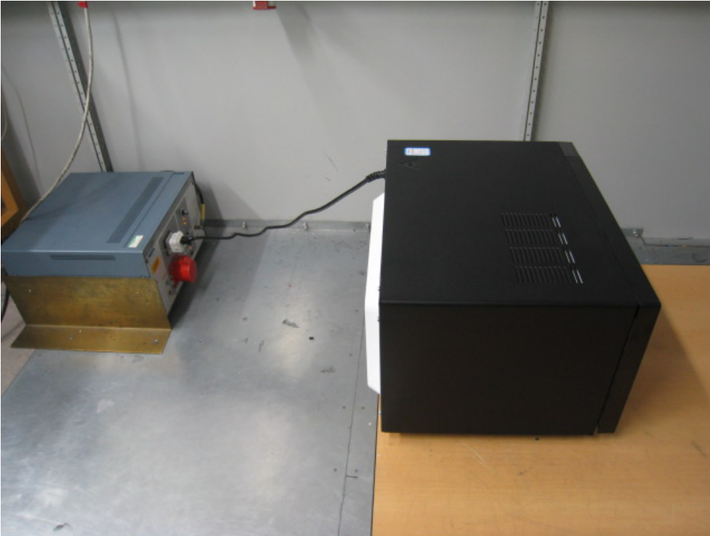
Photo 2 Conducted Disturbance Test (MEW60A-A)
