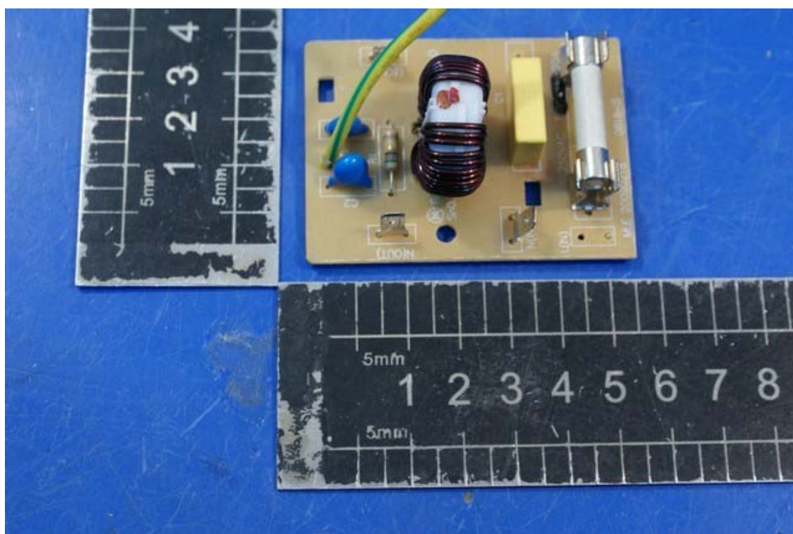
Photo 7 Internal photo of EUT (MEW60A-A)
