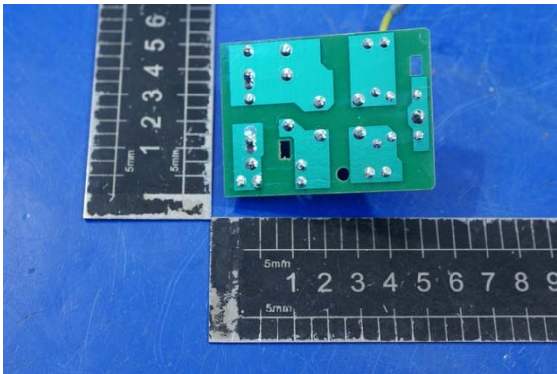
Photo 16 Internal photo of EUT (MEW60A-B)
