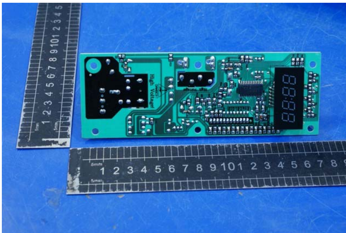
Photo 6 Internal photo of EUT (MEW60A-A)
