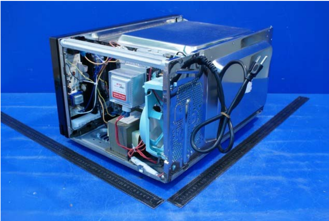
Photo 11 Internal photo of EUT (MEW60A-B)
