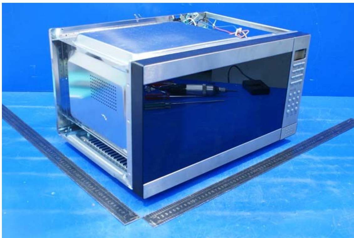
Photo 10 Internal photo of EUT (MEW60A-B)
