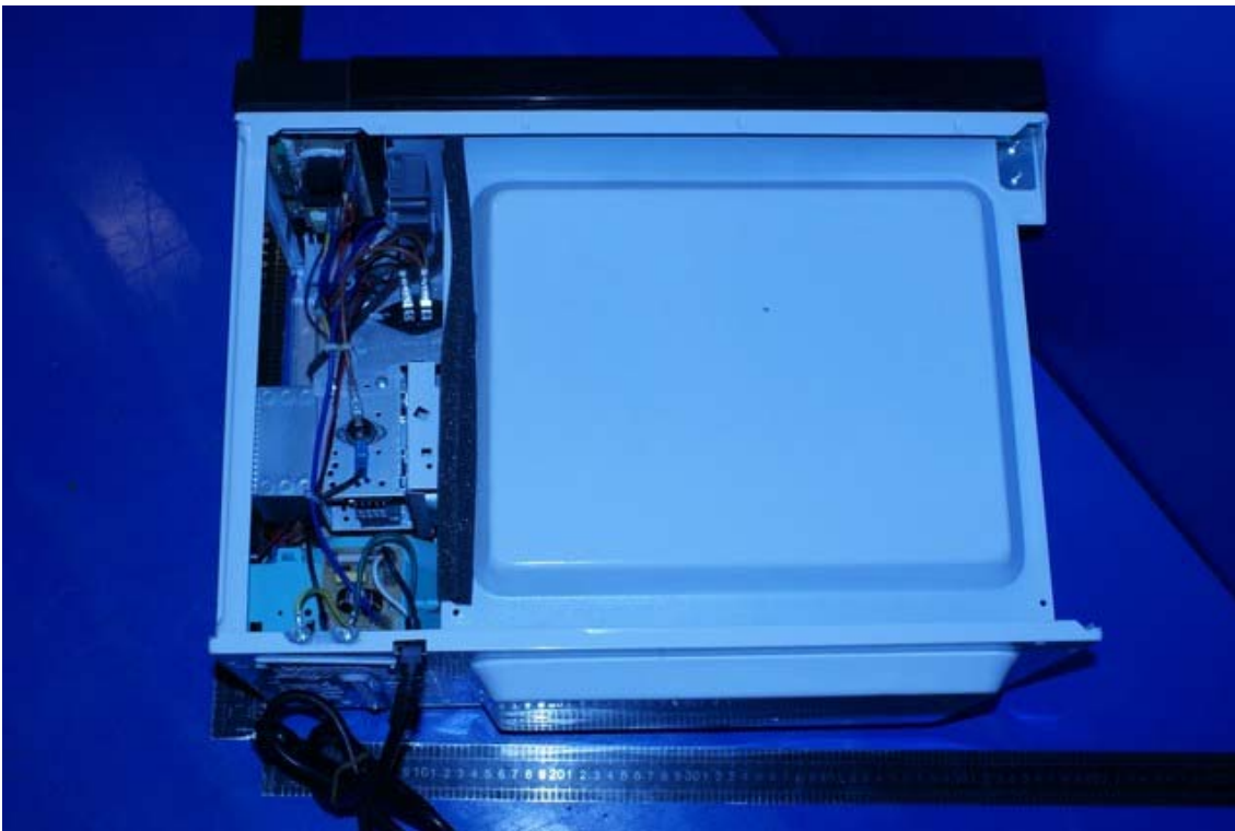
Photo 1 Internal photo of EUT (MEW60A-A)
