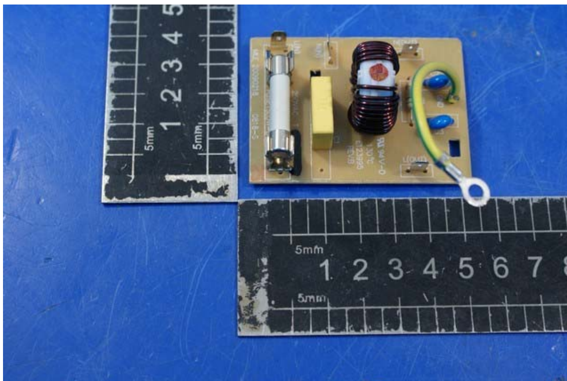
Photo 15 Internal photo of EUT (MEW60A-B)
