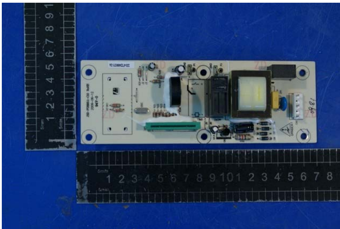
Photo 5 Internal photo of EUT (MEW60A-A)
