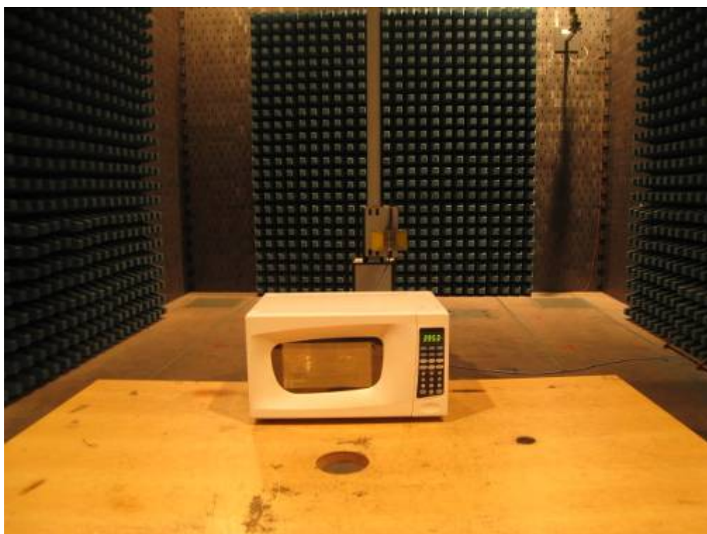
Photo 12 Radiated Disturbance Test (above 1GHz) (MEW50N-A)
