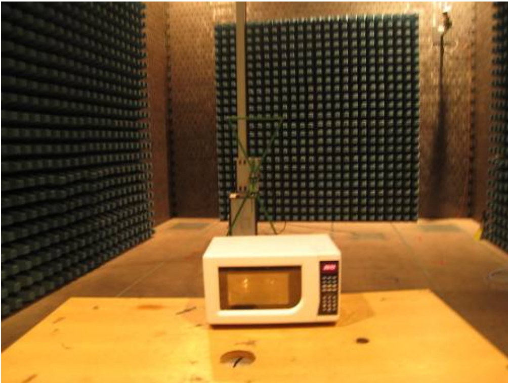
Photo 18 Radiated Disturbance Test (above 1GHz) (MEW50D-A)
