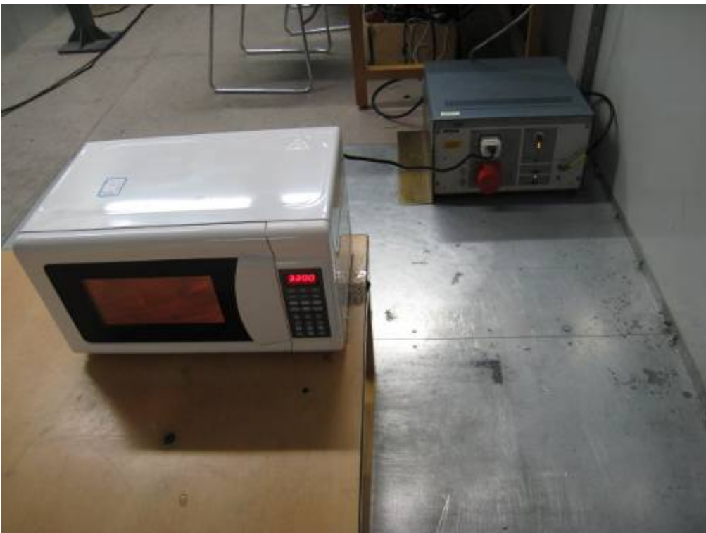
Photo 6 Conducted Disturbance Test (MEW50B-A)
