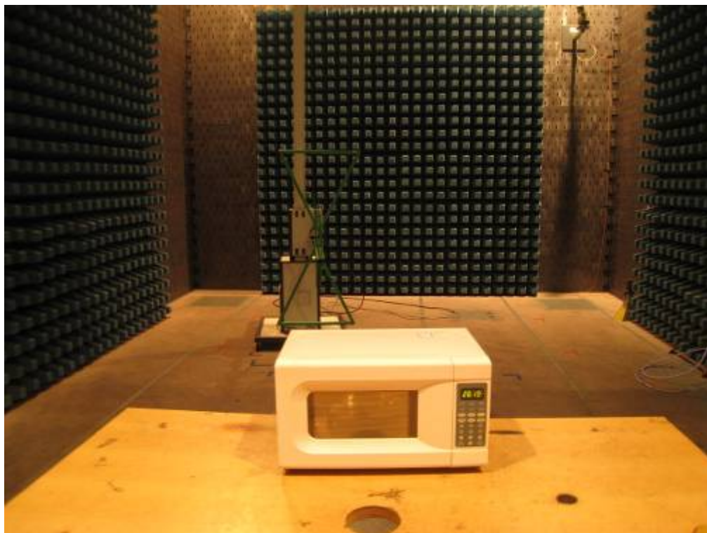
Photo 14 Radiated Disturbance Test (above 1GHz) (MEW50S-A)
