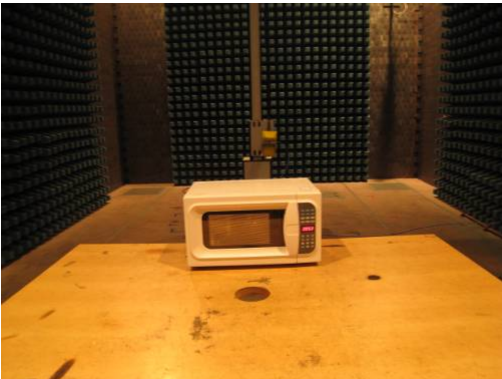
Photo 20 Radiated Disturbance Test (above 1GHz) (MEW50M-A)
