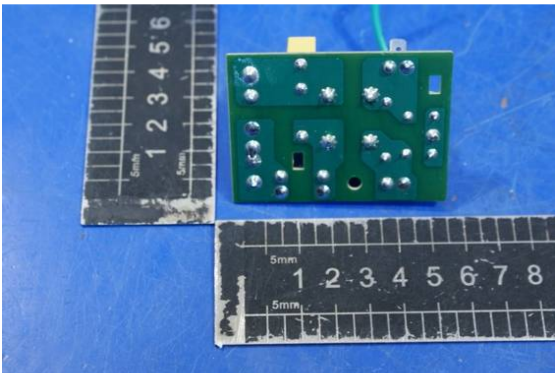
Photo 24 Internal photo of EUT (MEW50B-A)
