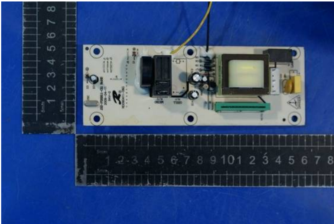
Photo 5 Internal photo of EUT (MEW50N-A)
