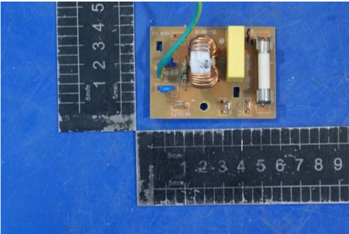
Photo 15 Internal photo of EUT (MEW50S-A)
