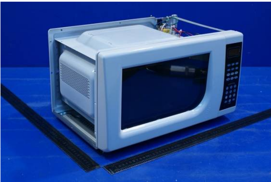
Photo 26 Internal photo of EUT (MEW50D-A)
