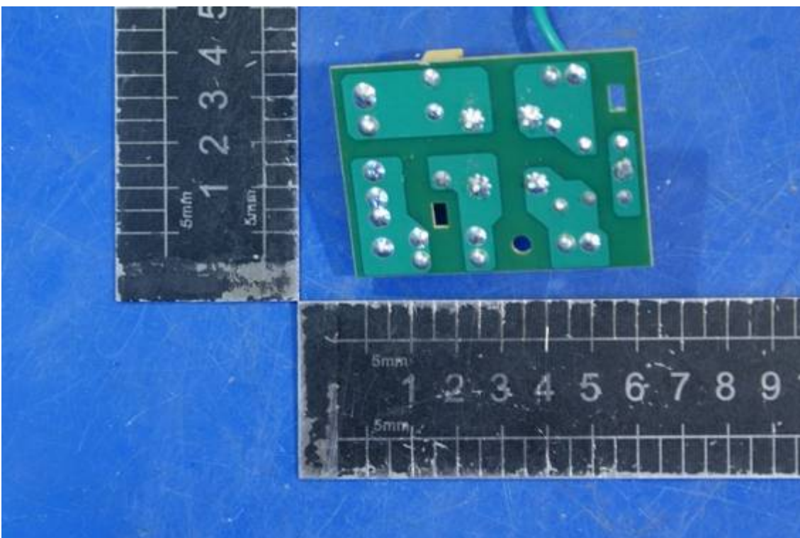
Photo 16 Internal photo of EUT (MEW50S-A)
