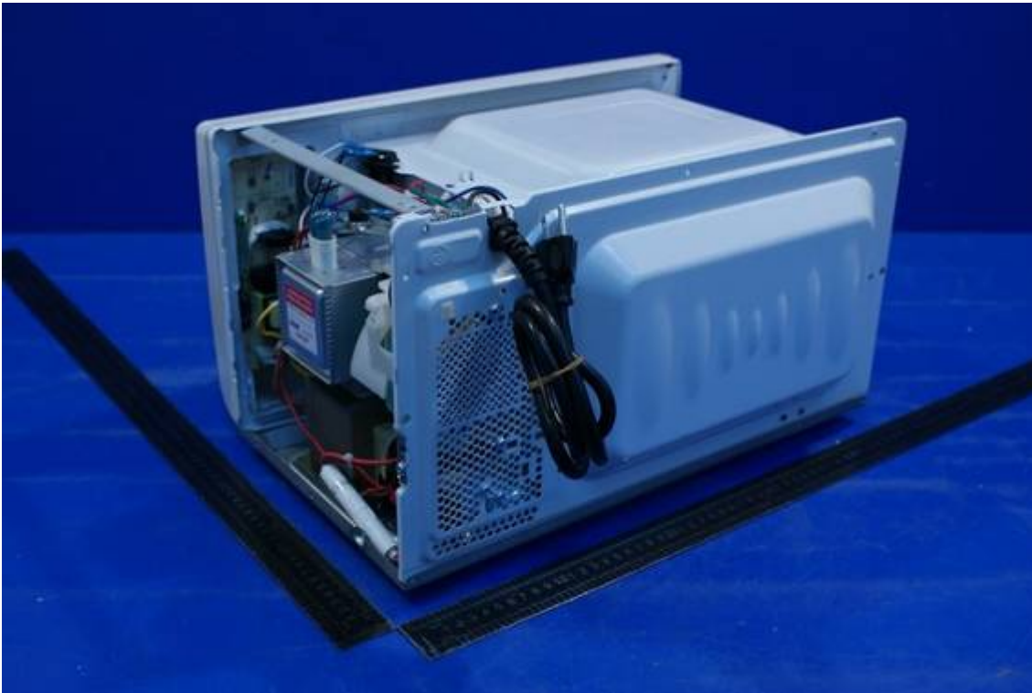
Photo 27 Internal photo of EUT (MEW50D-A)
