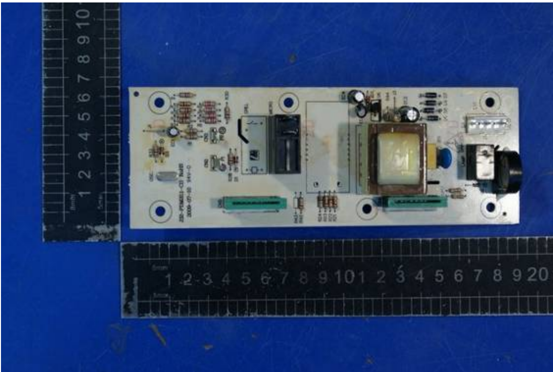
Photo 37 Internal photo of EUT (MEW50D-A)
