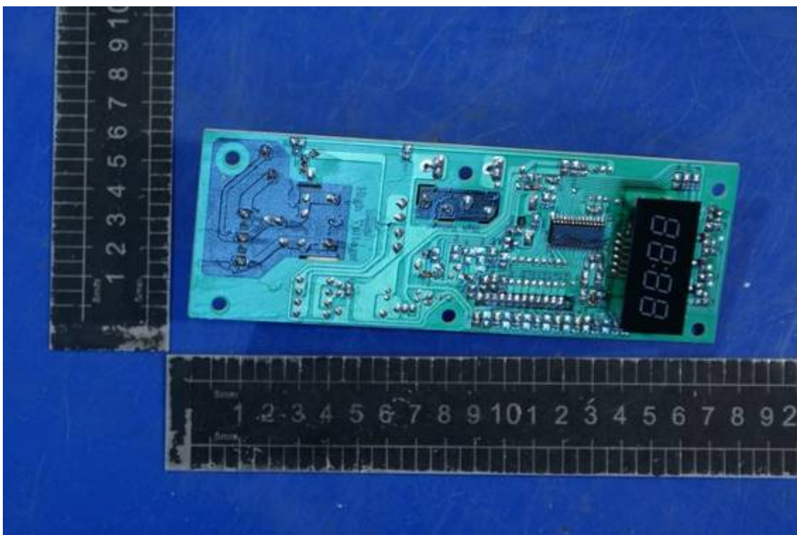
Photo 30 Internal photo of EUT (MEW50D-A)
