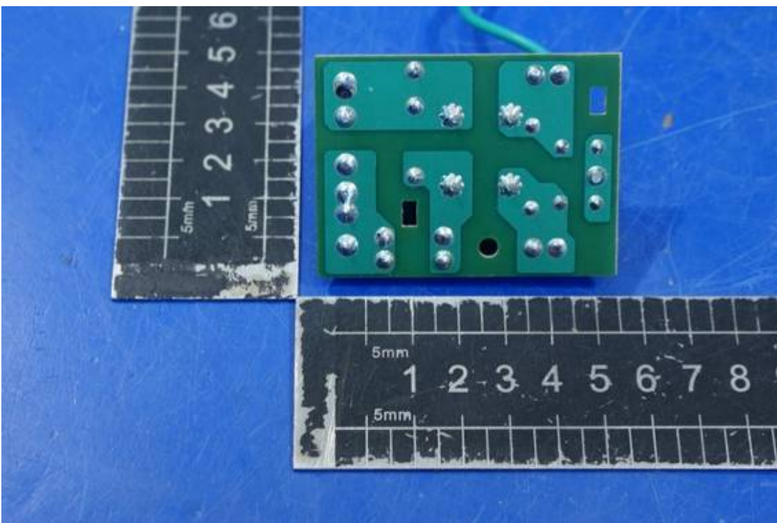
Photo 8 Internal photo of EUT (MEW50N-A)
