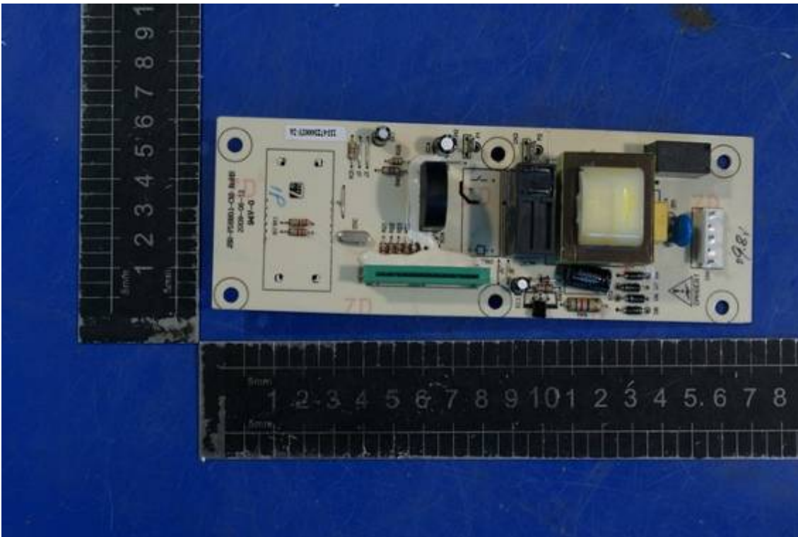
Photo 21 Internal photo of EUT (MEW50B-A)
