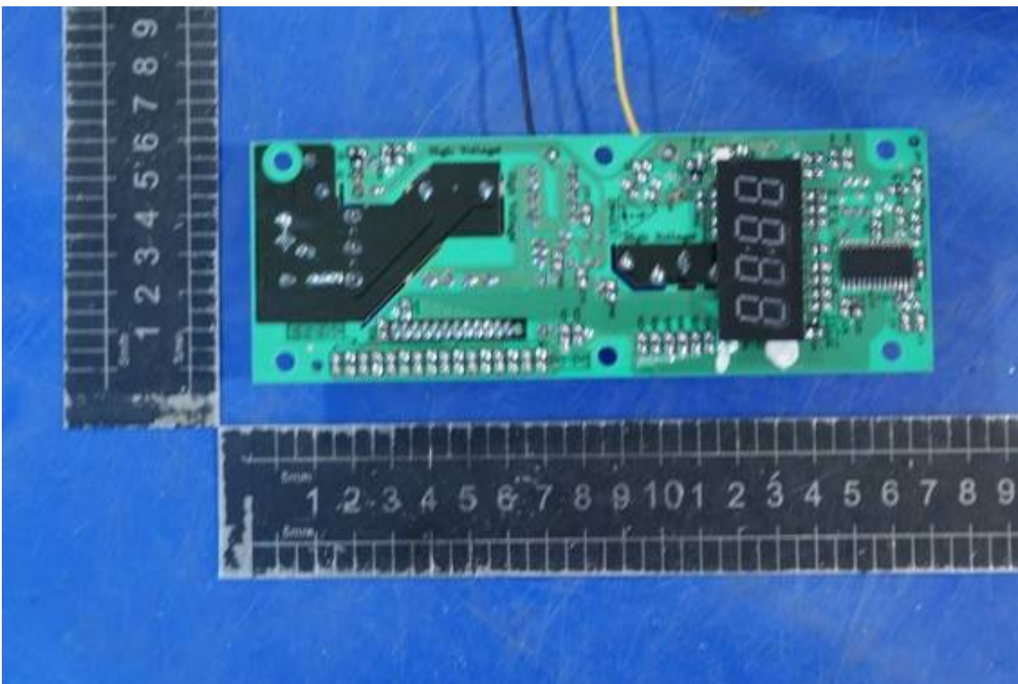
Photo 14 Internal photo of EUT (MEW50S-A)
