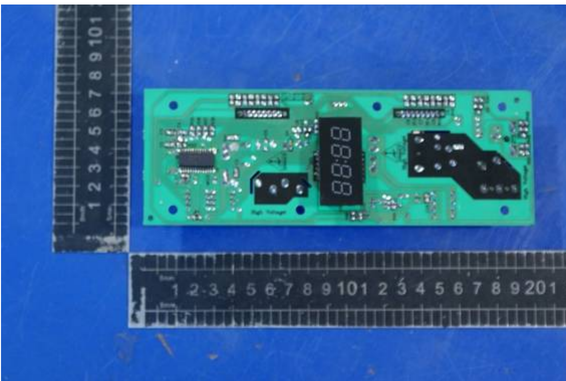
Photo 38 Internal photo of EUT (MEW50D-A)
