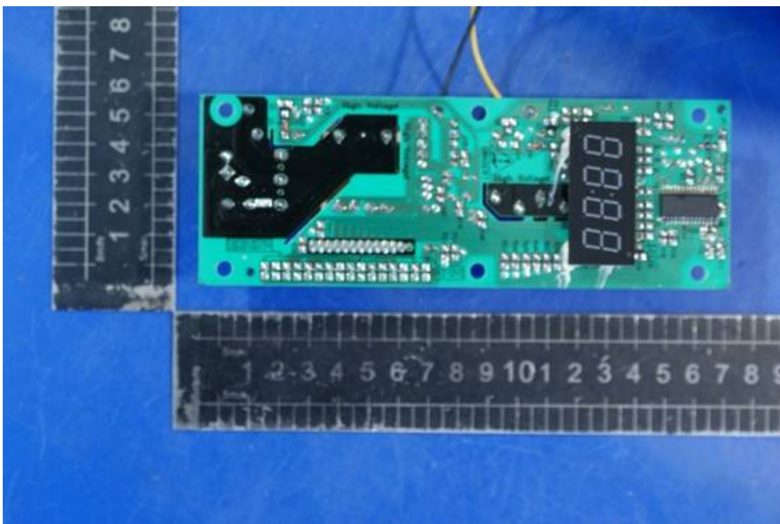
Photo 6 Internal photo of EUT (MEW50N-A)
