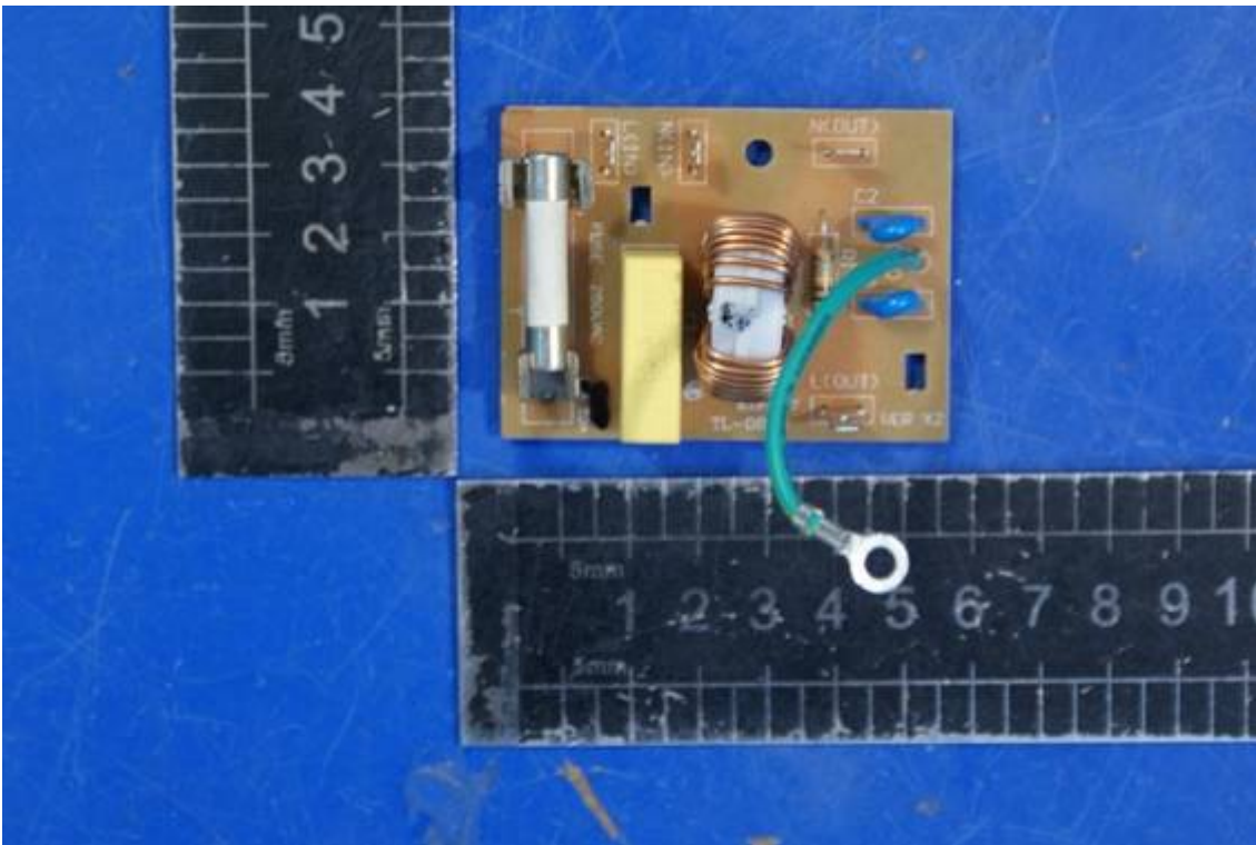
Photo 39 Internal photo of EUT (MEW50D-A)
