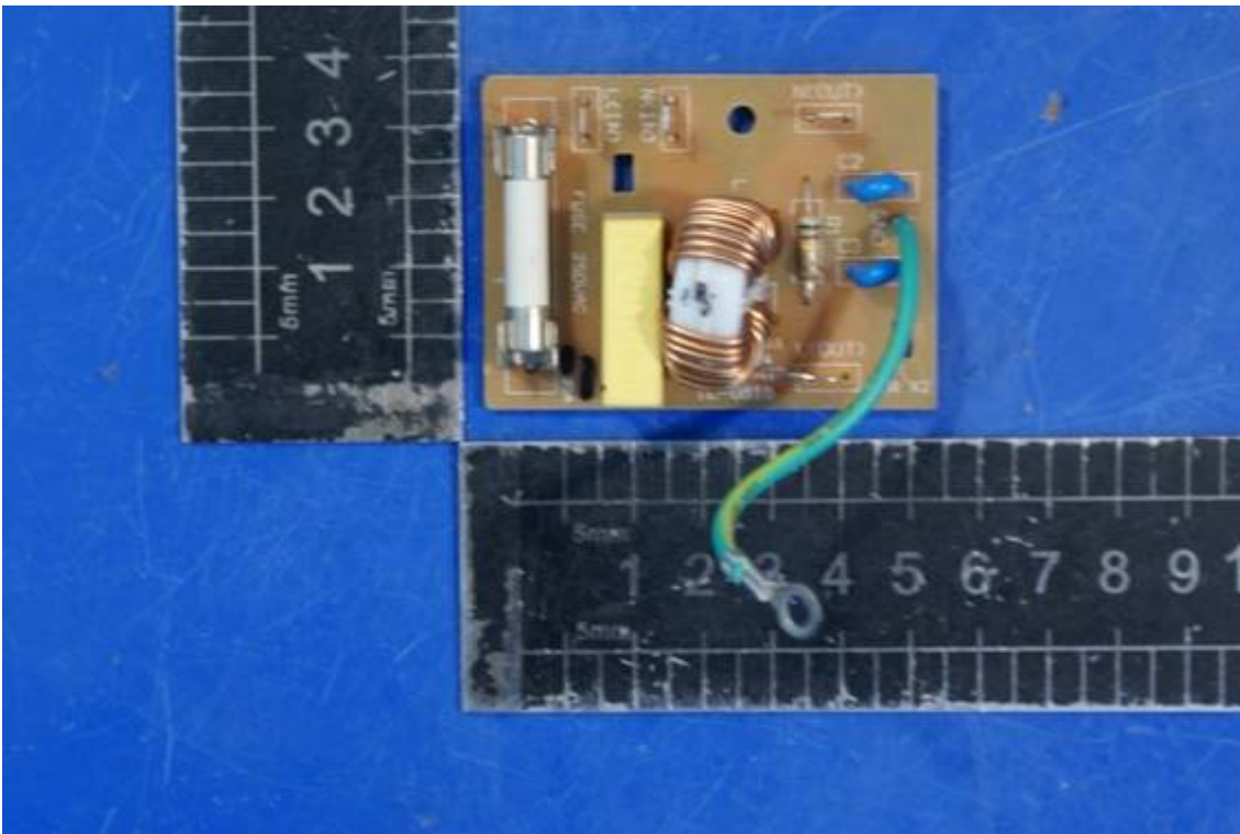
Photo 7 Internal photo of EUT (MEW50N-A)
