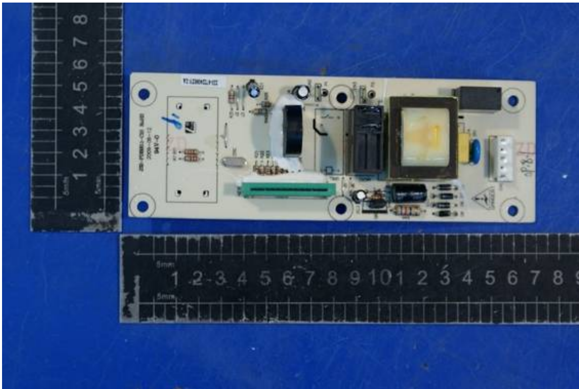
Photo 29 Internal photo of EUT (MEW50D-A)
