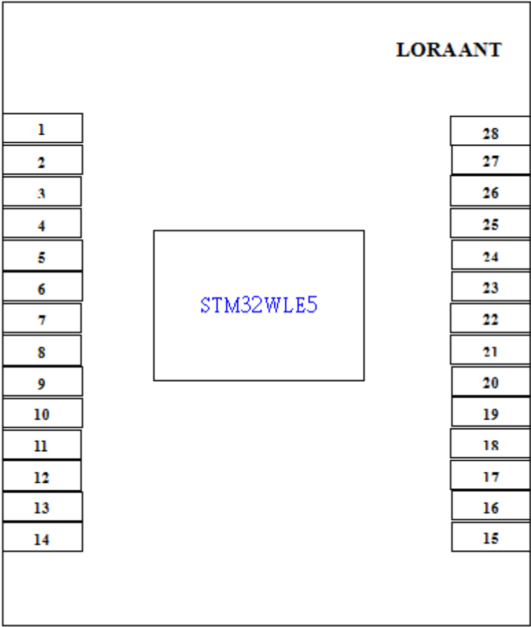
Figure 2 Block diagram
