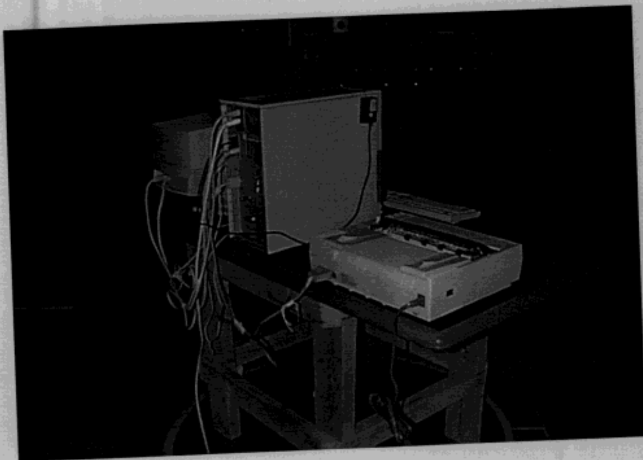
Photograph 4.2 Radiated Emission Measurements Setup
