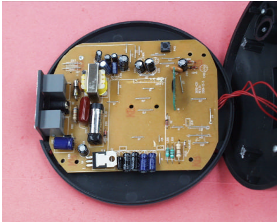
Base Main PCB comp side (View 2)
