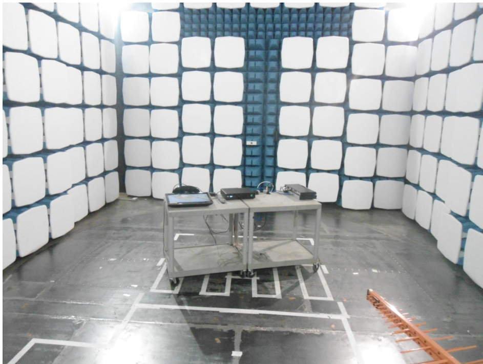
FCC Part 15B Radiated Emissions (Enclosure Port)
