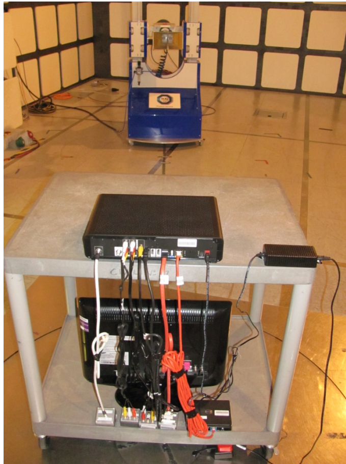
FCC Part 15.247 Radiated Emissions 1-18GHz
