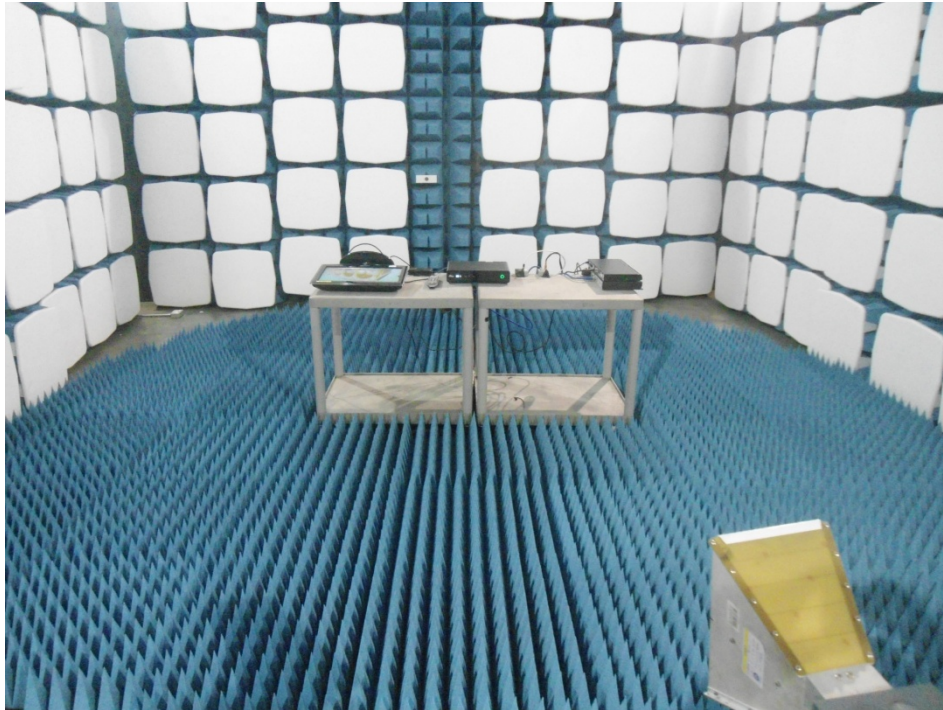
FCC Part 15B Radiated Emissions above 1 GHz (Enclosure Port)
