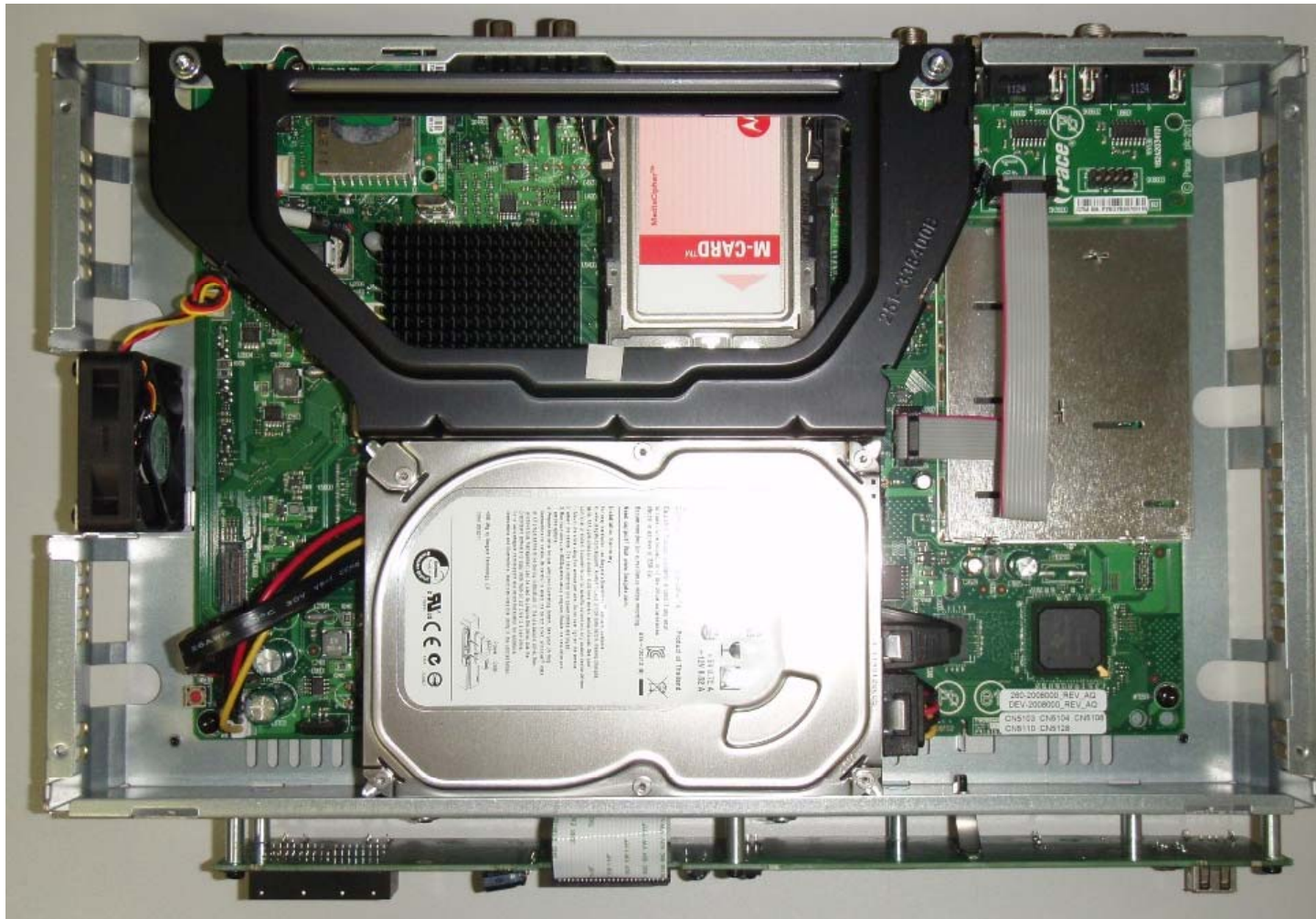
TOP - HDD Fitted
