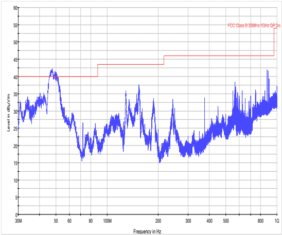
30 MHz – 1 GHz
