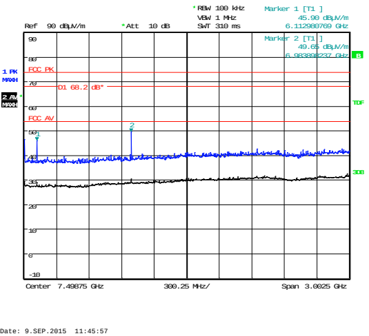
6 GHz – 9 GHz
