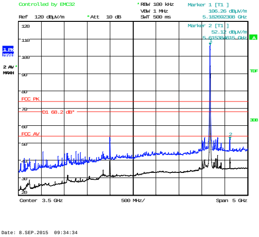
1 GHz – 6 GHz
