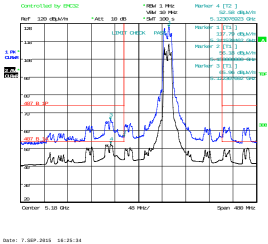
Bandedge
