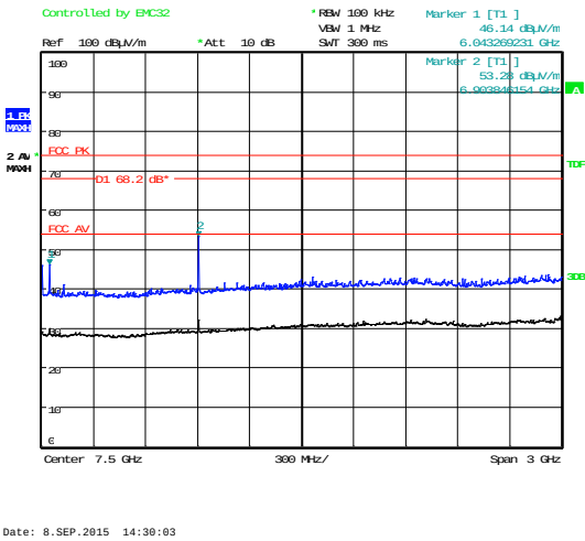
6 GHz – 9 GHz
