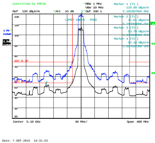
Bandedge
