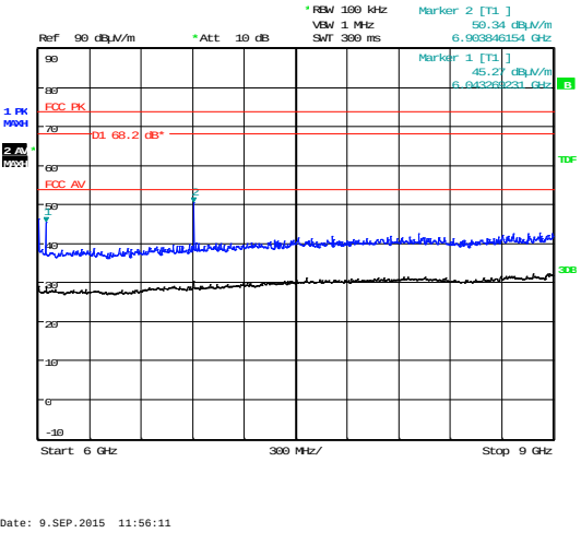
6 GHz – 9 GHz
