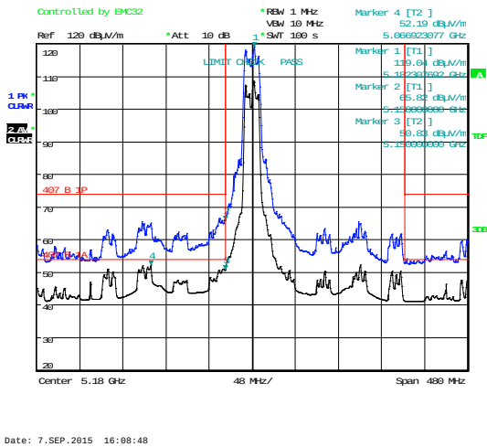
Bandedge
