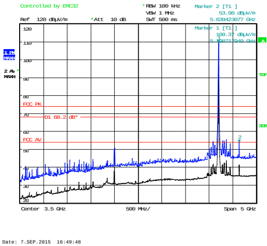
1 GHz – 6 GHz
