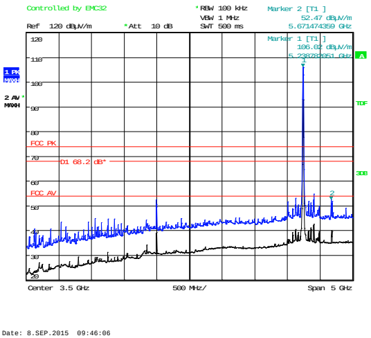
1 GHz – 6 GHz
