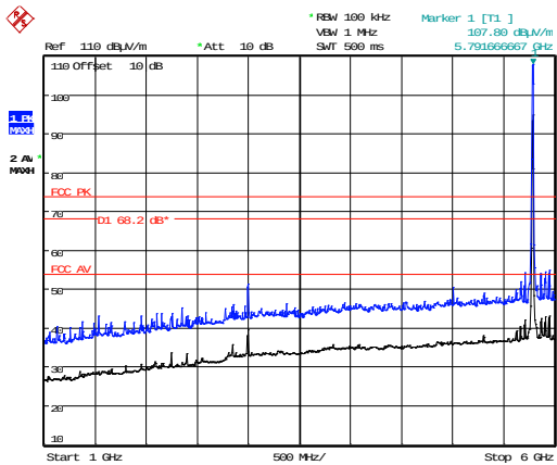
Bandedge
