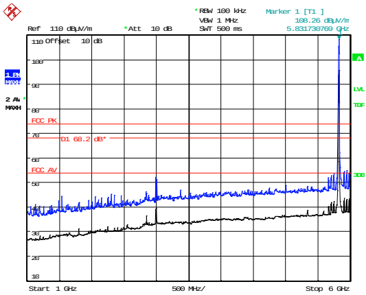
Bandedge
