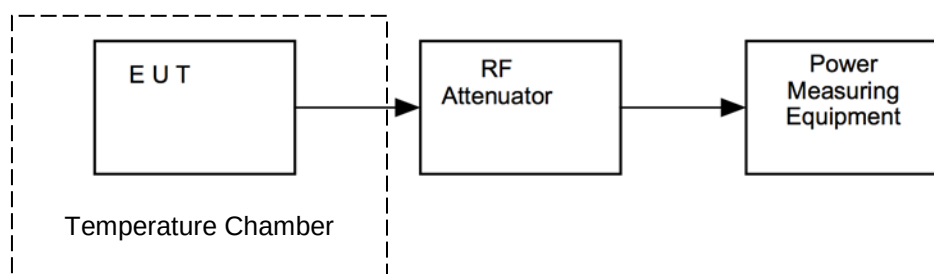
Figure vii Test Setup
