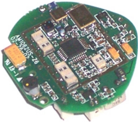
Assembled PCB top side view (transmitter area)
