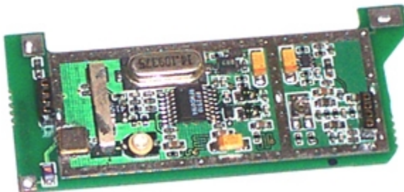
Assembled transmitter-board top view (one side assembled only)
