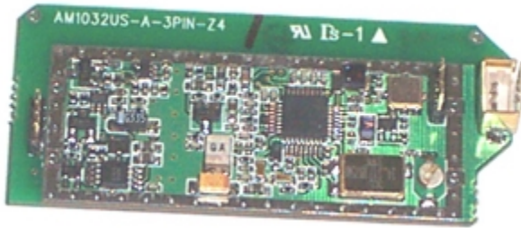
Assembled receiver-board top view
