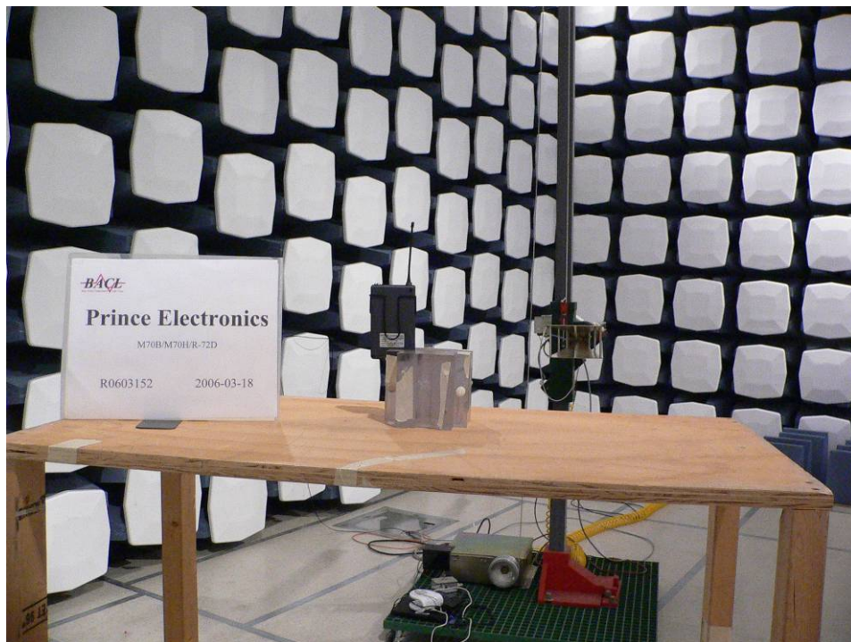
Radiated Emission - Rear View (M-70B)
