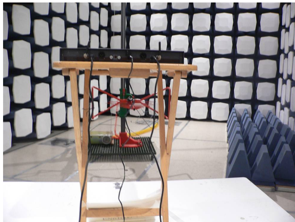
Radiated Emission - Rear View (R-72D)
