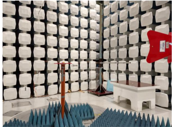
Radiated Emissions above 1GHz
