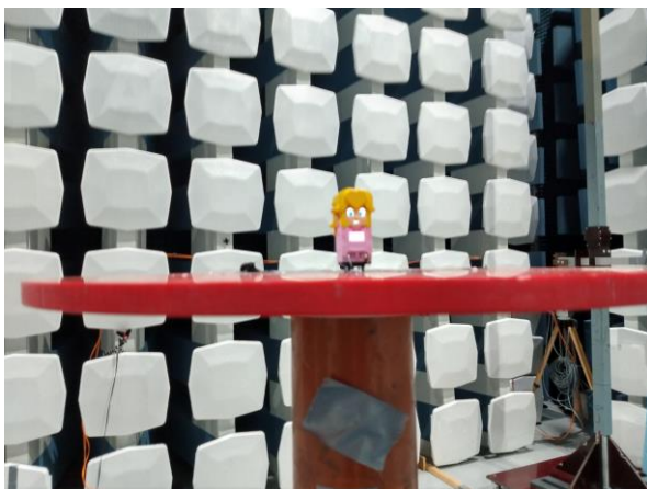
Radiated Emissions YZ plane
