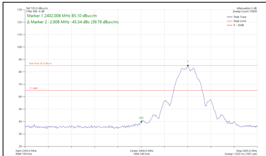
Figure 19 - CH37_LBE_LE1M_Core0_iPA, 2402 MHz, Band Edge Frequency 2400 MHz
