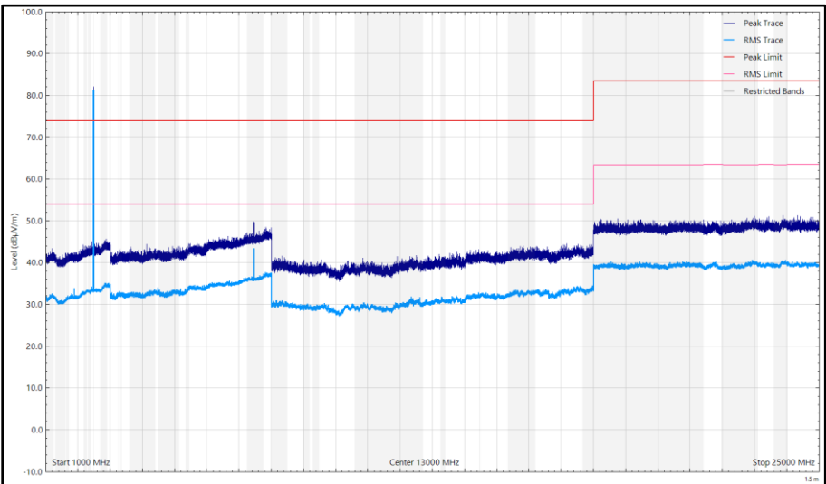
Figure 55 - CH39_LE1M_Y Plane, 2480 MHz, 1 GHz to 25 GHz, Vertical
