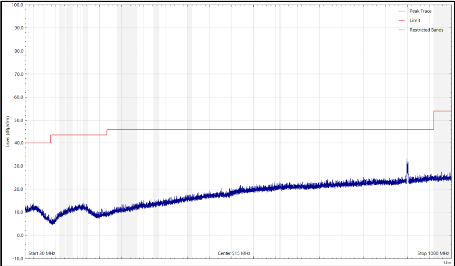
Figure 26 - CH37_LE1M_X Plane, 2402 MHz, 30 MHz to 1 GHz, Vertical (Peak)
