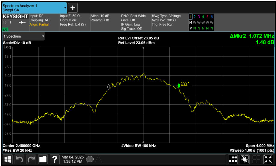
Figure 10 - 2480 MHz (CH39) 99% Bandwidth
