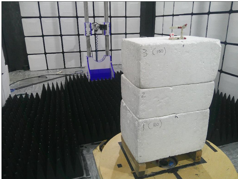
Figure 65 - Test Setup - 1 GHz to 8 GHz Z Plane
