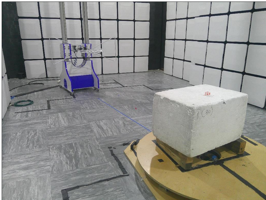
Figure 61 - Test Setup - 30 MHz to 1 GHz Y Plane
