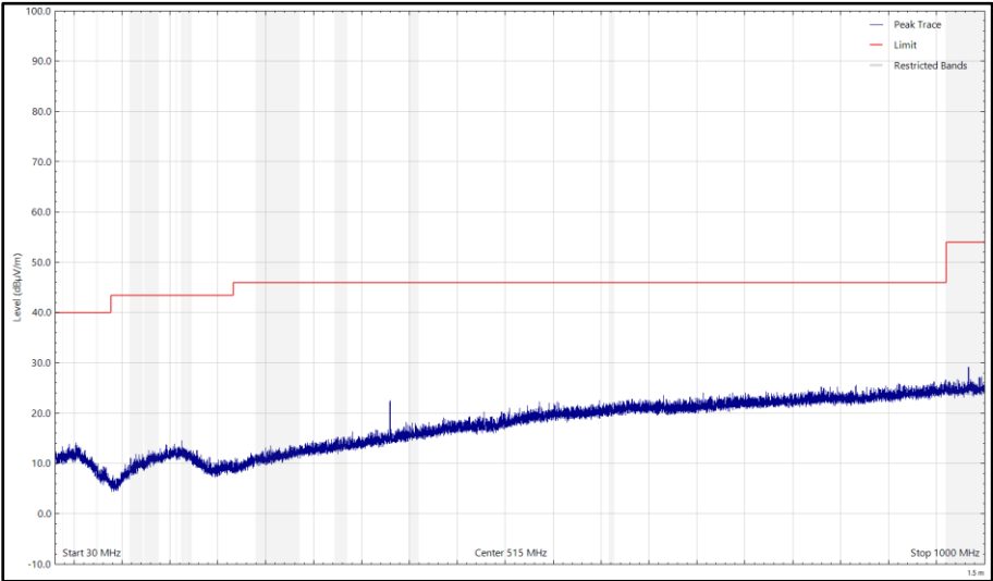
Figure 42 - CH18_LE1M_Y Plane, 2442 MHz, 30 MHz to 1 GHz, Vertical (Peak)
