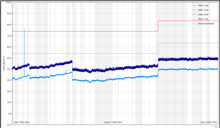
Figure 27 - CH37_LE1M_X Plane, 2402 MHz, 1 GHz to 25 GHz, Vertical
