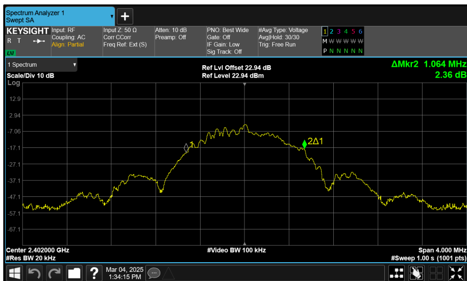
Figure 6 - 2402 MHz (CH37) 99% Bandwidth
