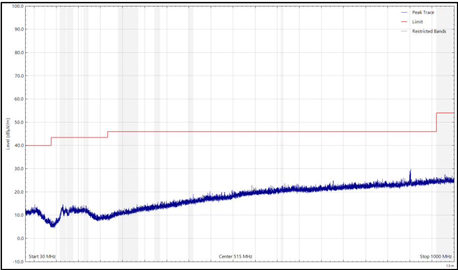
Figure 32 - CH37_LE1M_Z Plane, 2402 MHz, 30 MHz to 1 GHz, Horizontal (Peak)
