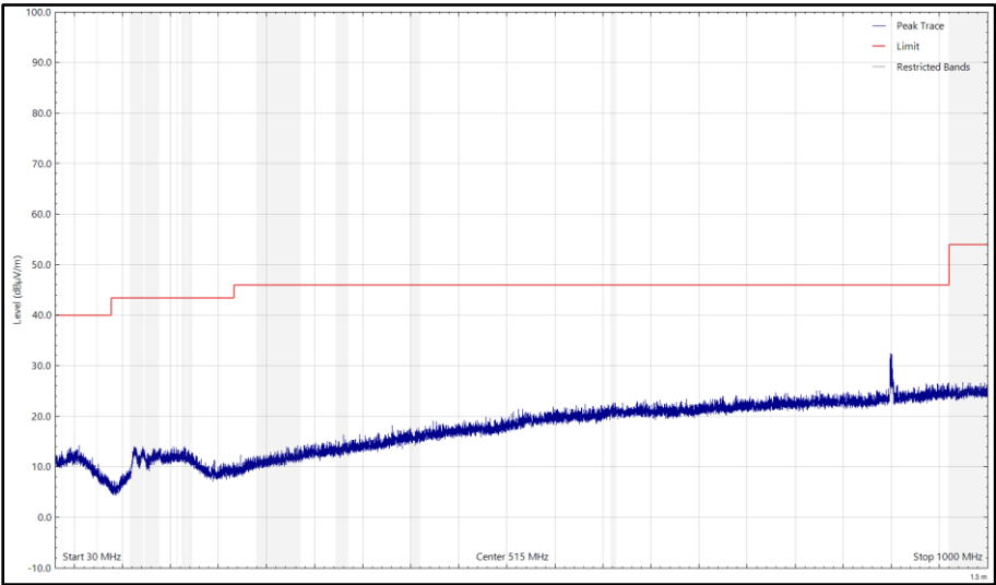
Figure 24 - CH37_LE1M_X Plane, 2402 MHz, 30 MHz to 1 GHz, Horizontal (Peak)
