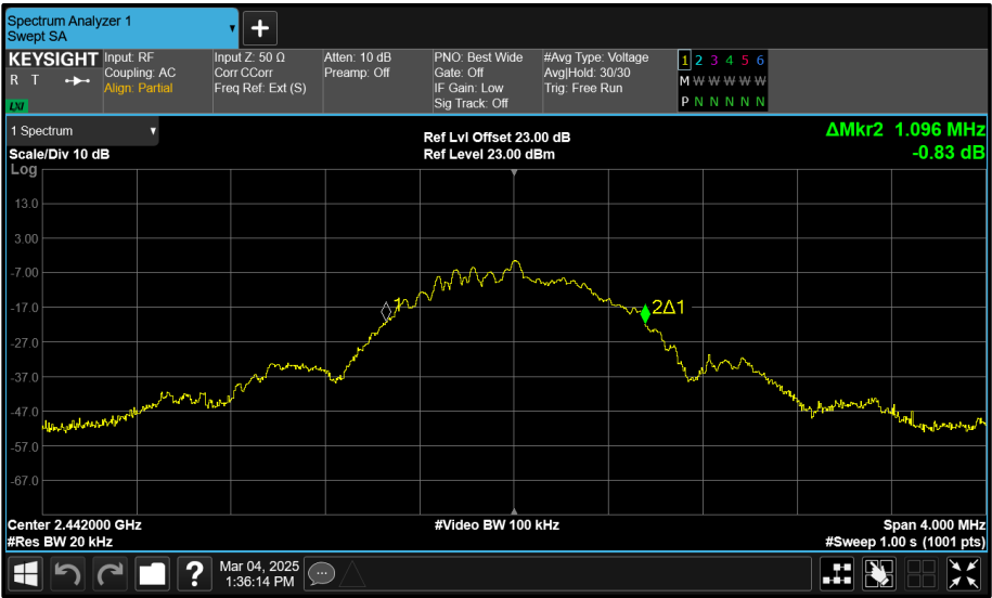
Figure 8 - 2442 MHz (CH18) 99% Bandwidth
