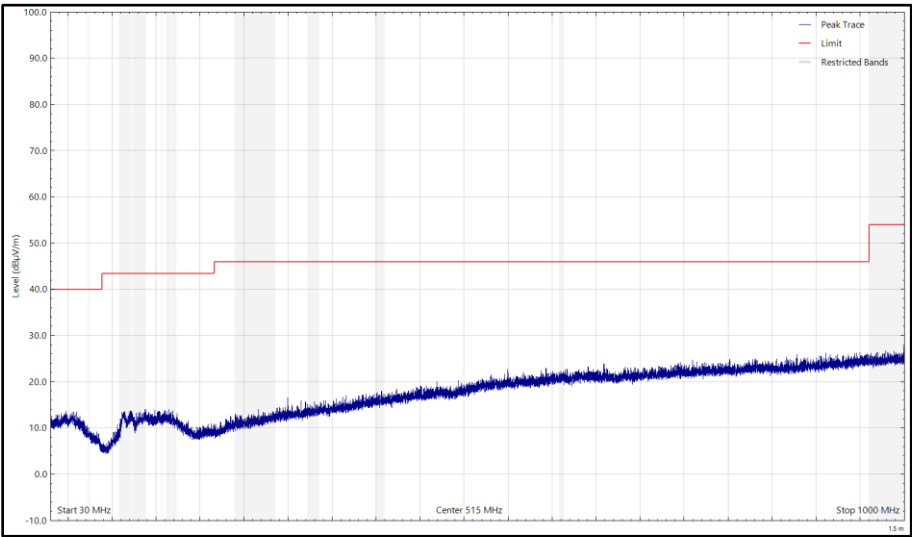
Figure 36 - CH18_LE1M_X Plane, 2442 MHz, 30 MHz to 1 GHz, Horizontal (Peak)
