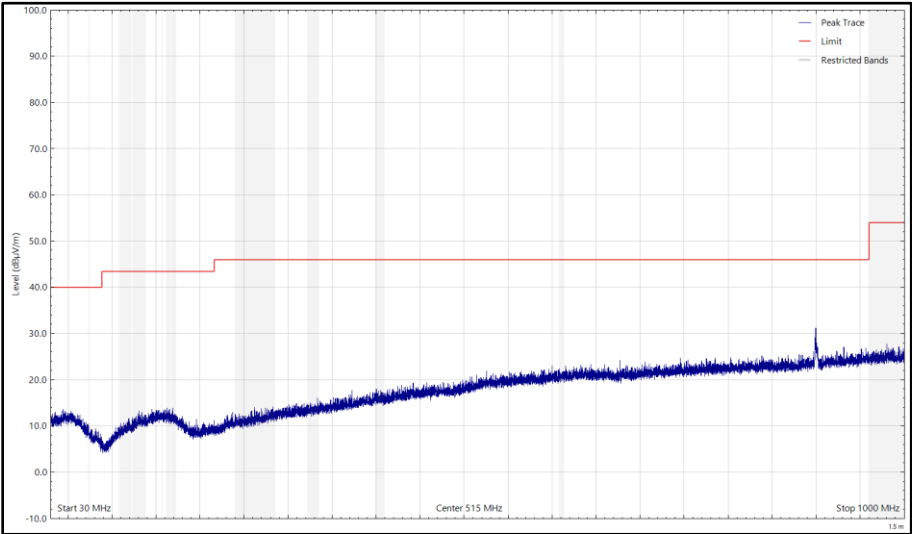
Figure 58 - CH39_LE1M_Z Plane, 2480 MHz, 30 MHz to 1 GHz, Vertical (Peak)
