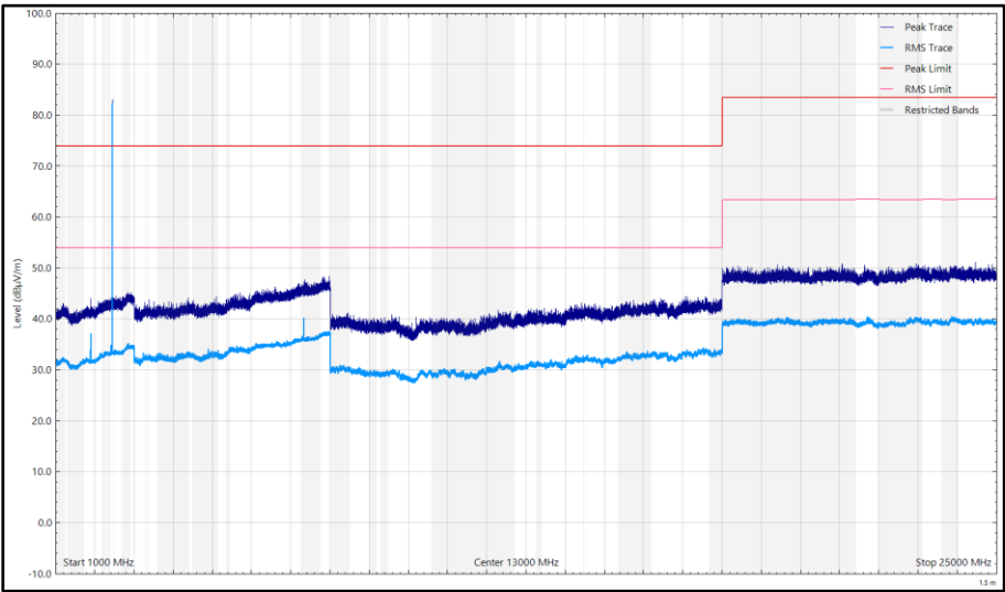
Figure 45 - CH18_LE1M_Z Plane, 2442 MHz, 1 GHz to 25 GHz, Horizontal
