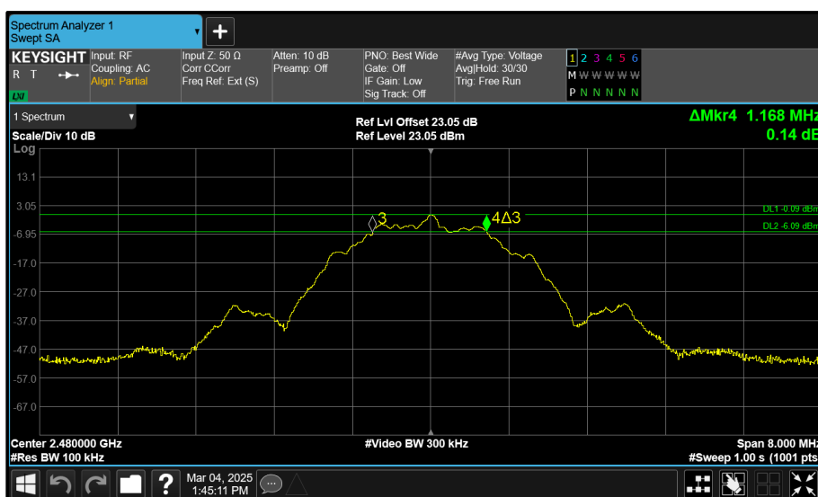
Figure 17 - 2480 MHz (CH39) 6 dB Bandwidth
