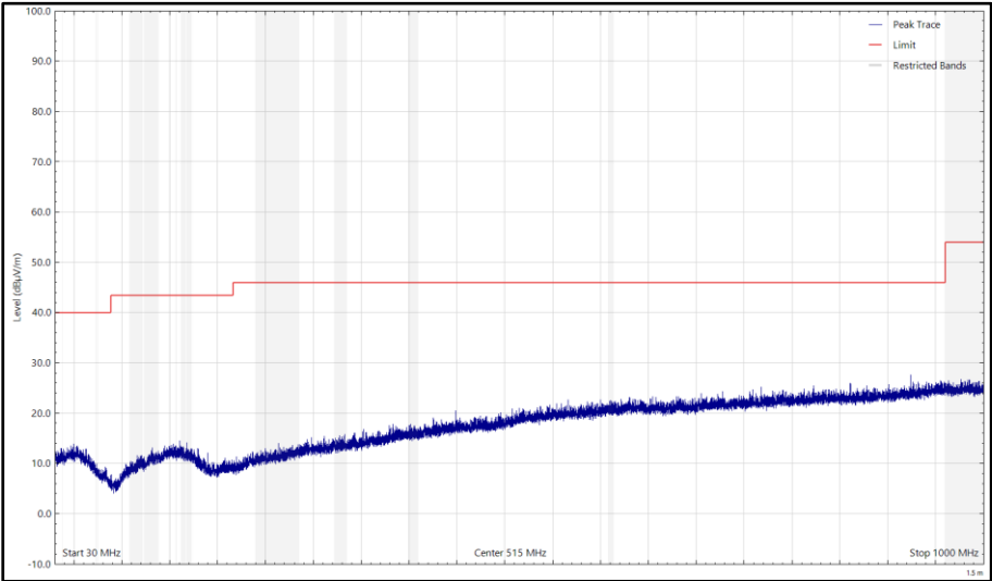
Figure 46 - CH18_LE1M_Z Plane, 2442 MHz, 30 MHz to 1 GHz, Vertical (Peak)
