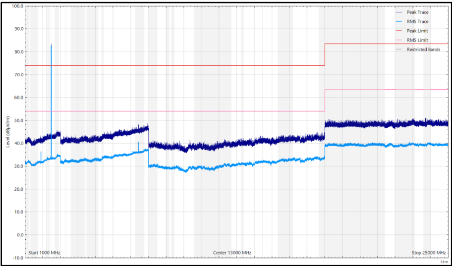
Figure 53 - CH39_LE1M_Y Plane, 2480 MHz, 1 GHz to 25 GHz, Horizontal
