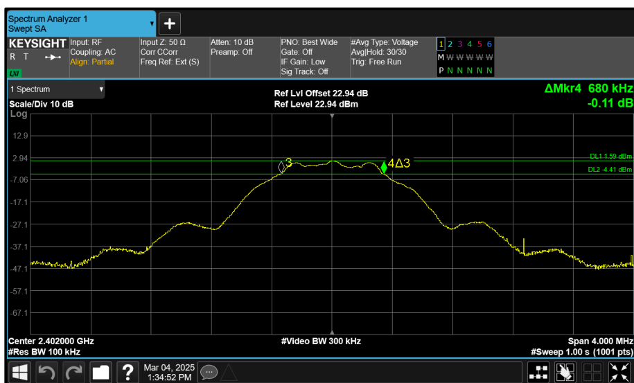
Figure 7 - 2402 MHz (CH37) 6 dB Bandwidth
