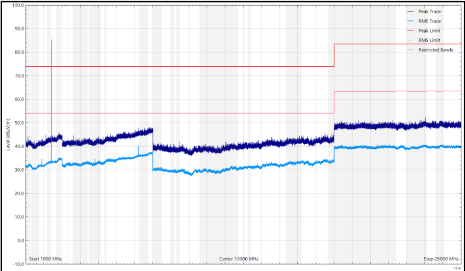
Figure 31 - CH37_LE1M_Y Plane, 2402 MHz, 1 GHz to 25 GHz, Vertical
