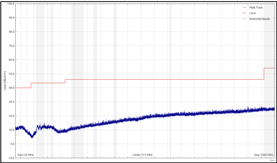
Figure 44 - CH18_LE1M_Z Plane, 2442 MHz, 30 MHz to 1 GHz, Horizontal (Peak)
