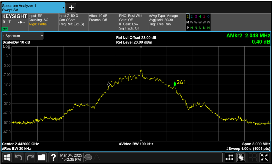
Figure 14 - 2442 MHz (CH18) 99% Bandwidth
