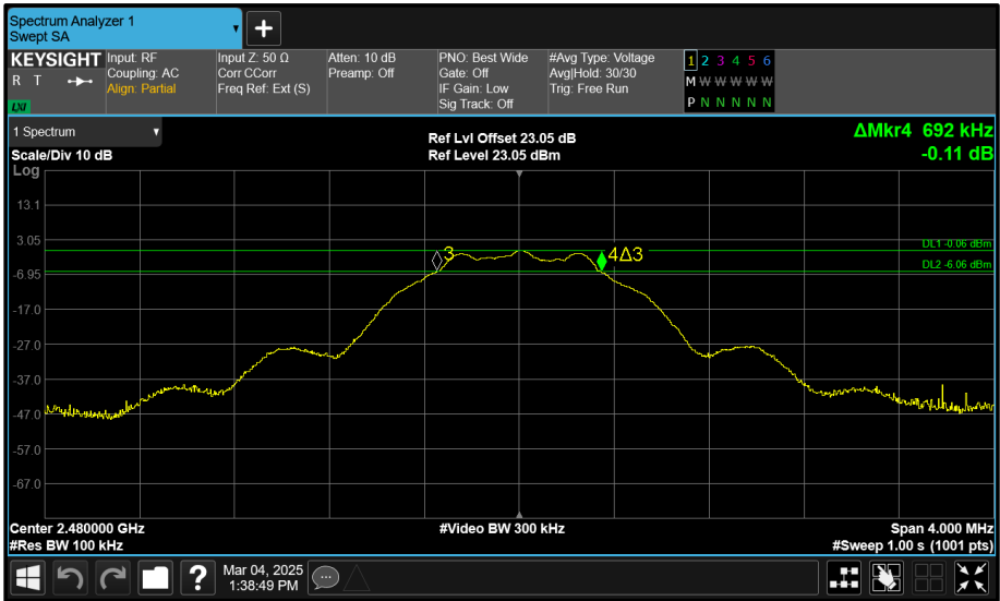
Figure 11 - 2480 MHz (CH39) 6 dB Bandwidth
