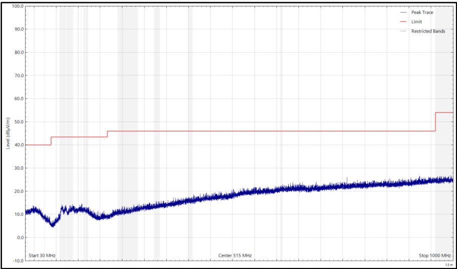
Figure 40 - CH18_LE1M_Y Plane, 2442 MHz, 30 MHz to 1 GHz, Horizontal (Peak)
