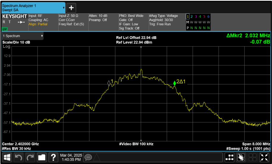
Figure 12 - 2402 MHz (CH37) 99% Bandwidth
