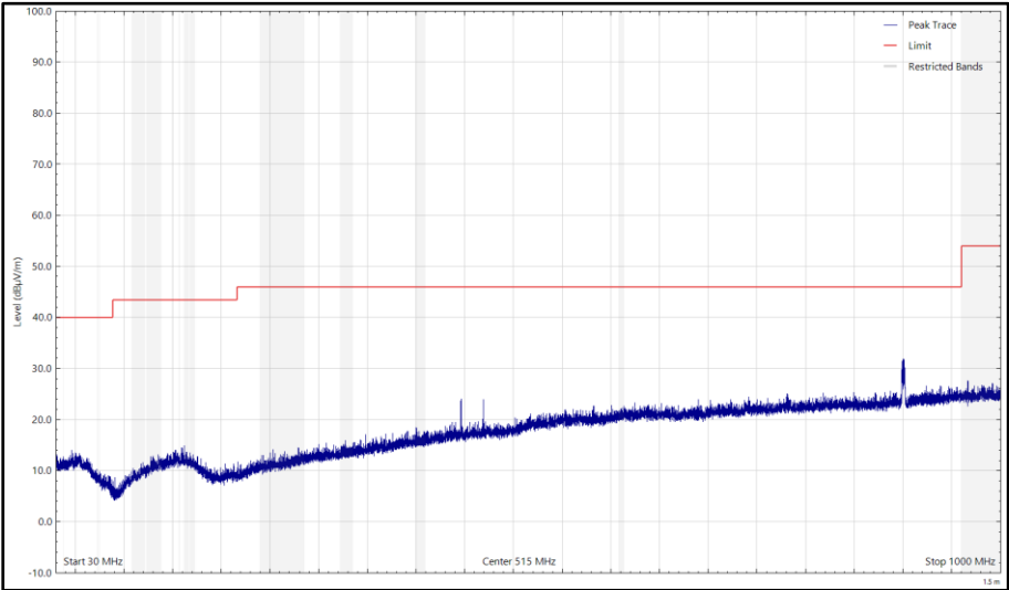
Figure 50 - CH39_LE1M_X Plane, 2480 MHz, 30 MHz to 1 GHz, Vertical (Peak)
