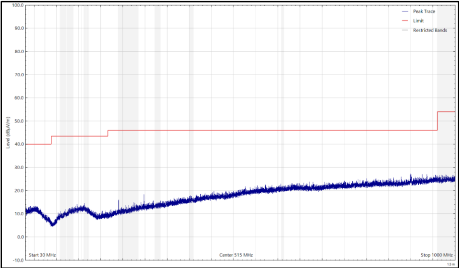
Figure 30 - CH37_LE1M_Y Plane, 2402 MHz, 30 MHz to 1 GHz, Vertical (Peak)
