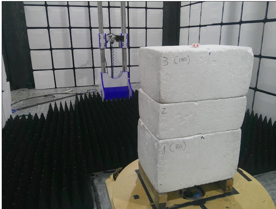
Figure 64 - Test Setup - 1 GHz to 8 GHz Y Plane
