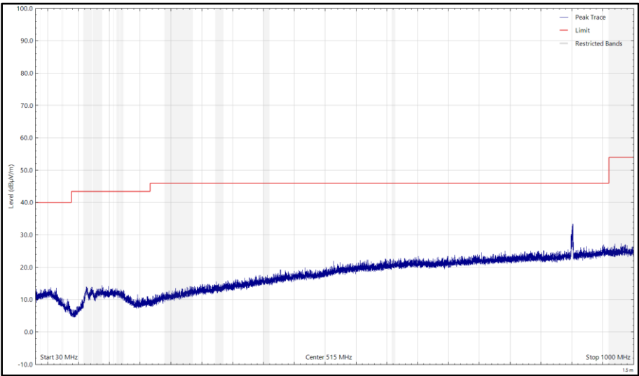
Figure 48 - CH39_LE1M_X Plane, 2480 MHz, 30 MHz to 1 GHz, Horizontal (Peak)
