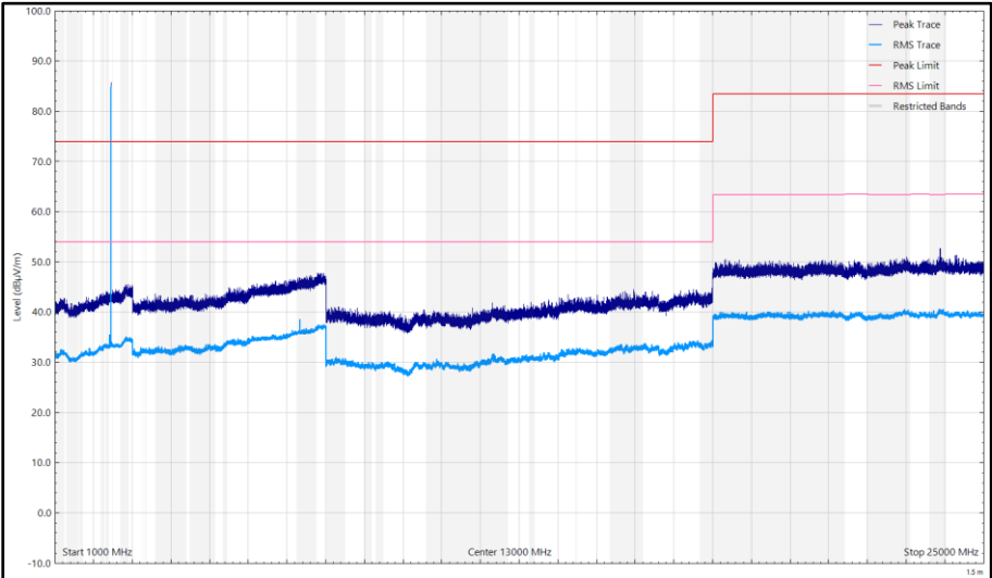
Figure 47 - CH18_LE1M_Z Plane, 2442 MHz, 1 GHz to 25 GHz, Vertical
