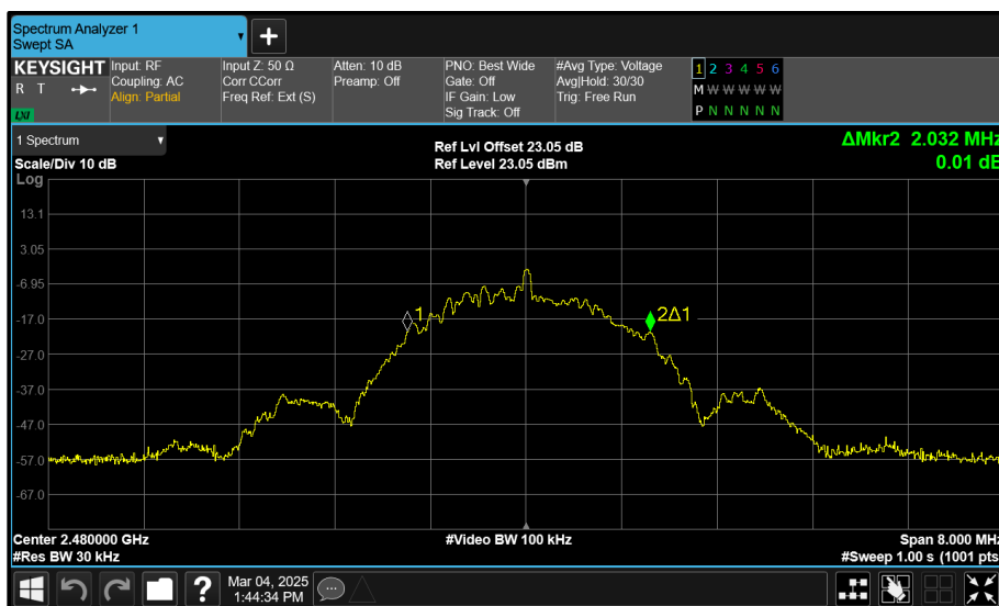
Figure 16 - 2480 MHz (CH39) 99% Bandwidth
