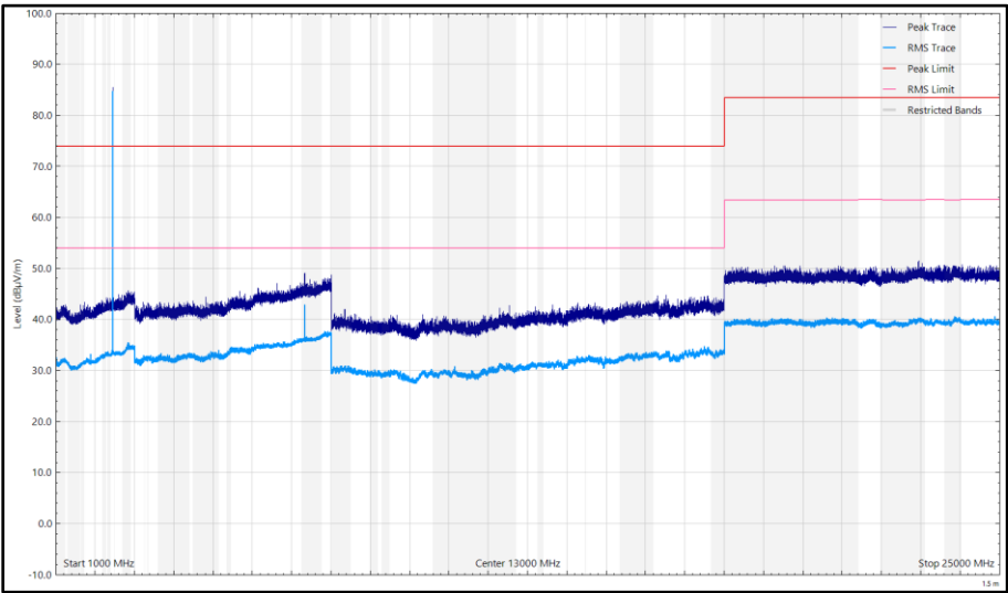
Figure 37 - CH18_LE1M_X Plane, 2442 MHz, 1 GHz to 25 GHz, Horizontal
