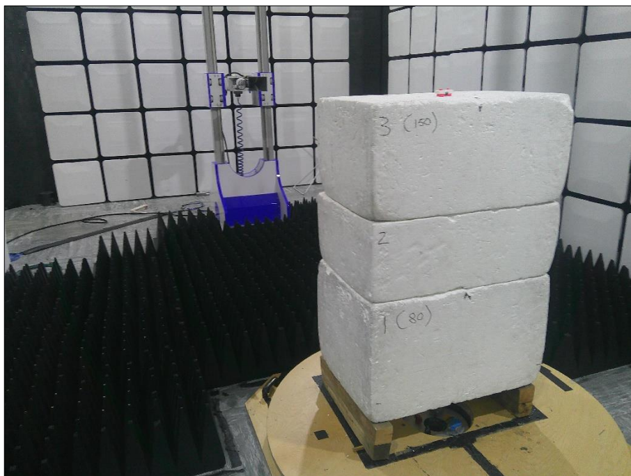
Figure 63 - Test Setup - 1 GHz to 8 GHz X Plane
