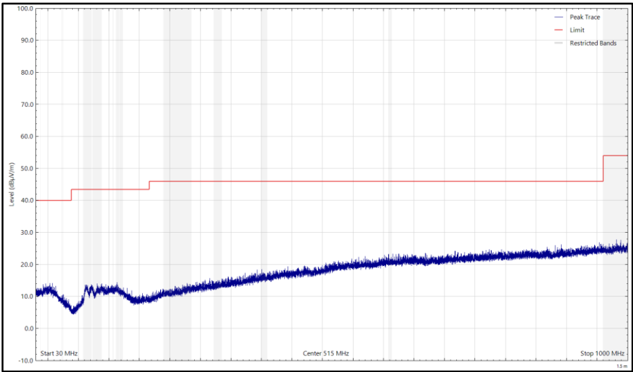
Figure 56 - CH39_LE1M_Z Plane, 2480 MHz, 30 MHz to 1 GHz, Horizontal (Peak)
