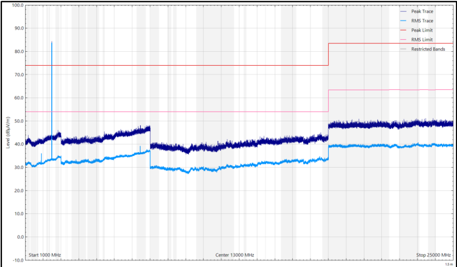
Figure 59 - CH39_LE1M_Z Plane, 2480 MHz, 1 GHz to 25 GHz, Vertical
