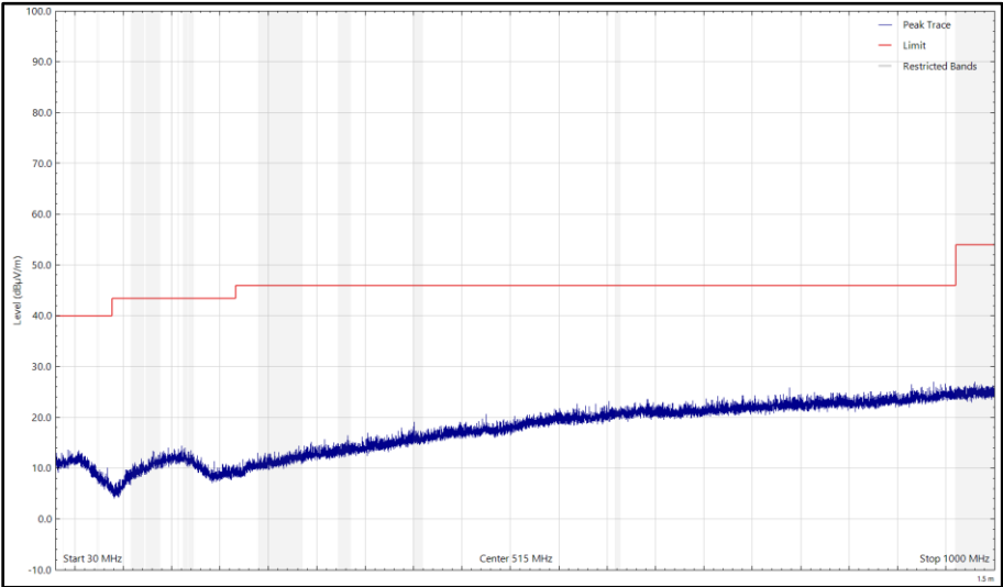
Figure 38 - CH18_LE1M_X Plane, 2442 MHz, 30 MHz to 1 GHz, Vertical (Peak)
