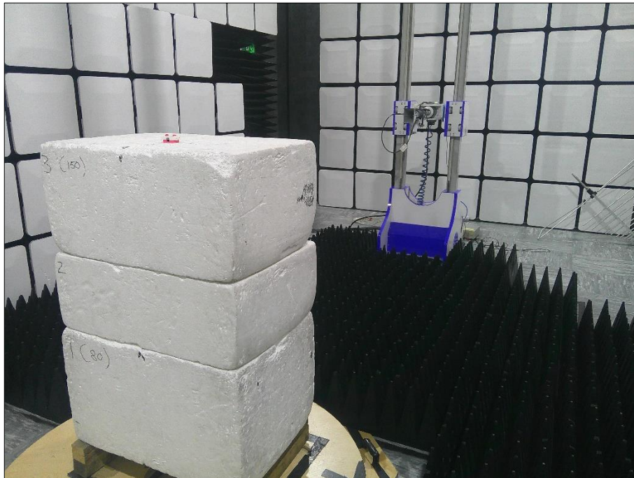
Figure 66 - Test Setup - 8 GHz to 18 GHz X Plane
