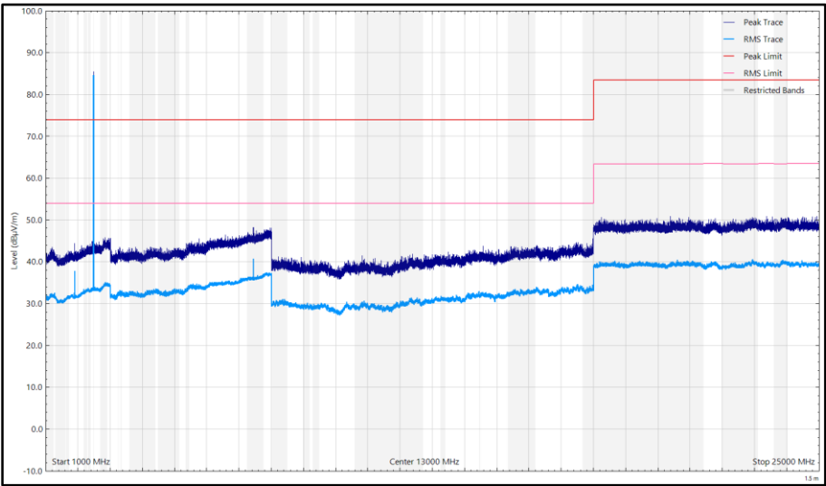
Figure 49 - CH39_LE1M_X Plane, 2480 MHz, 1 GHz to 25 GHz, Horizontal
