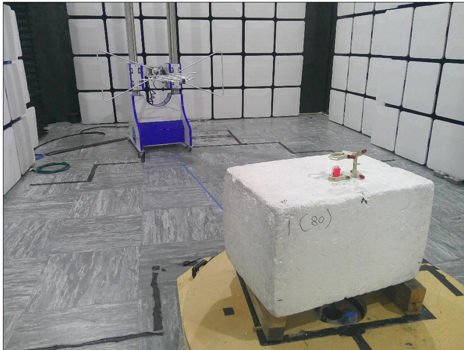
Figure 62 - Test Setup - 30 MHz to 1 GHz Z Plane
