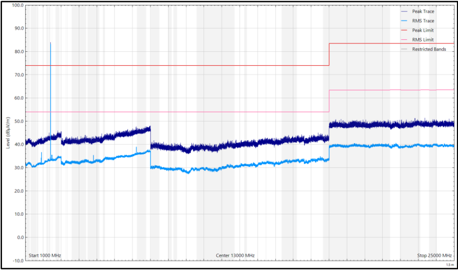
Figure 33 - CH37_LE1M_Z Plane, 2402 MHz, 1 GHz to 25 GHz, Horizontal
