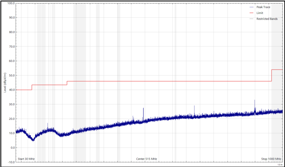
Figure 54 - CH39_LE1M_Y Plane, 2480 MHz, 30 MHz to 1 GHz, Vertical (Peak)
