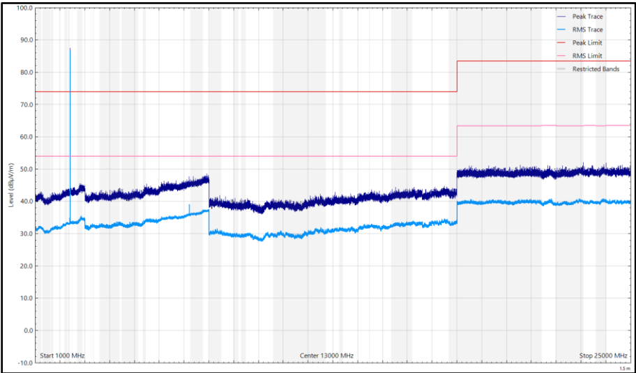
Figure 25 - CH37_LE1M_X Plane, 2402 MHz, 1 GHz to 25 GHz, Horizontal
