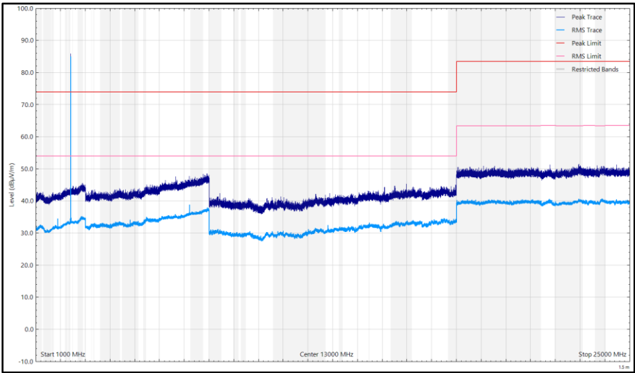
Figure 29 - CH37_LE1M_Y Plane, 2402 MHz, 1 GHz to 25 GHz, Horizontal
