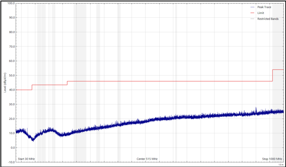
Figure 34 - CH37_LE1M_Z Plane, 2402 MHz, 30 MHz to 1 GHz, Vertical (Peak)
