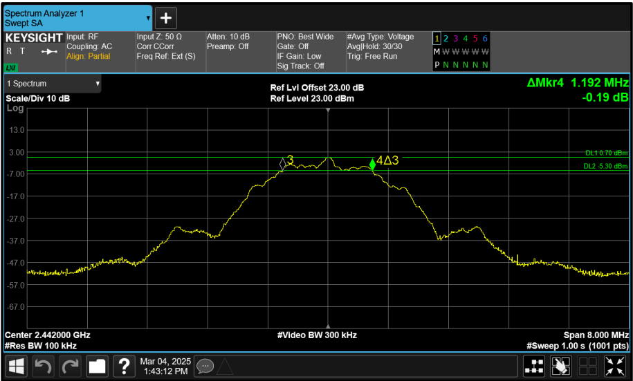
Figure 15 - 2442 MHz (CH18) 6 dB Bandwidth
