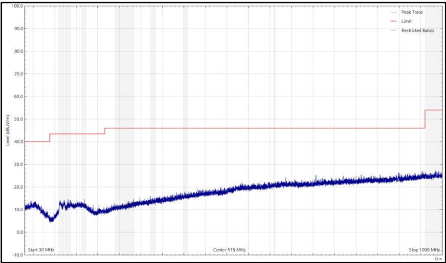
Figure 52 - CH39_LE1M_Y Plane, 2480 MHz, 30 MHz to 1 GHz, Horizontal (Peak)
