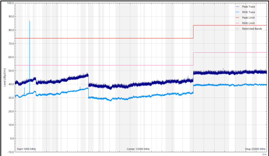
Figure 35 - CH37_LE1M_Z Plane, 2402 MHz, 1 GHz to 25 GHz, Vertical
