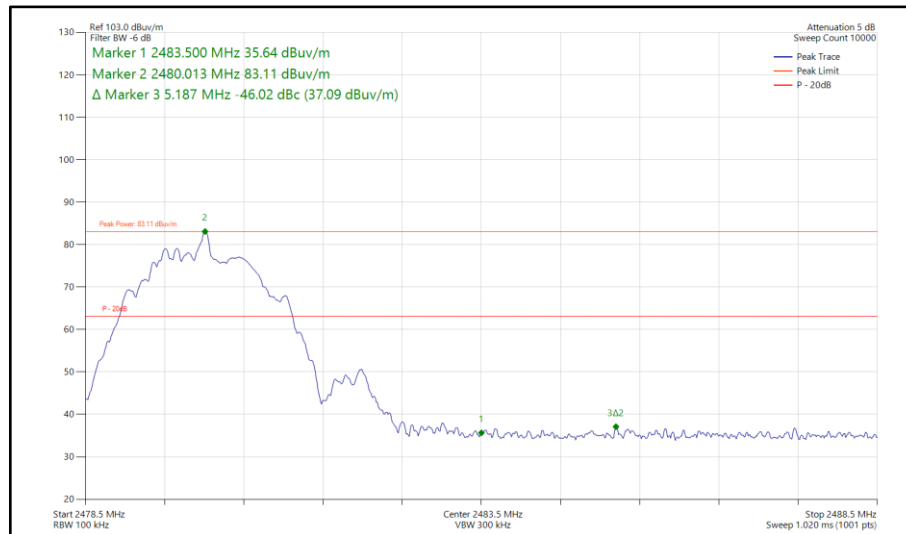
Figure 22 - CH39_UBE_LE2M_Core0_ePA, 2480 MHz, Band Edge Frequency 2483.5 MHz
