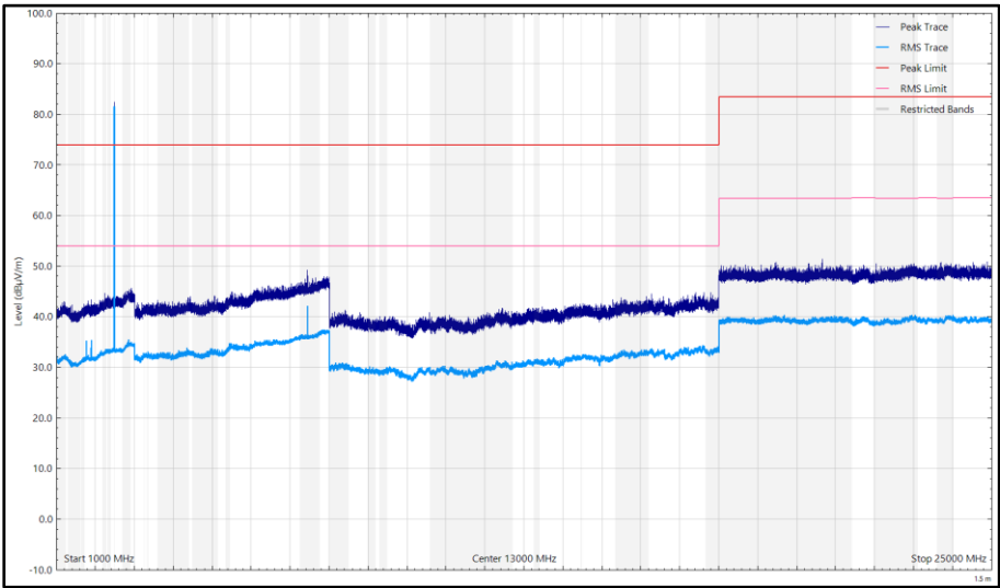
Figure 57 - CH39_LE1M_Z Plane, 2480 MHz, 1 GHz to 25 GHz, Horizontal
