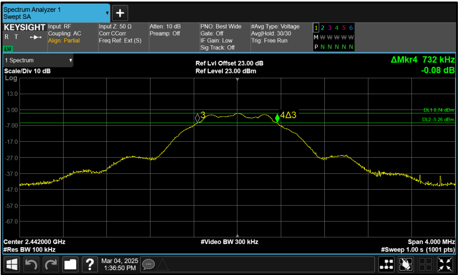
Figure 9 - 2442 MHz (CH18) 6 dB Bandwidth
