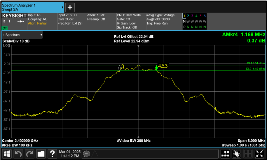
Figure 13 - 2402 MHz (CH37) 6 dB Bandwidth
