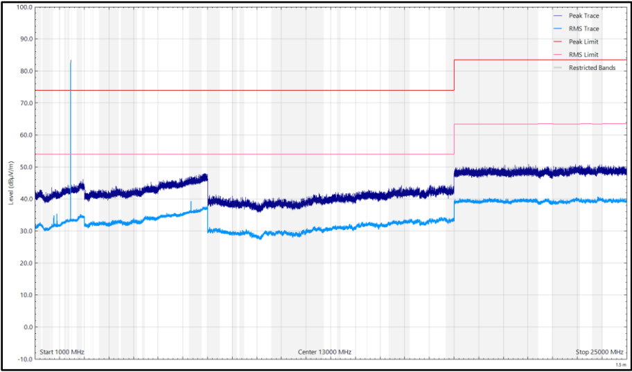
Figure 41 - CH18_LE1M_Y Plane, 2442 MHz, 1 GHz to 25 GHz, Horizontal
