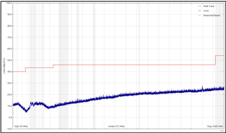
Figure 28 - CH37_LE1M_Y Plane, 2402 MHz, 30 MHz to 1 GHz, Horizontal (Peak)
