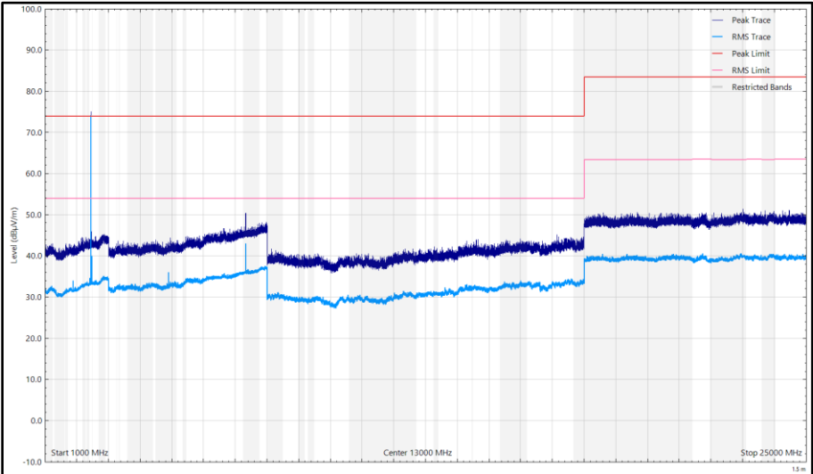
Figure 39 - CH18_LE1M_X Plane, 2442 MHz, 1 GHz to 25 GHz, Vertical
