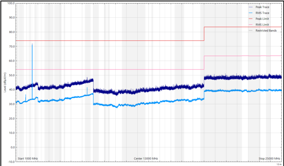
Figure 51 - CH39_LE1M_X Plane, 2480 MHz, 1 GHz to 25 GHz, Vertical
