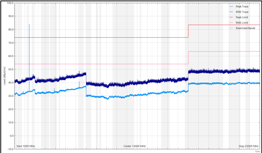
Figure 43 - CH18_LE1M_Y Plane, 2442 MHz, 1 GHz to 25 GHz, Vertical
