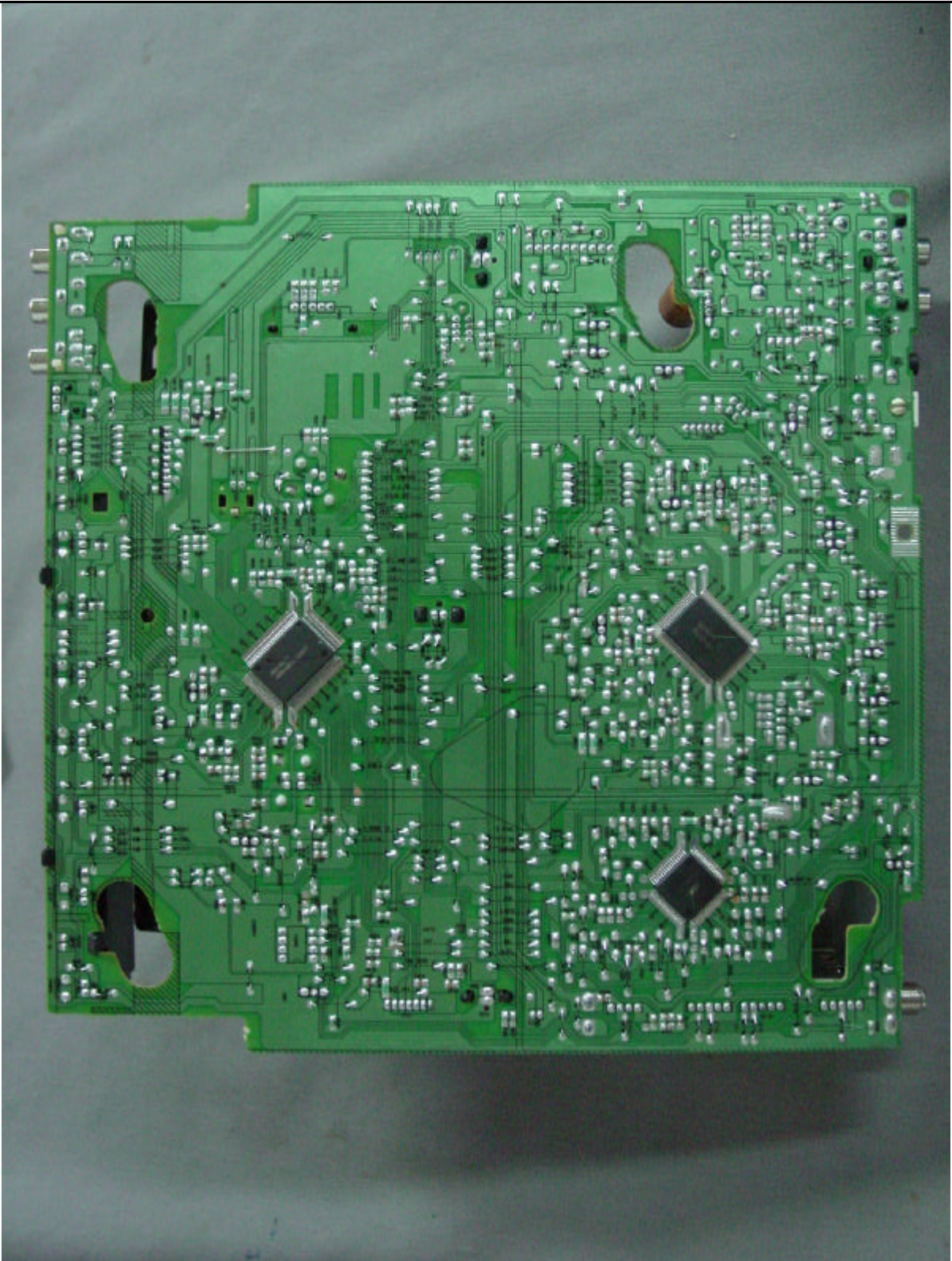
[ Bottom View of the Main Board ]
