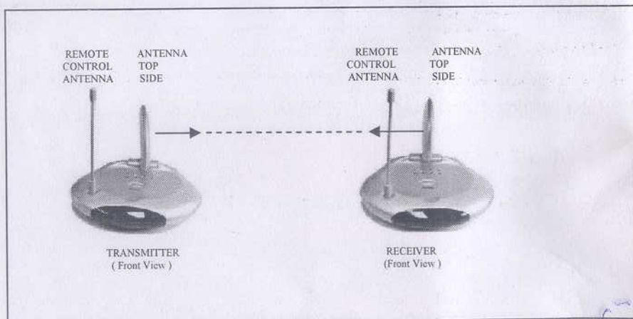
Fig-1: How to orienting the 5.8GHz audio and video antennas.
