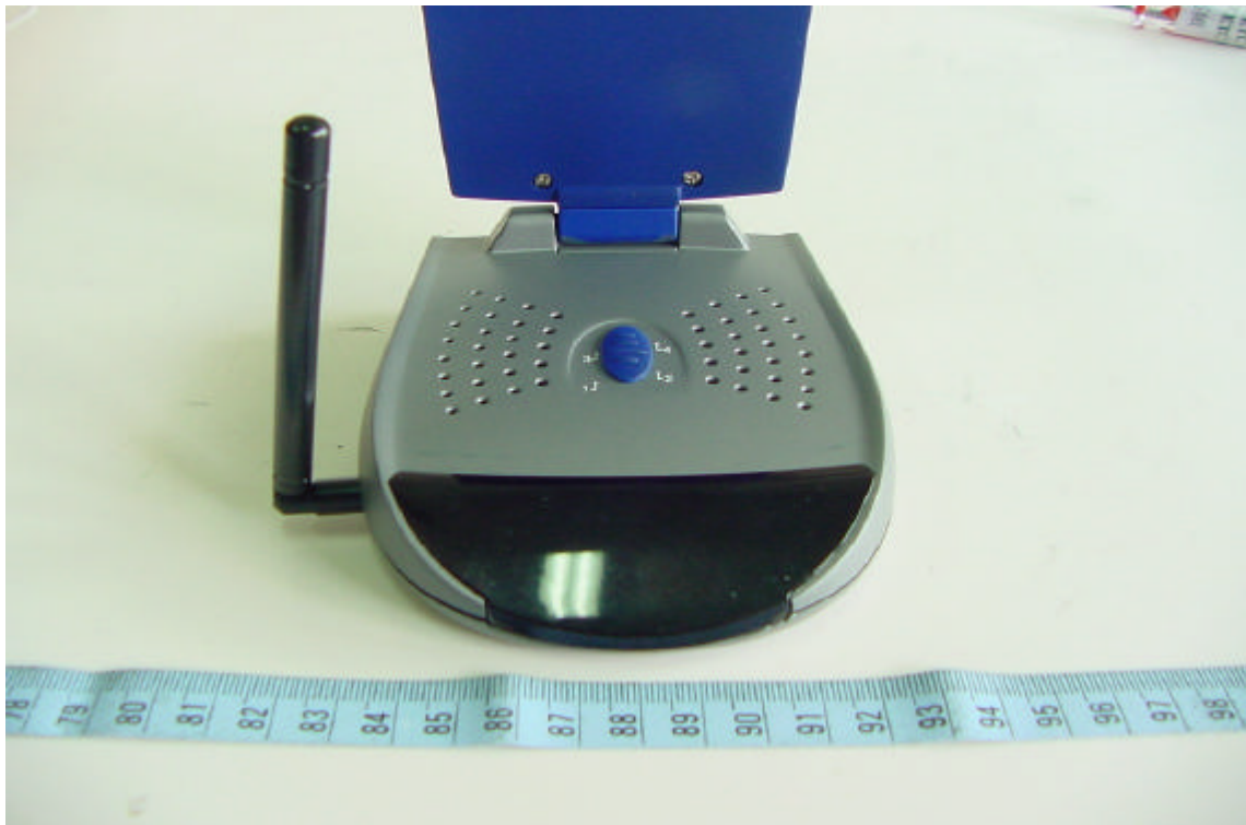
Front View of Receiver
