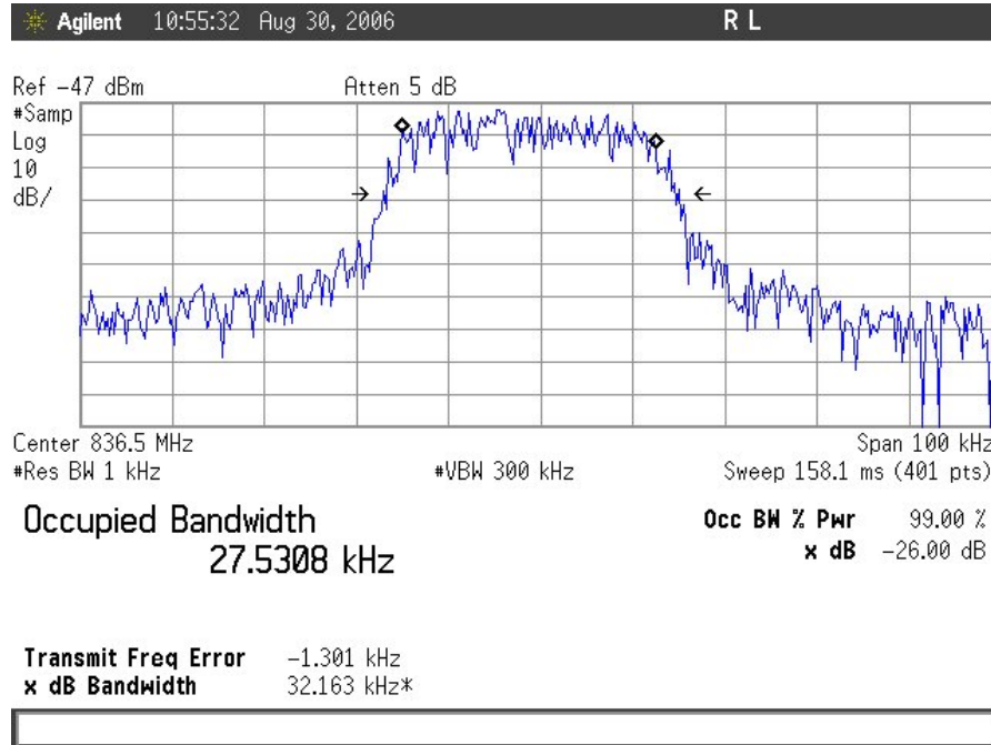
TDMA Uplink Input (Mid Channel - Cellular)
