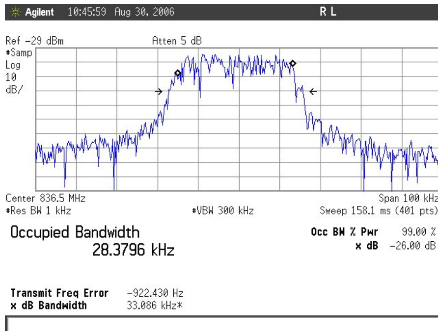
TDMA Uplink Output (Mid Channel - Cellular)
