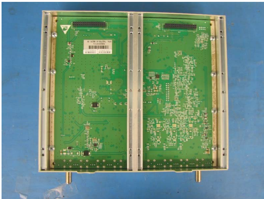
Internal Assembly 2
