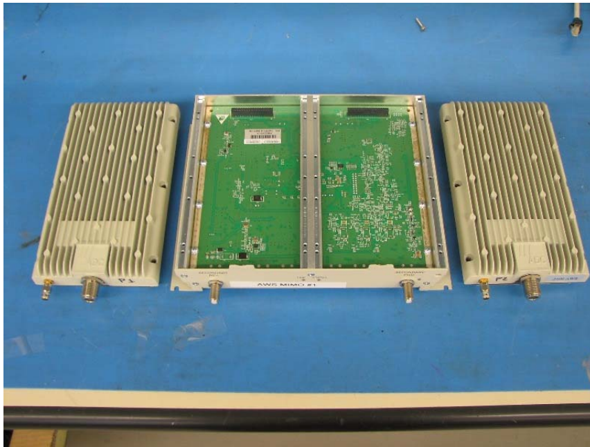
Internal Assembly 1
