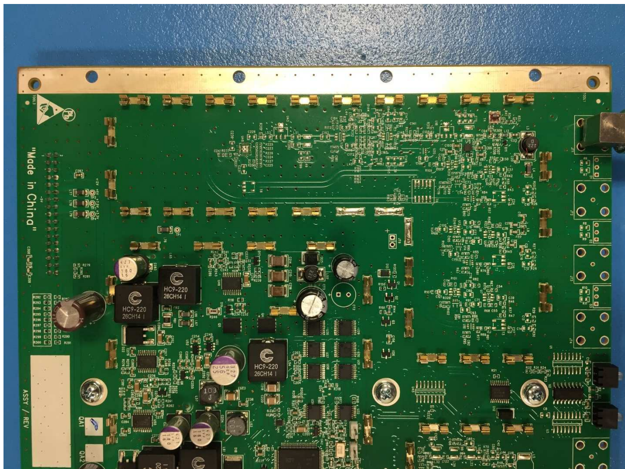
IF Board Bottom Right Side View
