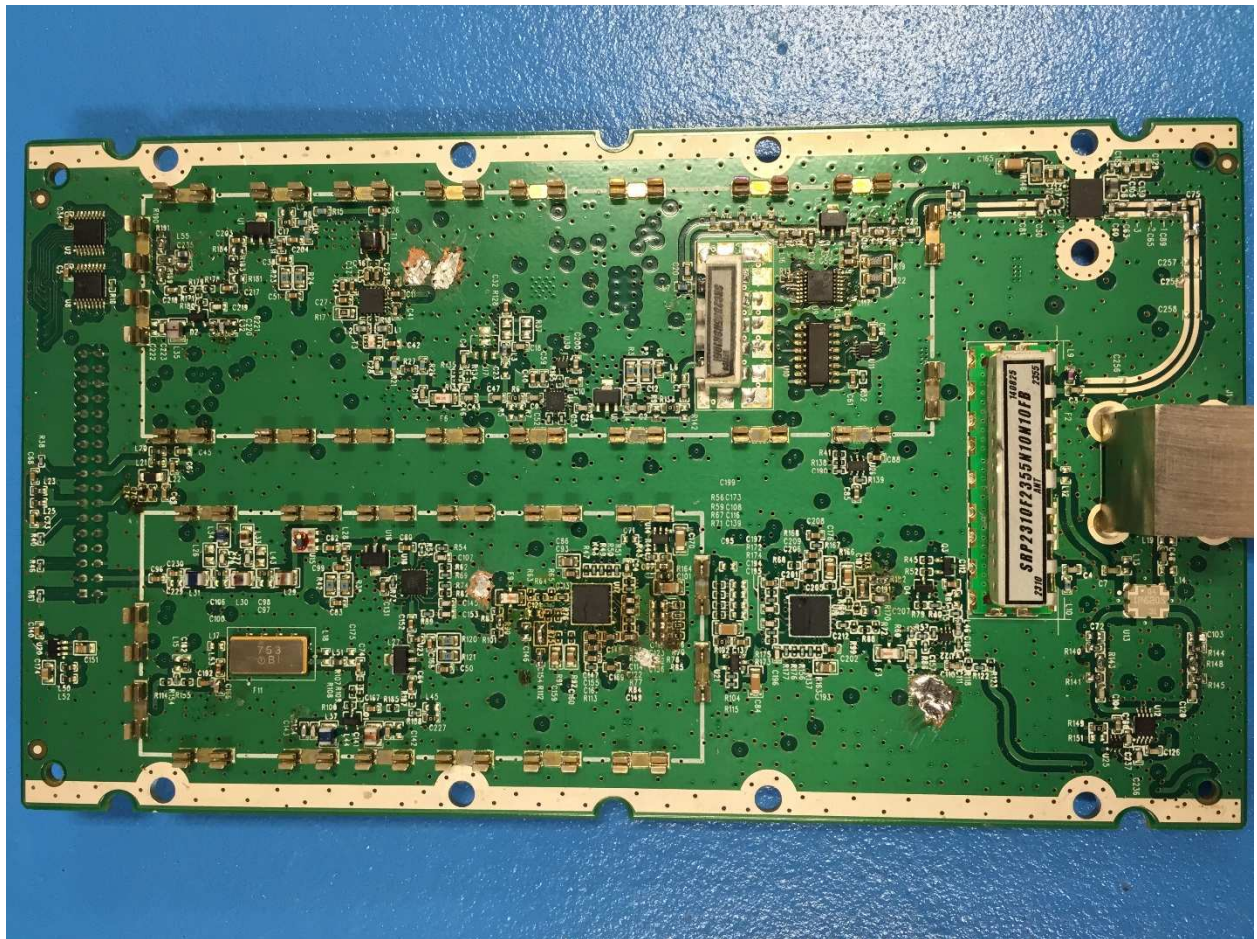
Path 2 RF Board Top View
