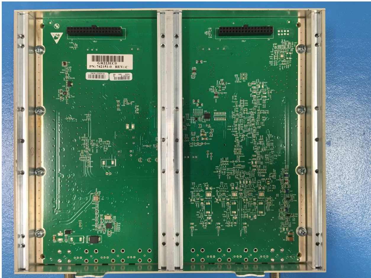
IF Board Top View
