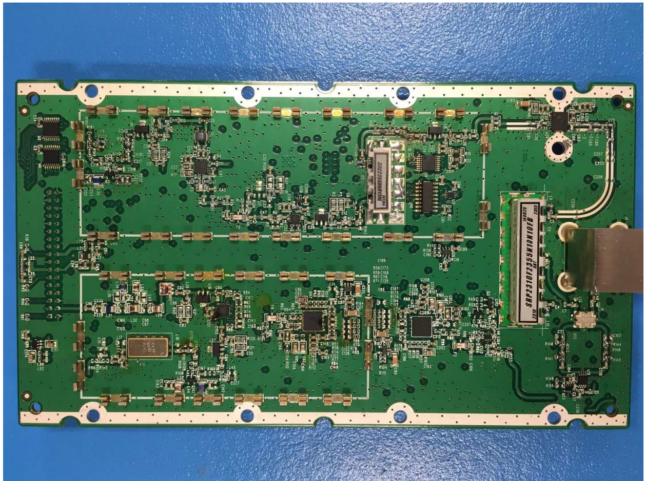
Path 1 RF Board Top View
