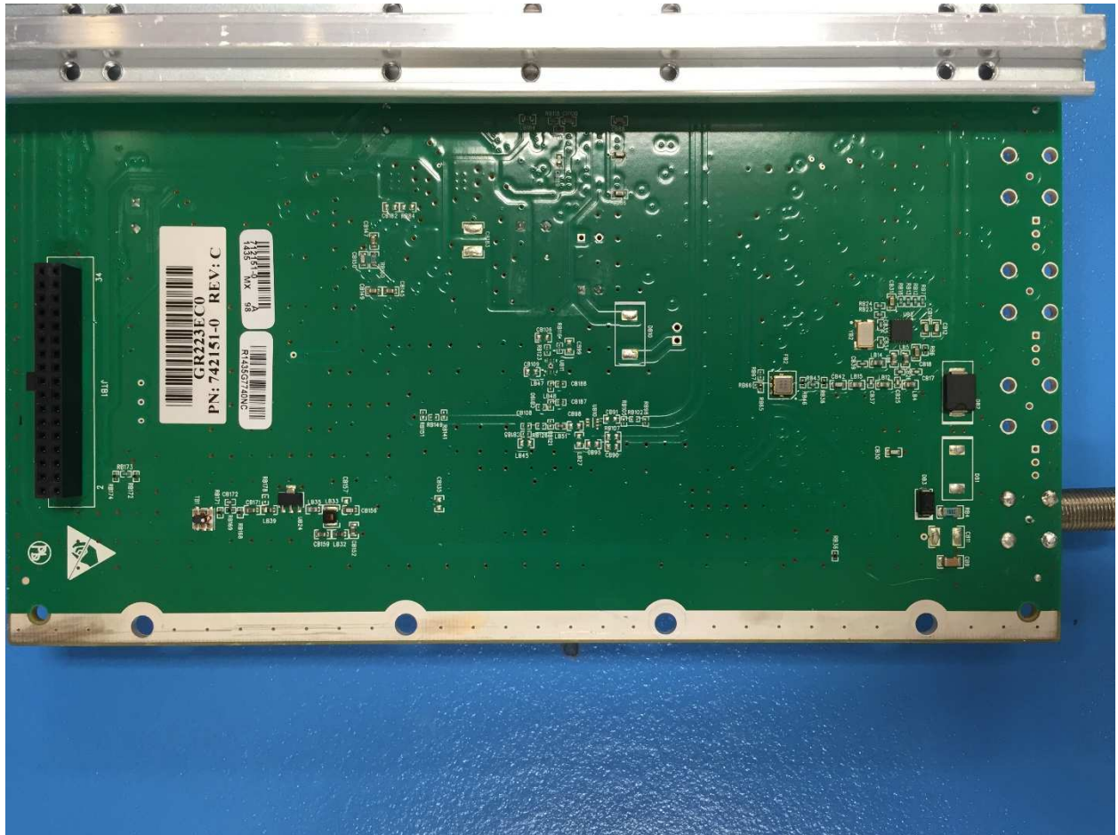
IF Board Top Left Side View
