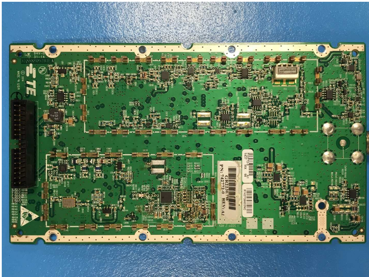
Path 2 RF Board Bottom View
