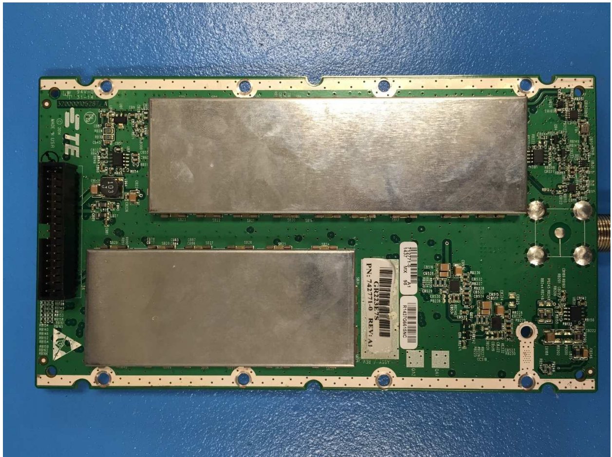
Path 1 RF Board Bottom View (Shielded)
