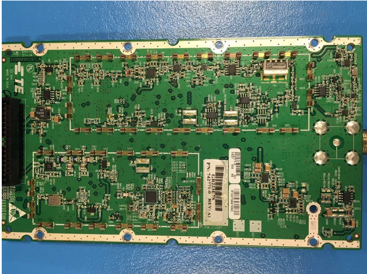
Path 1 RF Board Bottom View
