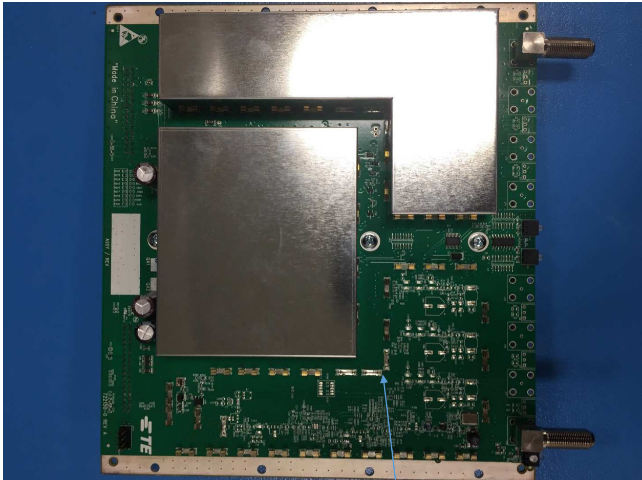
IF Board Bottom Right Side View (Shielded – one shield missing)
