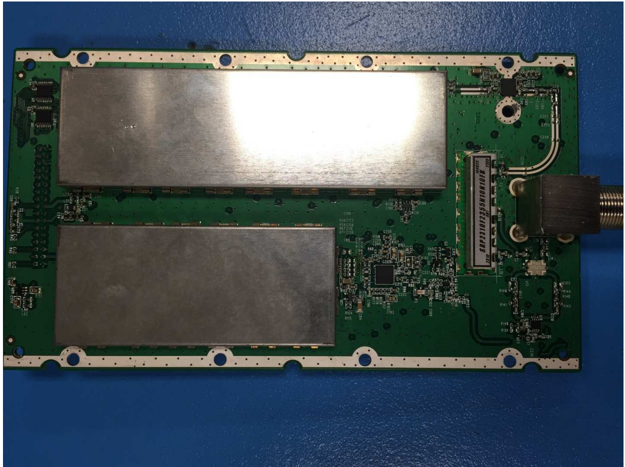
Path 1 RF Board Top View (Shielded)
