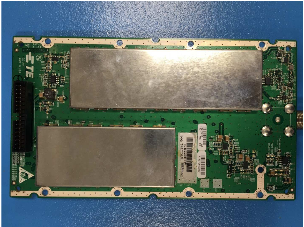
Path 2 RF Board Bottom View (Shielded)
