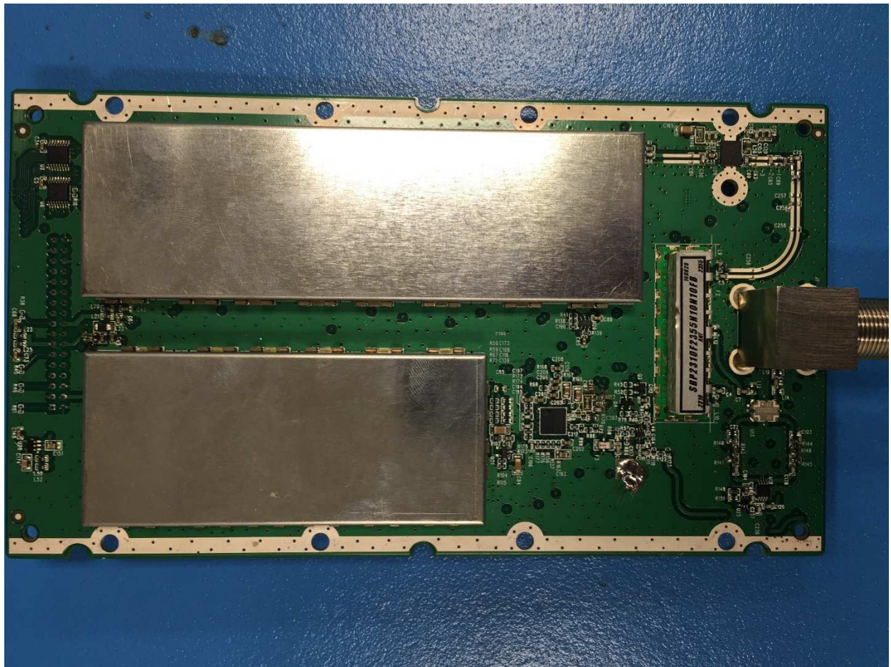
Path 2 RF Board Top View (Shielded)
