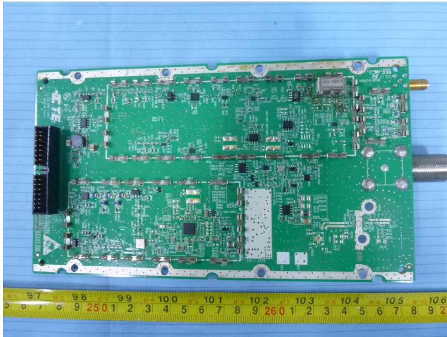
EUT – 1900 MHz Band Main Board Bottom Shielding off View
