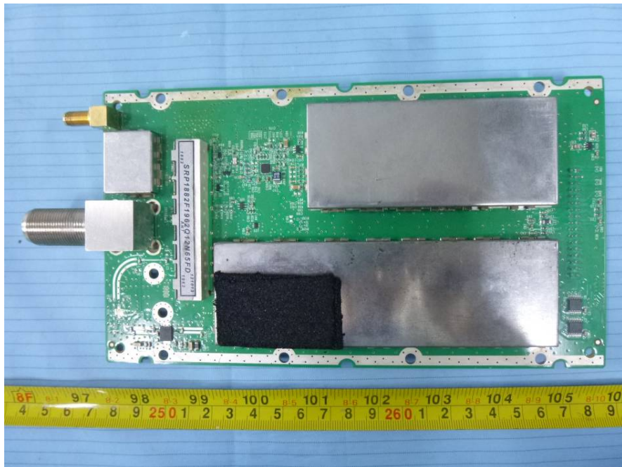
EUT – 1900 MHz Band Main Board Top View
