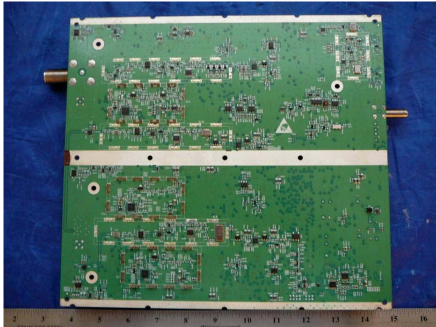
EUT PCB Assembly (Without Shielding) Bottom View – RUA
