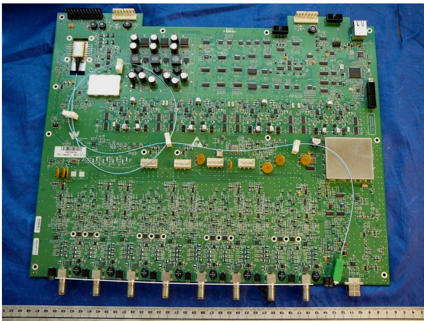
EUT PCB Assembly (With Shielding) Top View – EHUB
