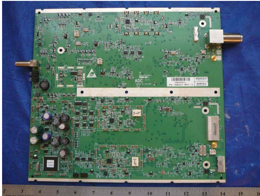
EUT PCB Assembly (Without Shielding) Top View - RUA
