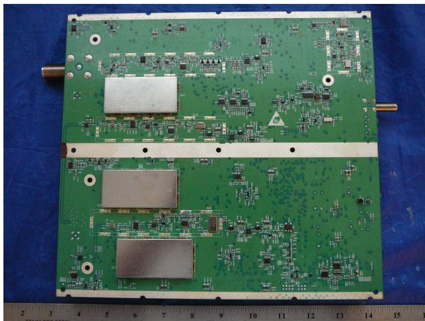
EUT PCB Assembly (With Shielding) Bottom View – RUA
