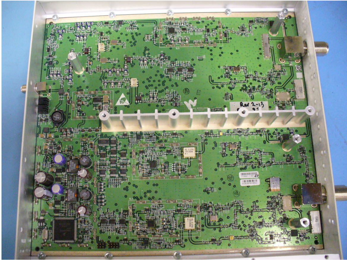
InterReach® Fusion Remote Access Unit Top View – Covers Removed
