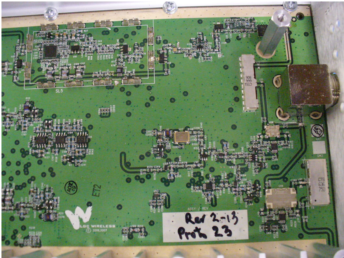
InterReach® Fusion Remote Access Unit Top View - 4
