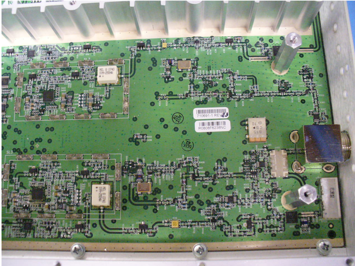
InterReach® Fusion Remote Access Unit Top View - 1
