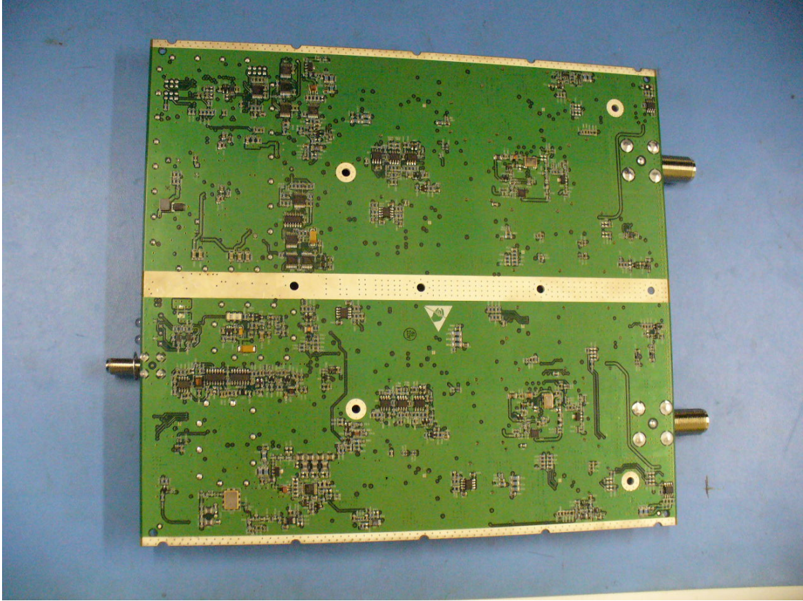
InterReach® Fusion Remote Access Unit Bottom View
