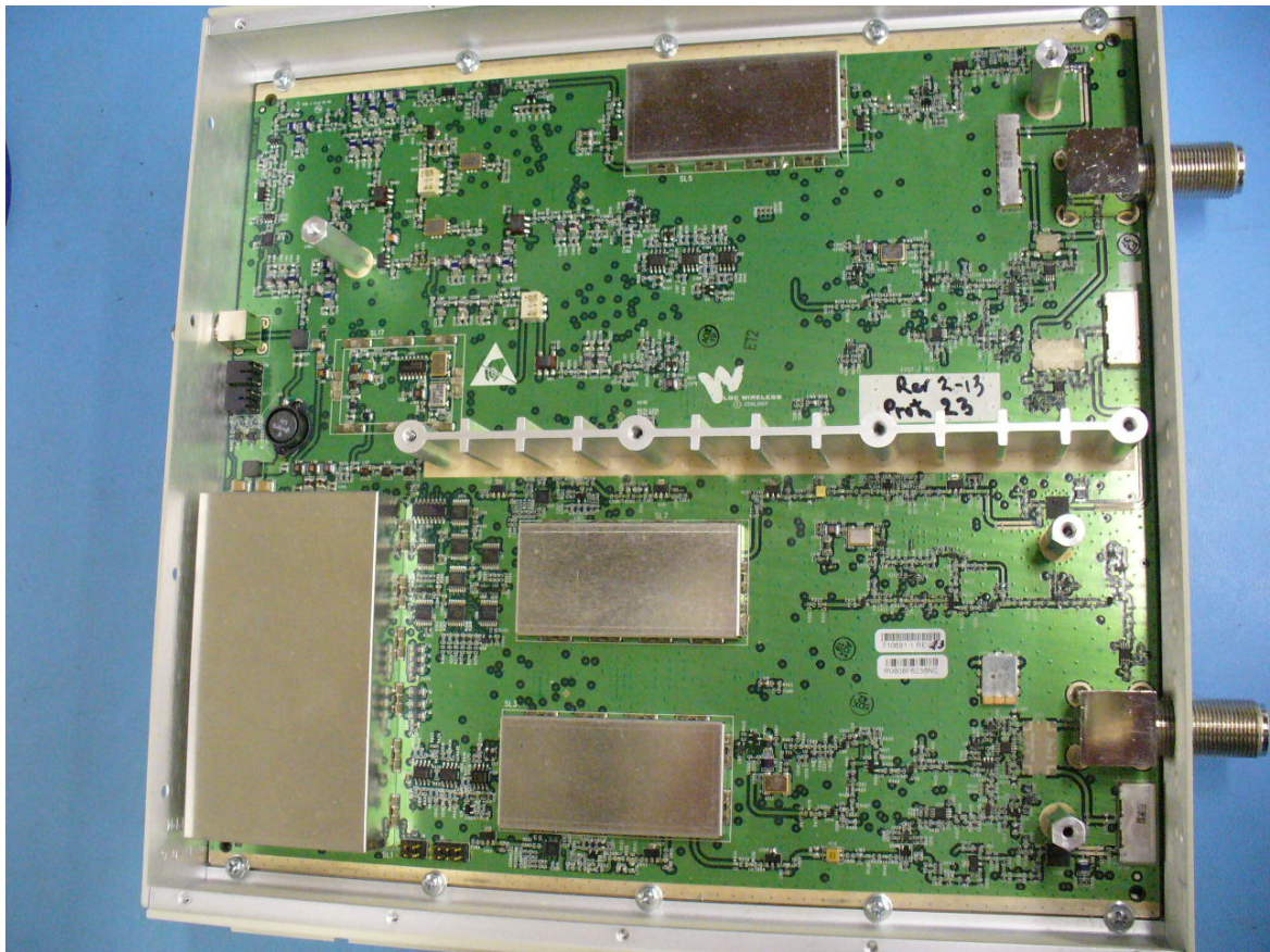
InterReach® Fusion Remote Access Unit Top View
