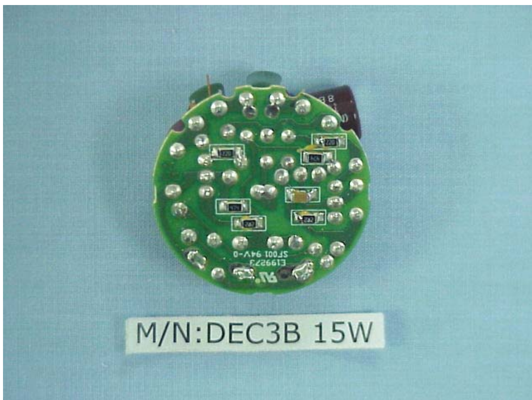
FIGURE 6 ELECTRONIC ENERGY SAVING LAMP (M/N: DEC3B 15W) MAIN BOARD (SOLDERED SIDE)
