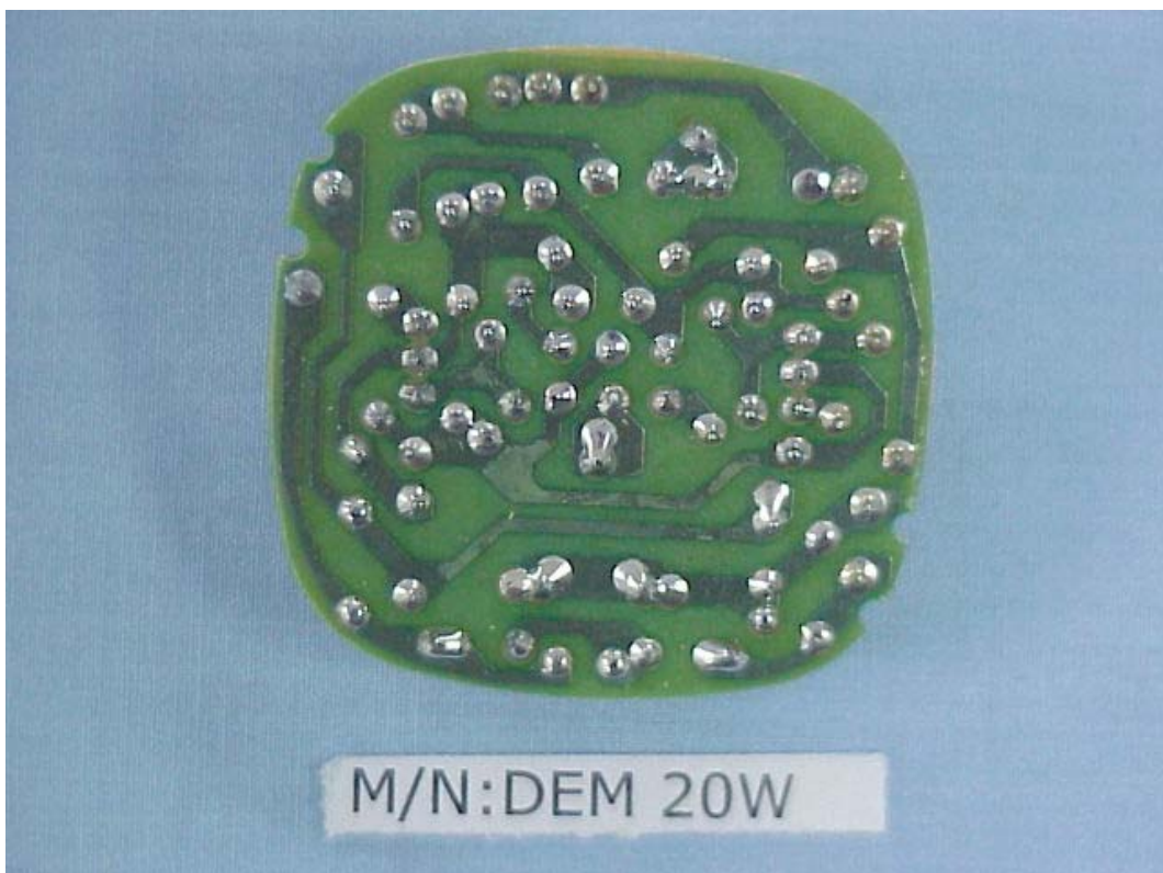
FIGURE 12 ELECTRONIC ENERGY SAVING LAMP (M/N: DEM 20W) MAIN BOARD (SOLDERED SIDE)
