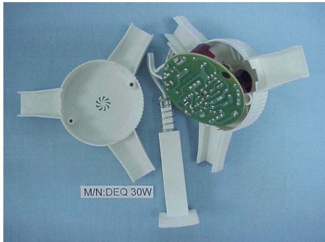
Figure 19 ELECTRONIC ENERGY SAVING LAMP (M/N: DEQ 30W) COVER REMOVED
