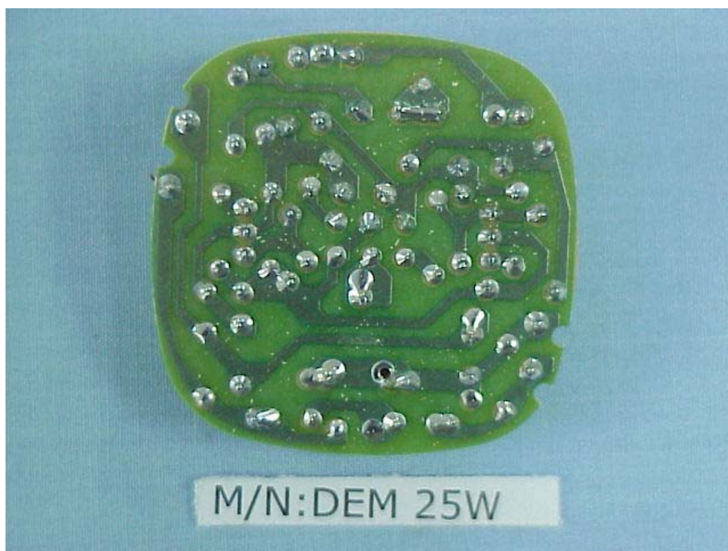
FIGURE 15 ELECTRONIC ENERGY SAVING LAMP (M/N: DEM 25W) MAIN BOARD (SOLDERED SIDE)
