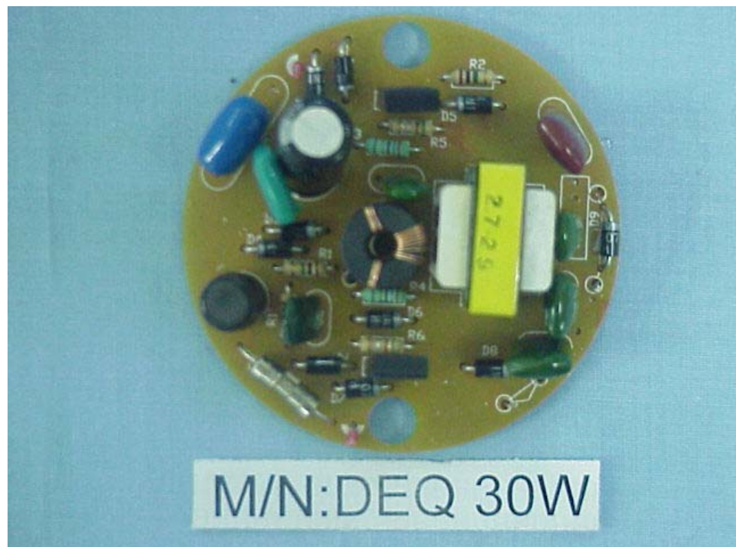
FIGURE 20 ELECTRONIC ENERGY SAVING LAMP (M/N: DEQ 30W) MAIN BOARD (COMPONENT SIDE)
