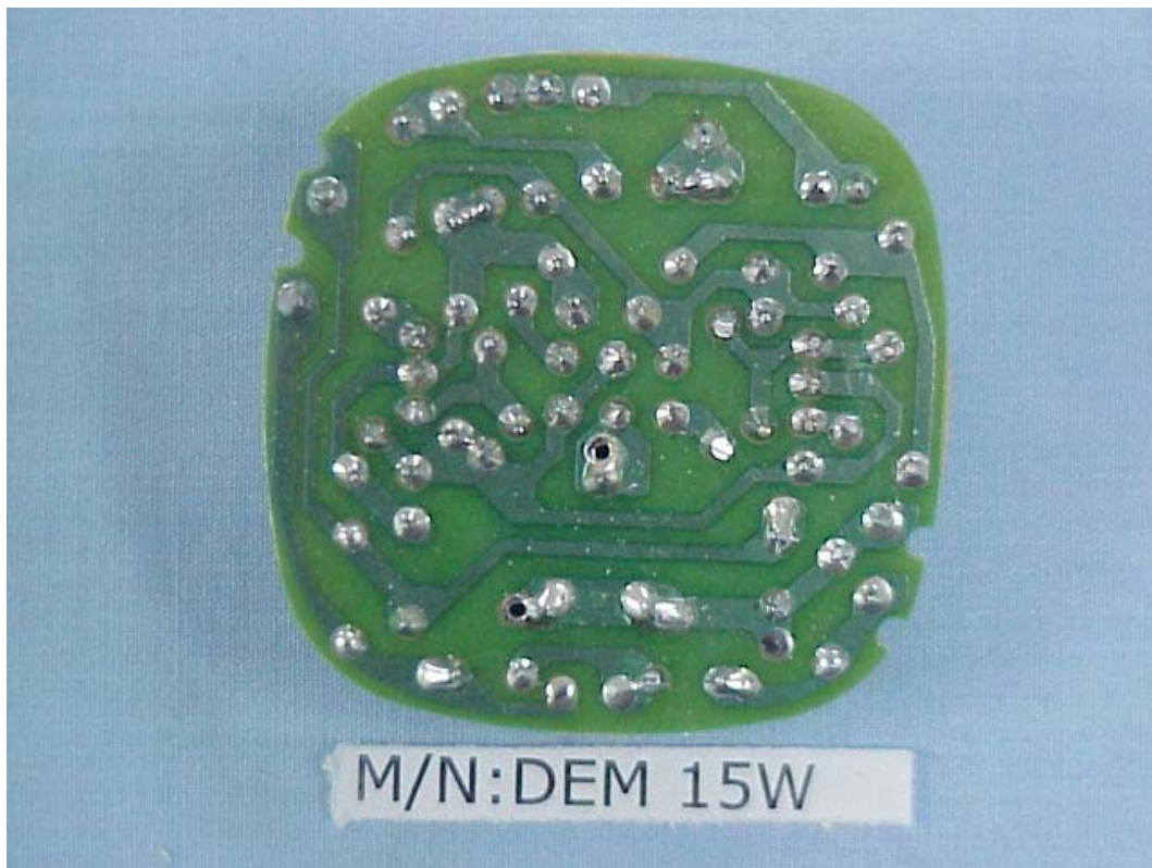
FIGURE 9 ELECTRONIC ENERGY SAVING LAMP (M/N: DEM 15W) MAIN BOARD (SOLDERED SIDE)
