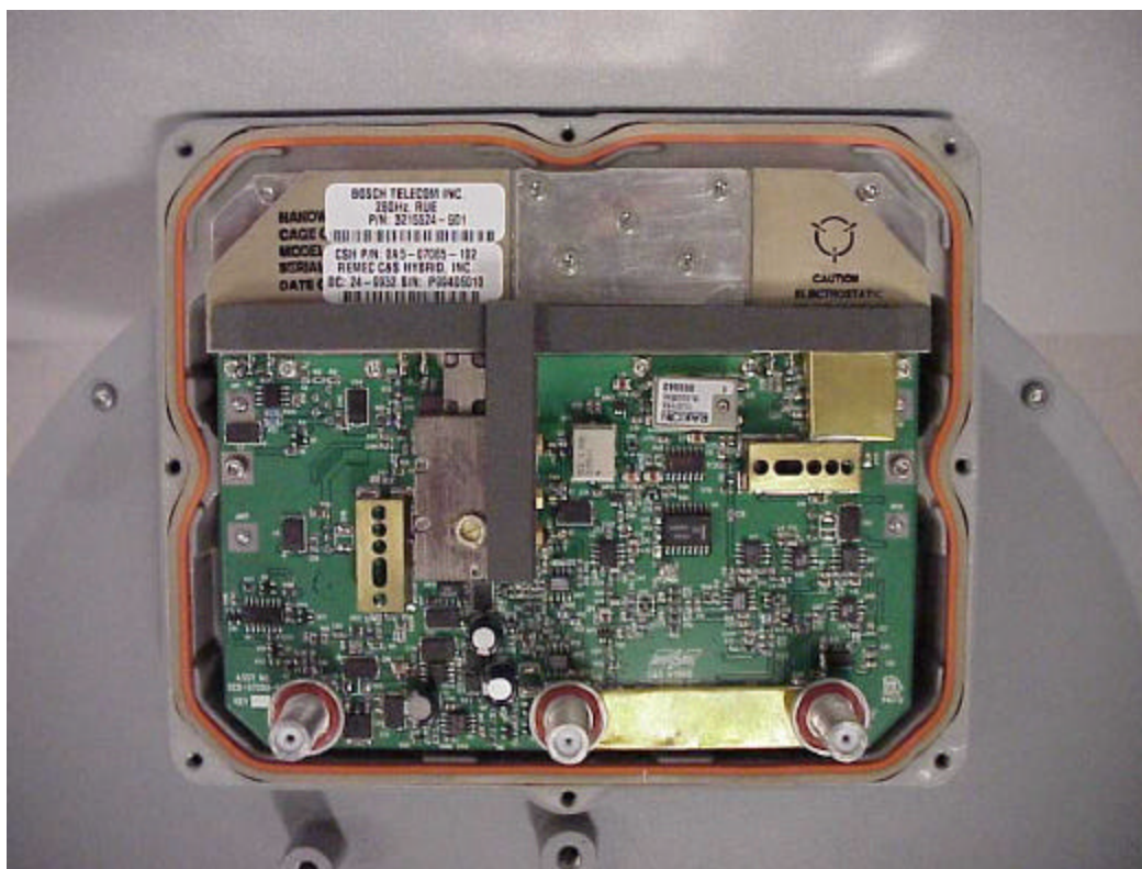
Figure 9-3 CPE Roof Unit with Electronics Board - Cover Removed (Close up view)
