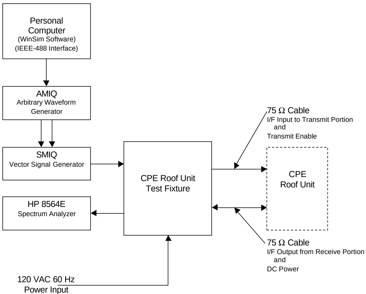
Figure 4-1 CPE Roof Unit Test and Support Equipment
