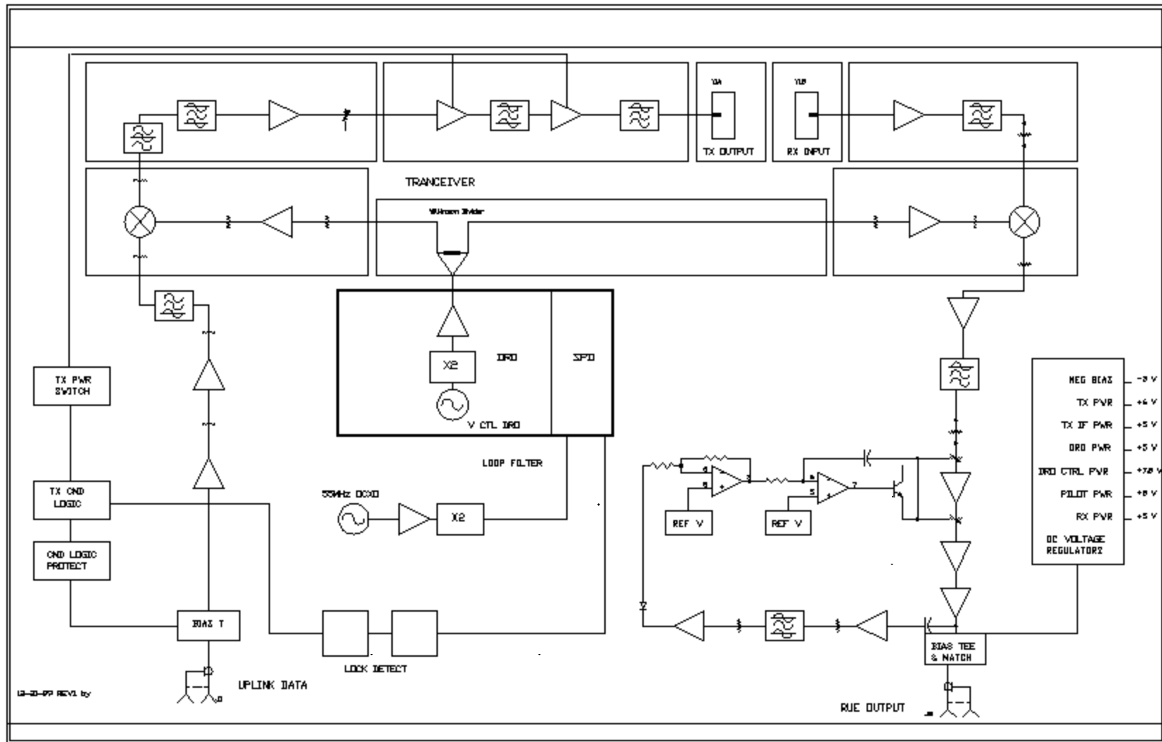
Figure 4-1 CPE ROOF UNIT BLOCK DIAGRAM
