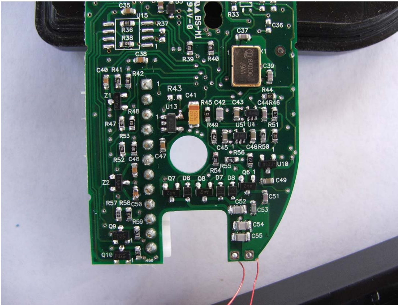
SECURA KEY INTERNAL REAR VIEW BOTTOM FCC ID: NNHDTR1 RKDT-SA-S
