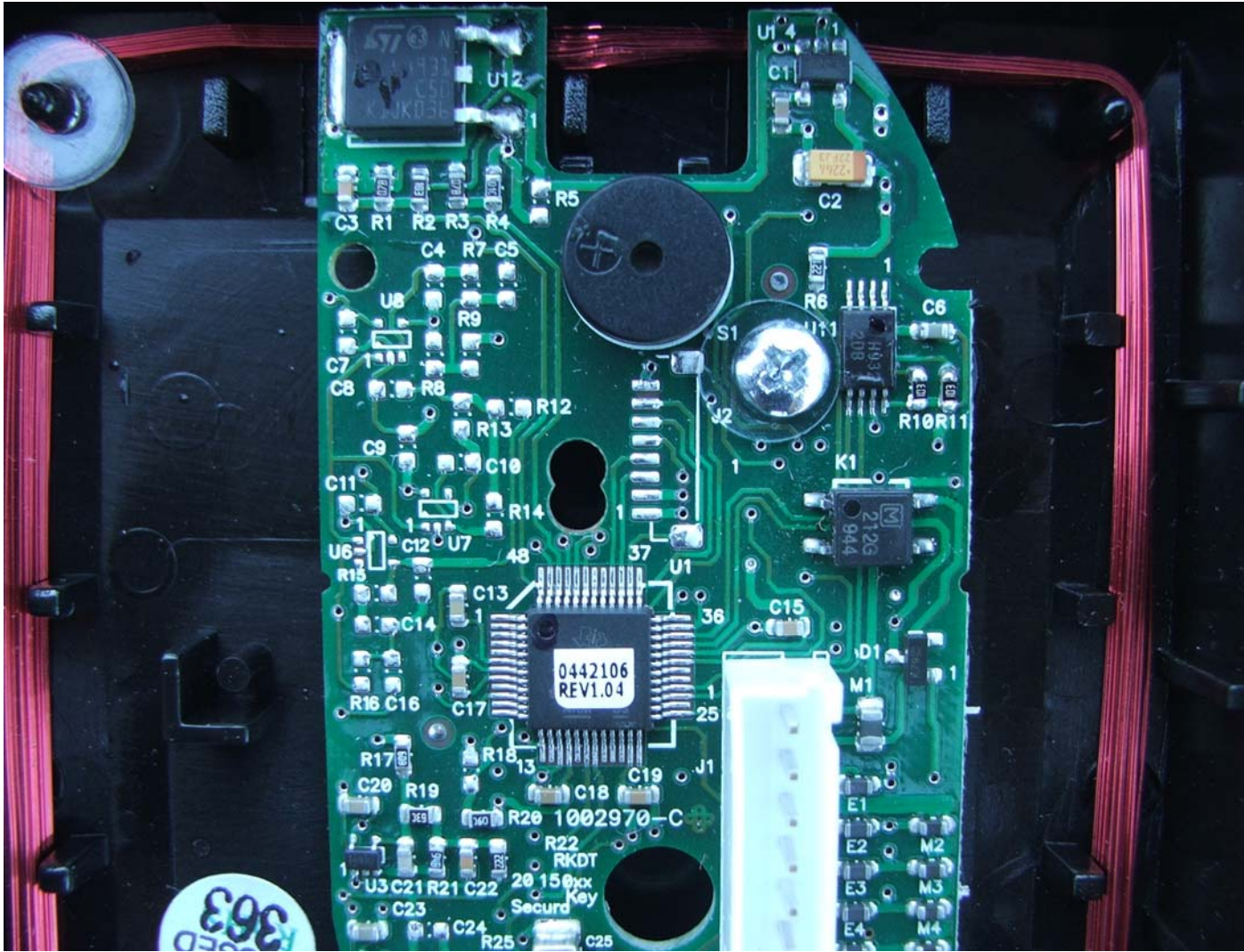
SECURA KEY INTERNAL FRONT VIEW TOP FCC ID: NNHDTR1 RKDT-SA-S
