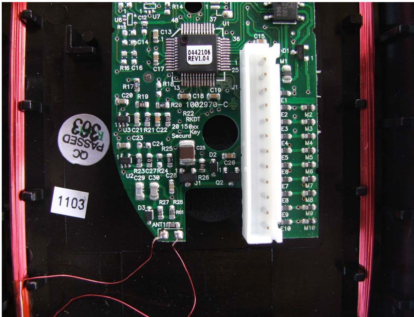
SECURA KEY INTERNAL FRONT VIEW BOTTOM FCC ID: NNHDTR1 RKDT-SA-S
