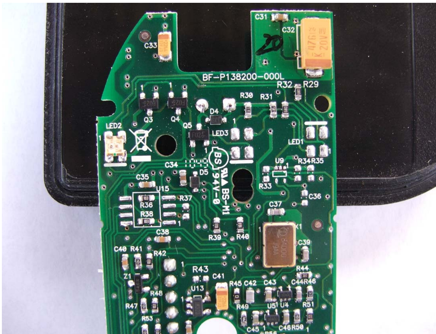
SECURA KEY INTERNAL REAR VIEW TOP FCC ID: NNHDTR1 RKDT-SA-S
