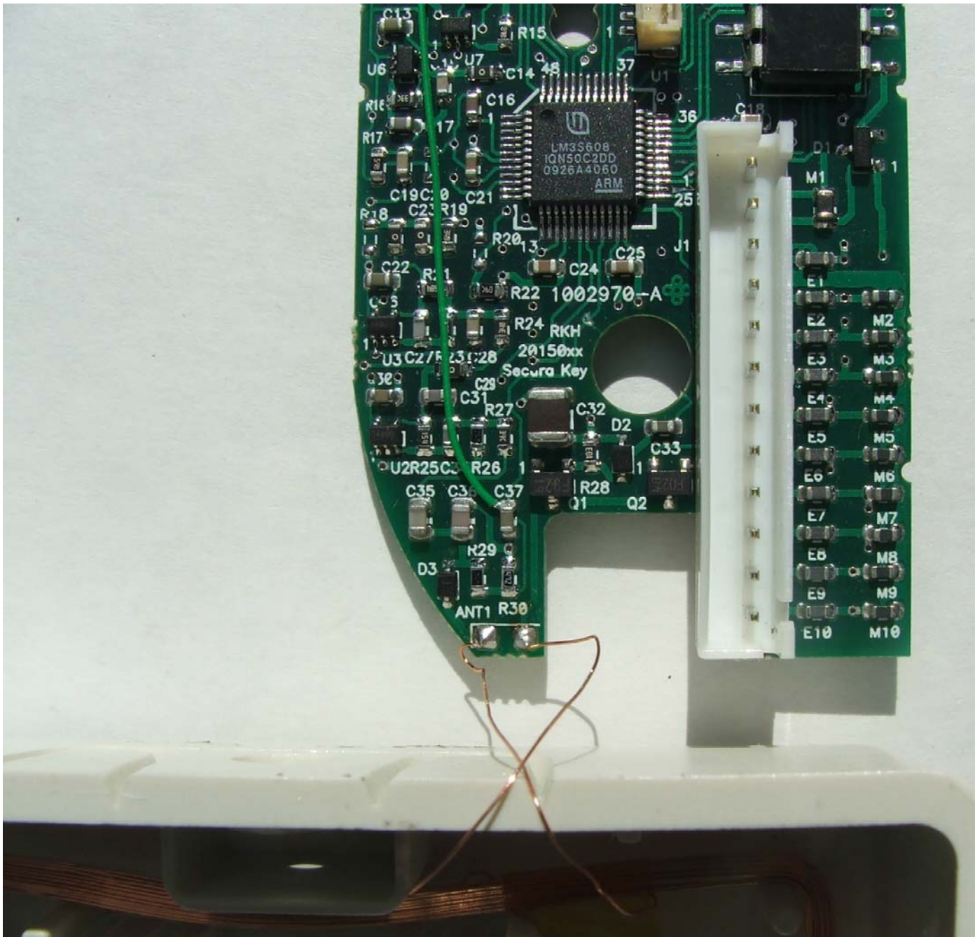
SECURA KEY INTERNAL FRONT VIEW BOTTOM FCC ID: NNHDTR1
