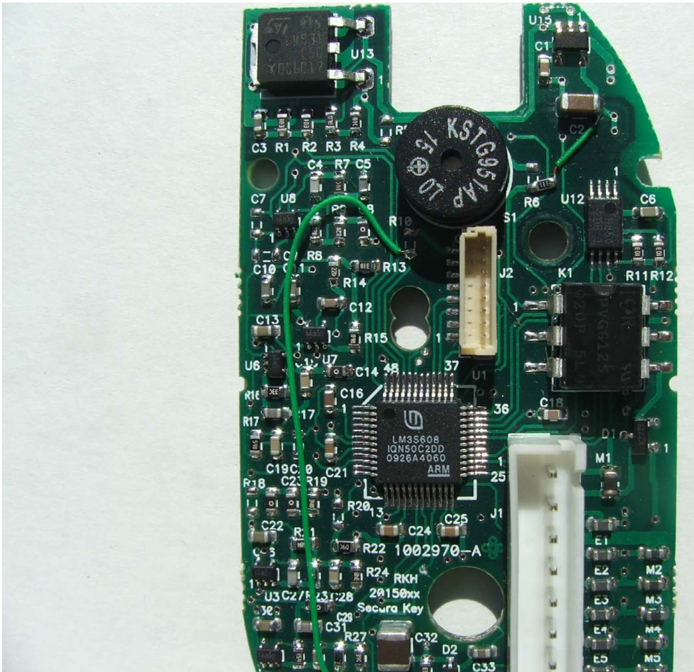
SECURA KEY INTERNAL FRONT VIEW TOP FCC ID: NNHDTR1
