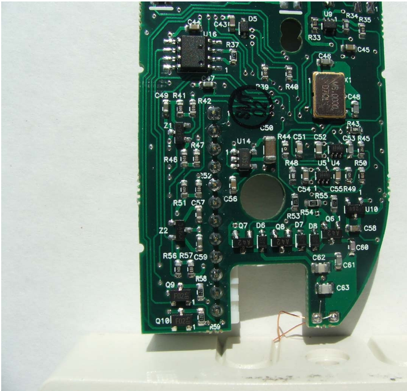
SECURA KEY INTERNAL REAR VIEW BOTTOM FCC ID: NNHDTR1
