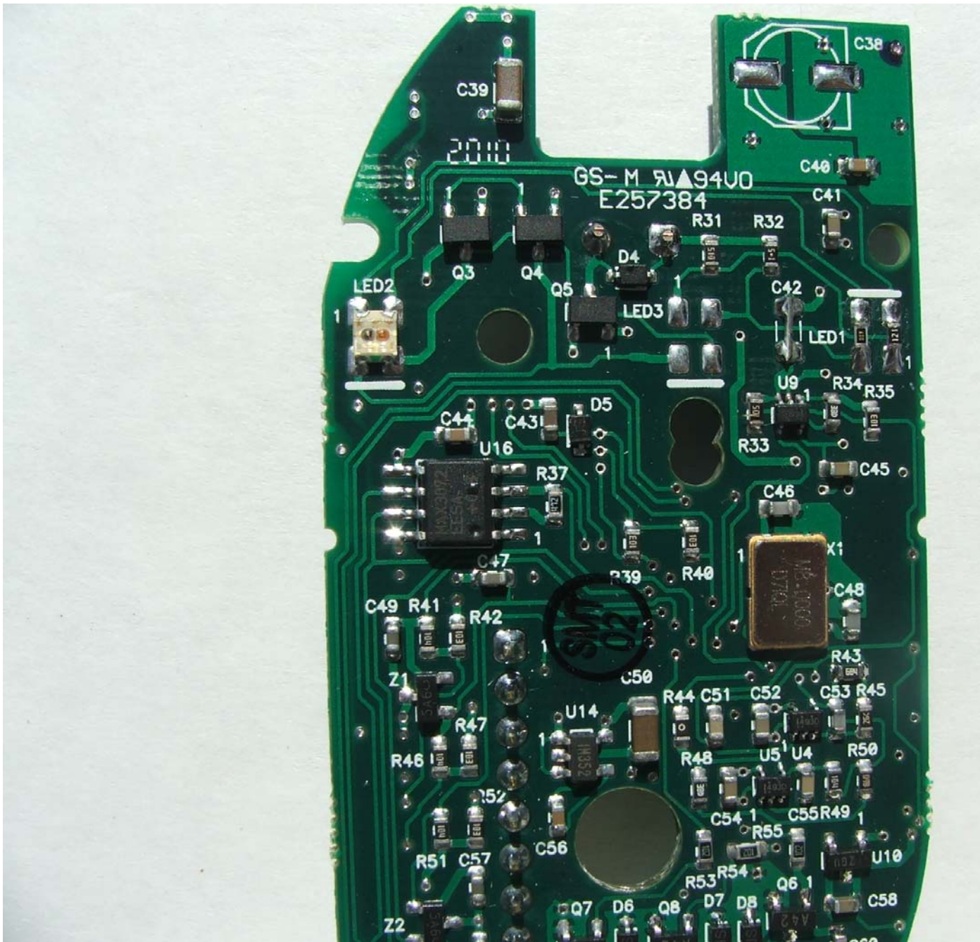
SECURA KEY INTERNAL REAR VIEW TOP FCC ID: NNHDTR1
