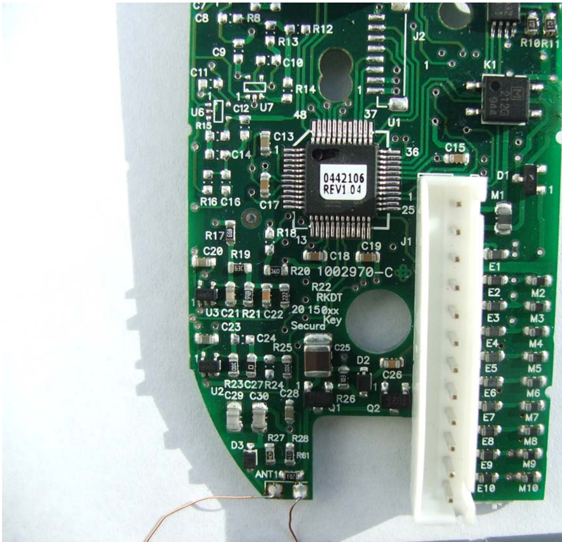
SECURA KEY INTERNAL FRONT VIEW BOTTOM FCC ID: NNHDTR1 PPLX
