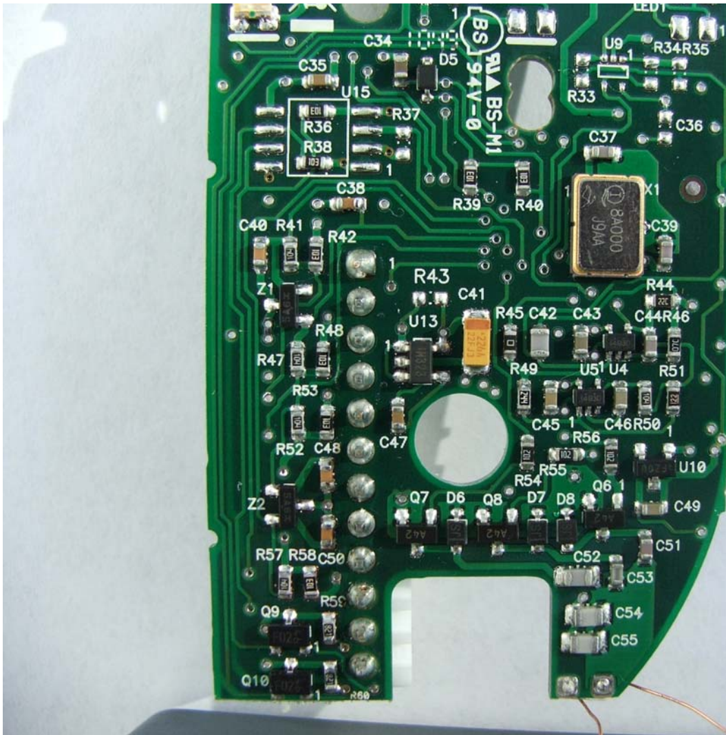
SECURA KEY INTERNAL REAR VIEW BOTTOM FCC ID: NNHDTR1 PPLX
