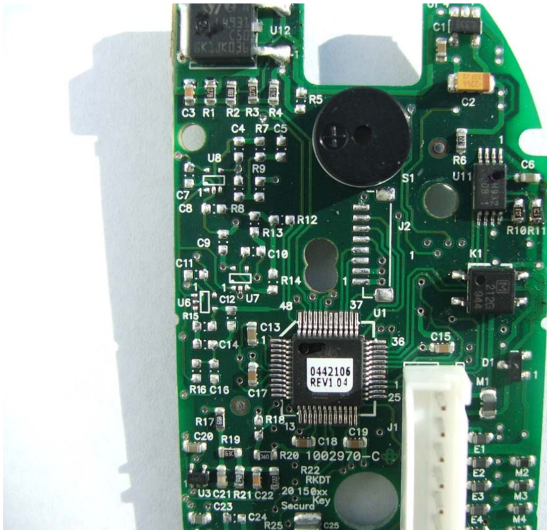
SECURA KEY INTERNAL FRONT VIEW TOP FCC ID: NNHDTR1 PPLX
