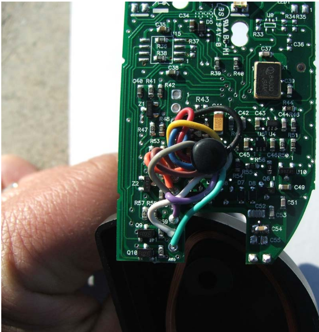
SECURA KEY INTERNAL REAR VIEW BOTTOM FCC ID: NNHDTR1 AM-DPR (RKDT-WM)
