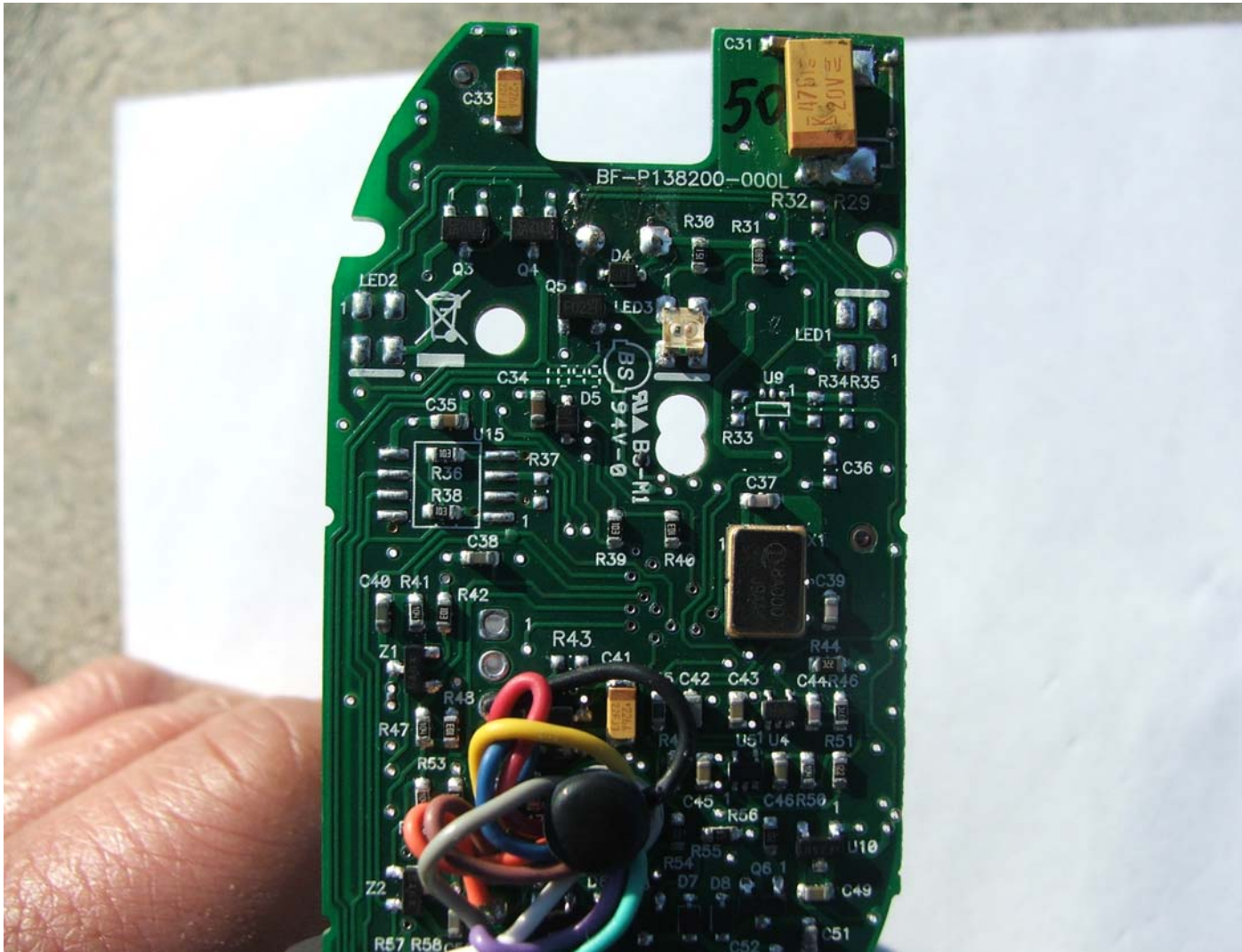
SECURA KEY INTERNAL REAR VIEW TOP FCC ID: NNHDTR1 AM-DPR (RKDT-WM)
