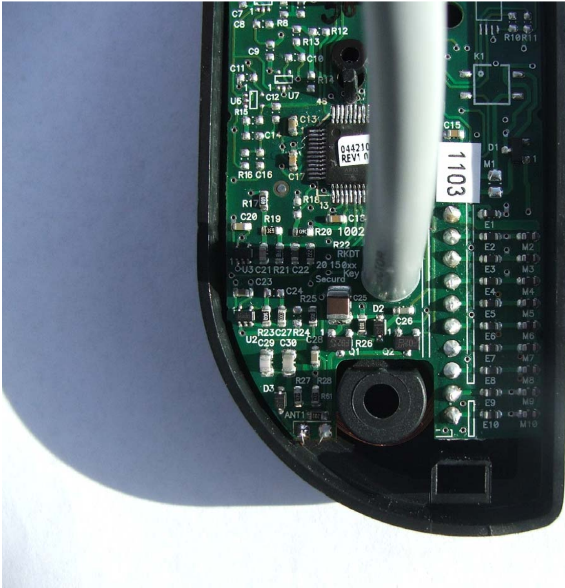
SECURA KEY INTERNAL FRONT VIEW BOTTOM FCC ID: NNHDTR1 AM-DPR (RKDT-WM)
