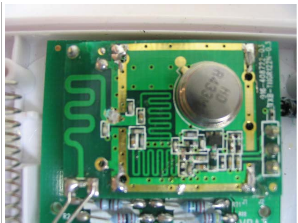
Transmitter
