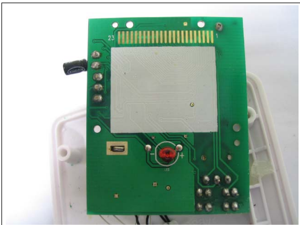
Transmitter
