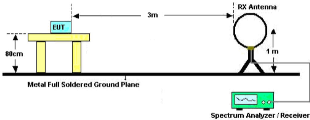
Radiated Emission Test-Setup Frequency Below 30MHz
