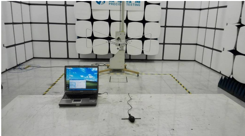
FCC RADIATED EMISSION TEST SETUP
