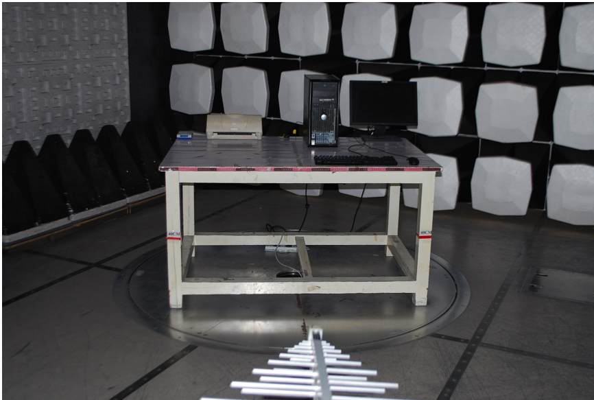
Radiated Emission
