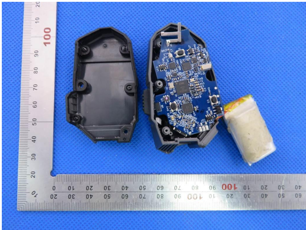
Series Model MOTION 6 OPEN VIEW OF EUT
