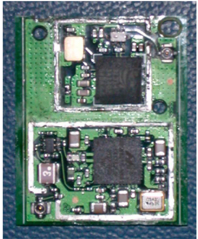
Shields removed
