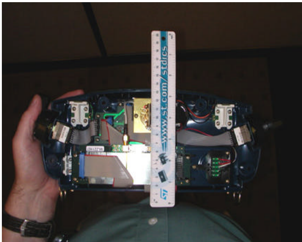
Top view showing measured distance of Antenna to Human Body Measured distance is constant at approximately ... 3.5 inches or 8.89 cm's
