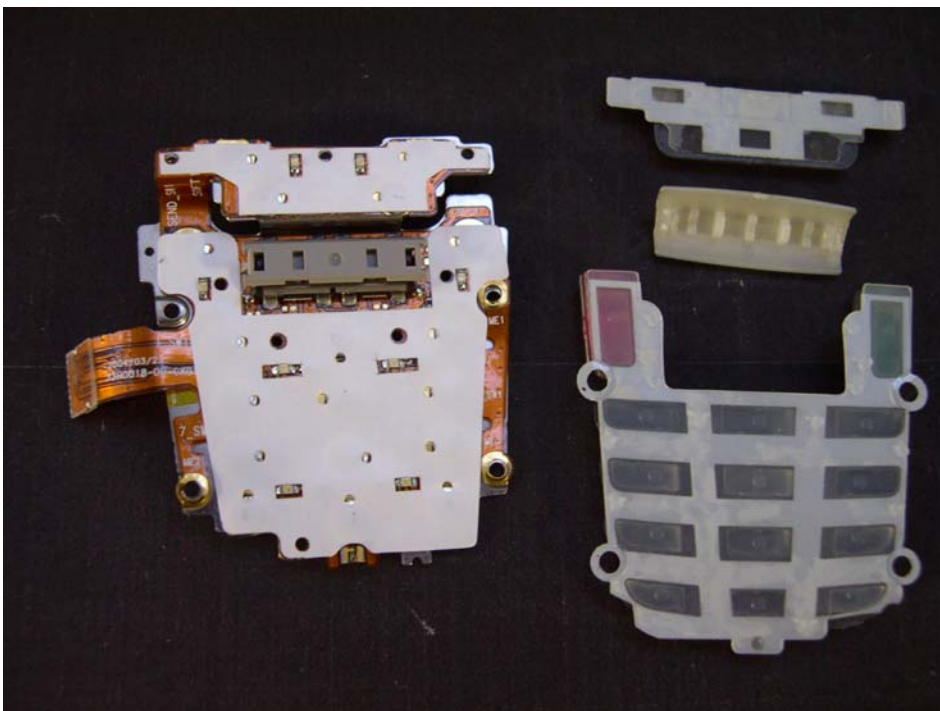
Keypad View II
