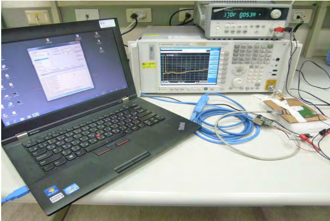
Conducted Setup Photo – 2 (Measurement at Antenna Port)
