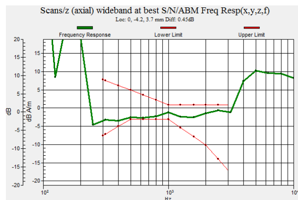
Fig. 9.12 CDMA2000 BC15 Ch875 (Sample 2)
