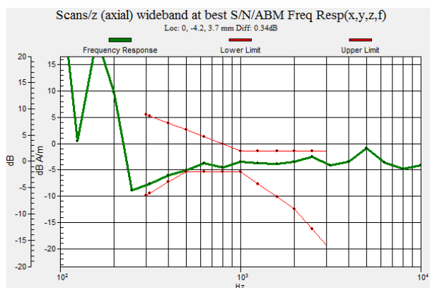
Fig. 9.11 CDMA2000 BC15 Ch875 (Sample 1)
