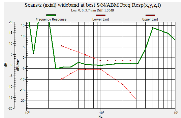
Fig. 9.8 CDMA2000 BC1 Ch600 (Sample 2)
