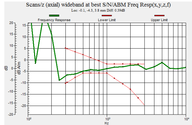
Fig. 9.6 CDMA2000 BC1 Ch600 (Sample 1)
