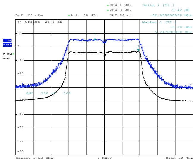
Peak Excursion Ratio Plot on 802.11n HT40 Channel 46
