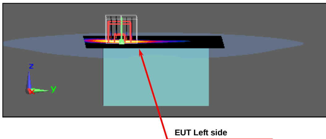
Figure 7. Body SAR Test Setup (Flat Section)
