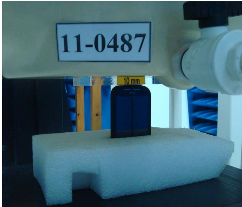
Figure 10. Body SAR Test Setup (Flat Section)
