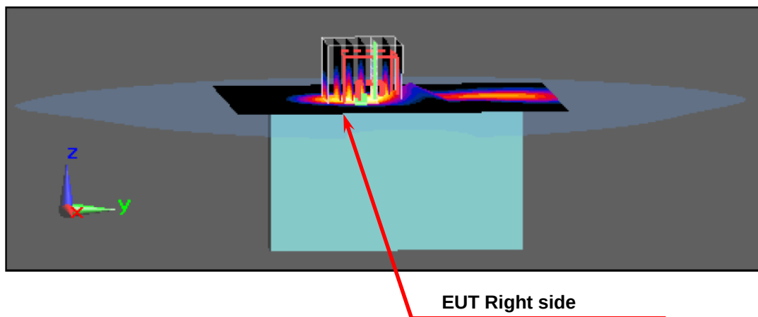
Figure 8. Body SAR Test Setup (Flat Section)
