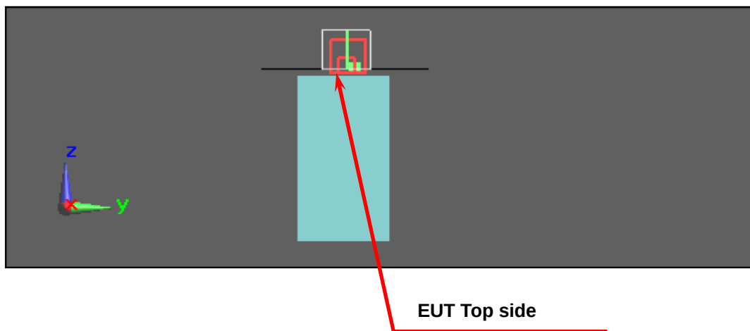
Figure 10. Body SAR Test Setup (Flat Section)
