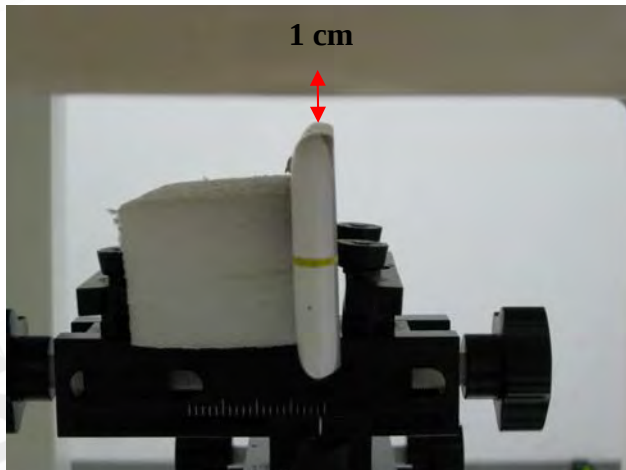
Fig.12 Hotspot mode- EUT Left to flat phantom and distance between flat phantom and mobile phone is 1 cm.
