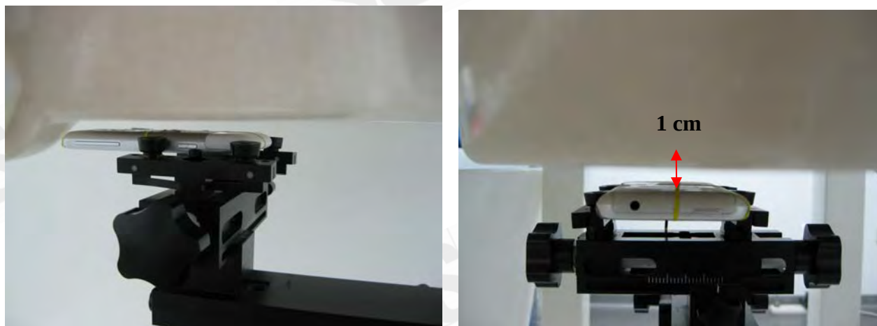
Fig.8 Hotspot mode- EUT back to flat phantom and distance between flat phantom and mobile phone is 1 cm.
