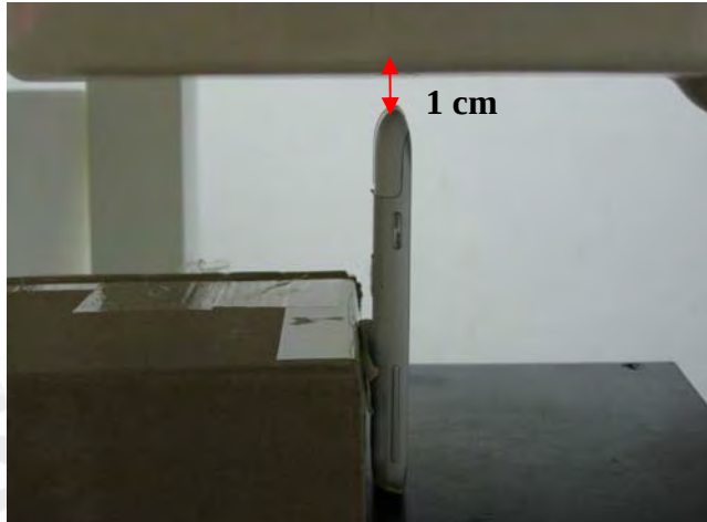
Fig.10 Hotspot mode- EUT Bottom to flat phantom and distance between flat phantom and mobile phone is 1 cm.
