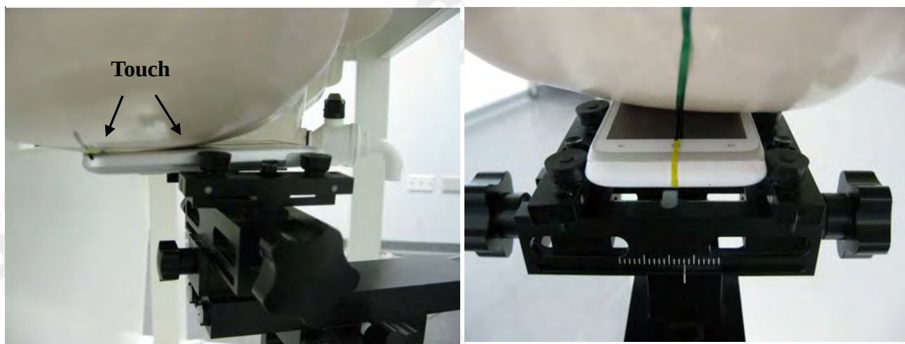
Fig.3 Right Head Section / Cheek-Touch Position
