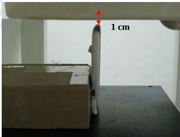
Fig.9 Hotspot mode- EUT Top to flat phantom and distance between flat phantom and mobile phone is 1 cm.
