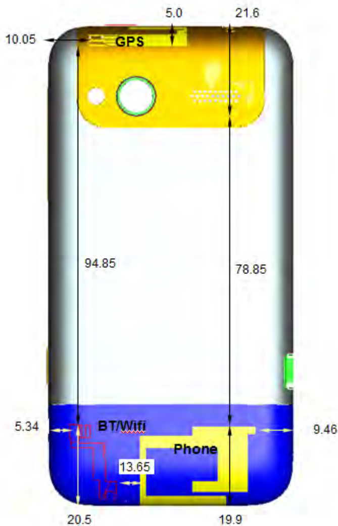
Fig.18 Antenna position of EUT
