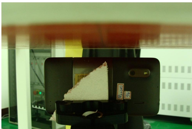
Right Side of the DUT with Phantom 1 cm Gap for DUT without Earphone
