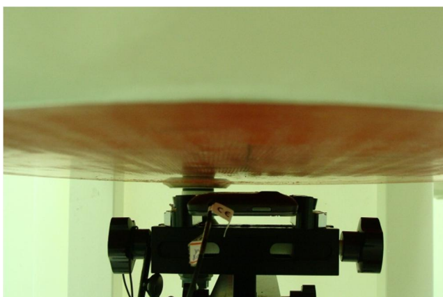
Rear Face of the DUT with Phantom 1 cm Gap for DUT with Earphone
