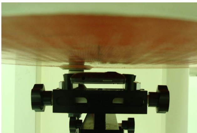
Rear Face of the DUT with Phantom 1 cm Gap for DUT without Earphone
