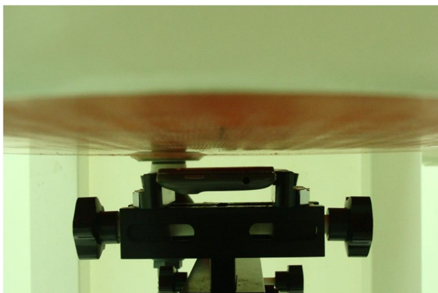
Front Face of the DUT with Phantom 1 cm Gap for DUT without Earphone
