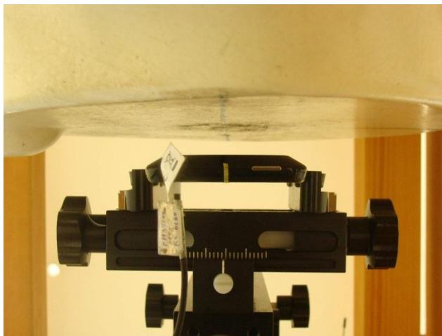
Back of the DUT with Phantom 1 cm Gap for DUT with Earphone 3
