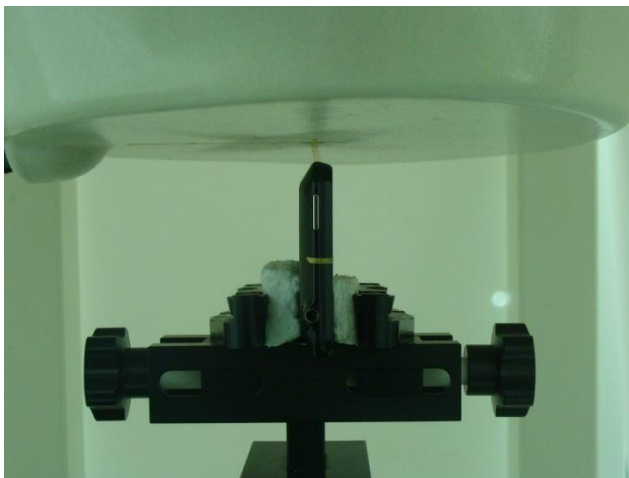
Right Side of the DUT with Phantom 1 cm Gap for DUT without Earphone
