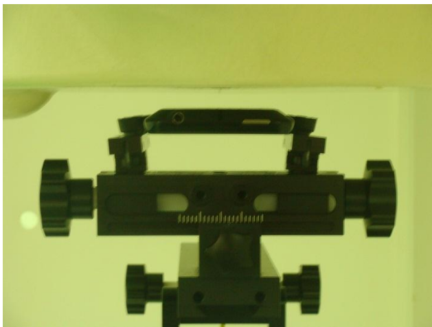
Back of the DUT with Phantom 1 cm Gap for DUT without Earphone
