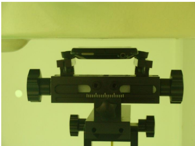
Front of the DUT with Phantom 1 cm Gap for DUT without Earphone
