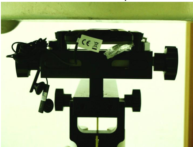
Rear Face of the DUT with Phantom 1.0 cm Gap for DUT with Earphone
